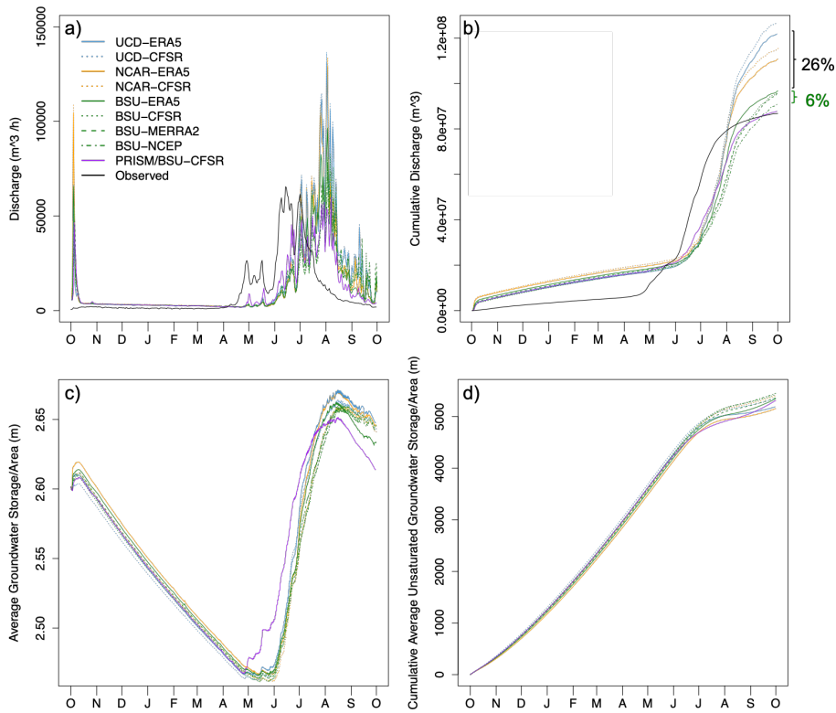
00 Figure 7. Time-series of ParFlow-CLM simulations of discharge rate (a), cumulative discharge (b), groundwater storage per unit area of the watershed (c), and cumulative average unsaturated groundwater storage per area of the watershed (d) for the IPM configurations described in Table 2. The brackets on the far-right indicate the percent difference of cumulative discharge and unsaturated groundwater storage per area (b and d, respectively) for WRF simulations across different meteorological forcings (green) and subgrid-scale physics schemes (black).
