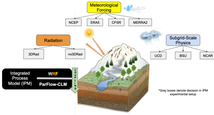
80 Figure 2. Conceptual framework for developing a set of different WRF configurations of the IPM to evaluate the sensitivities of subgrid-scale physics parameterization choice, meteorological forcing, and radiation scheme in the representation of mountain water and energy budgets.
