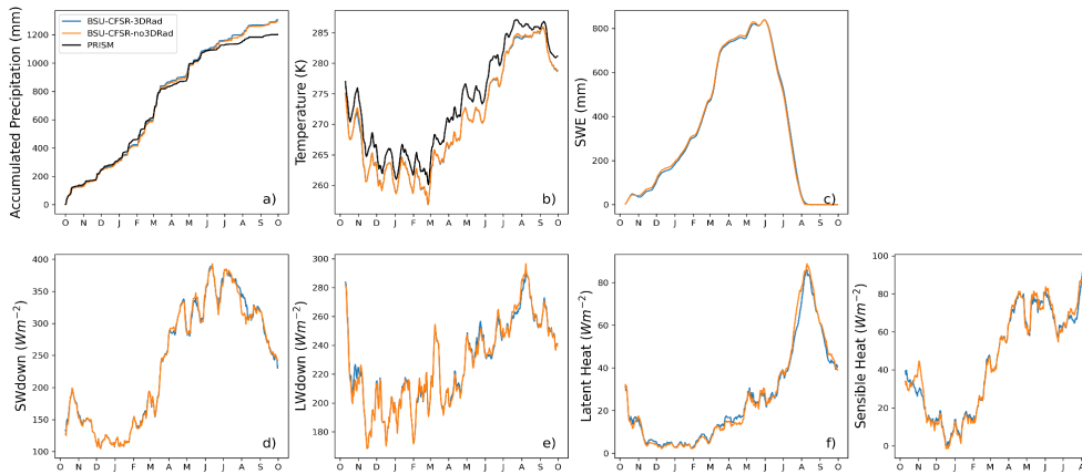
Figure 5. Spatial-average cumulative precipitation, two-meter surface air temperature and snow water equivalent (SWE) (first row), shortwave and longwave radiation, and latent and sensible heat (second row) over the ERW as simulated by the IPM configurations with and without realistic topographic radiation effects, along with, where available, estimates from PRISM. 3DRad indicates a simulation with topo_shading and slope_rad turned on in the WRF inner domain but not the outer WRF
