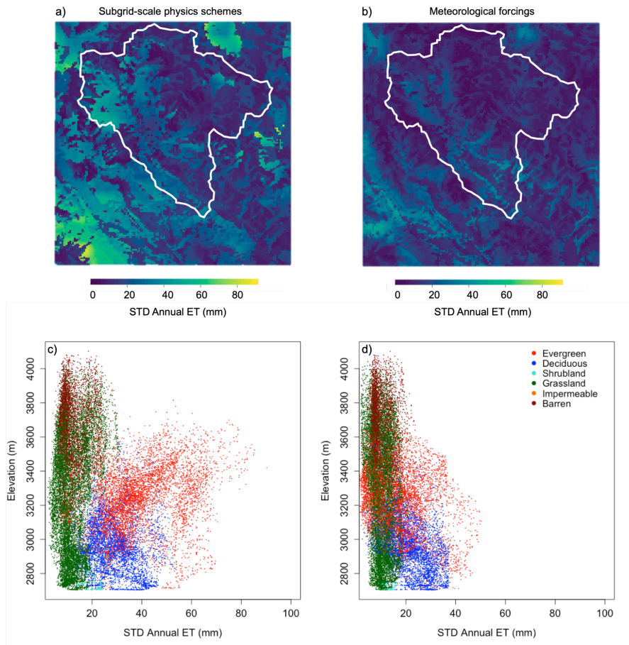
Figure 8. Pixel-level standard deviation in annual total evapotranspiration (ET) over the ParFlow-CLM domain from WRF with different subgrid-scale physics schemes (a,c) or meteorological forcing (b,d). The ERW outline is overlain in white in the
