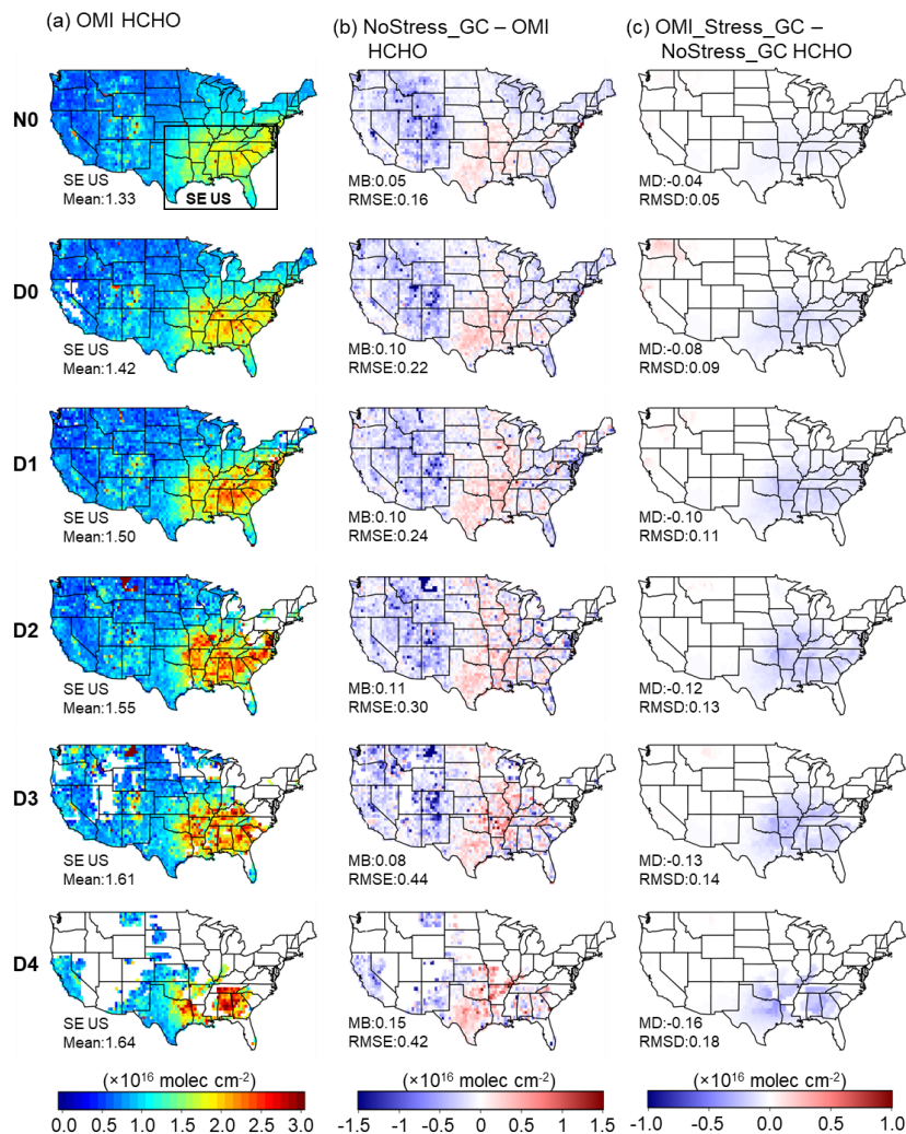
Figure 10. Mean HCHO column densities during JJA 2005-2017 by USDM dryness category for OMI (a), NoStress_GC minus OMI (b), and OMI_Stress_GC minus NoStress_GC (c). Numbers at the bottom-left corner of each panel indicate the SE US (black box) regional mean of OMI HCHO column (left column), mean bias (MB), and root mean square error (RMSE) in HCHO column densities between NoStress_GC and OMI (middle column), and mean differences (MD) and root mean square deviation (RMSD) between OMI_Stress_GC and NoStress_GC (right column). MD and RMSD are calculated in the same way as MB and RMSE; the different names are used to distinguish between model-to-model comparison and model-to-observation comparison, respectively.
