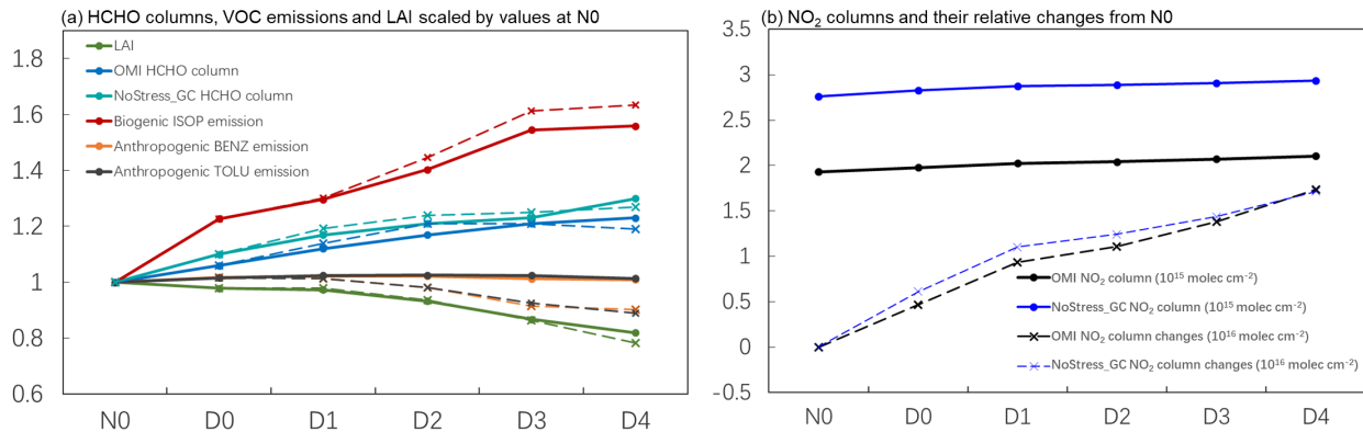
Figure 4. (a) Relative changes of regional-mean OMI HCHO column, GEOS Chem (NoStress_GC) simulated HCHO column, isoprene emissions, anthropogenic benzene emission, anthropogenic toluene emission, and MODIS leaf area index (LAI) under different drought levels in the southeast US. All data are scaled to their respective values at N0. The dotted lines are the arithmetic mean of all grids, and the solid lines are the corrected mean excluding the missing area. (b) Regional-mean tropospheric NO 2 columns from OMI and NoStress_GC (solid lines), and their respective changes from non-drought (N0) conditions (dashed lines). Note the different scales between the solid and dashed lines. The calculation is based on the grids with the presence of all USDM levels.
