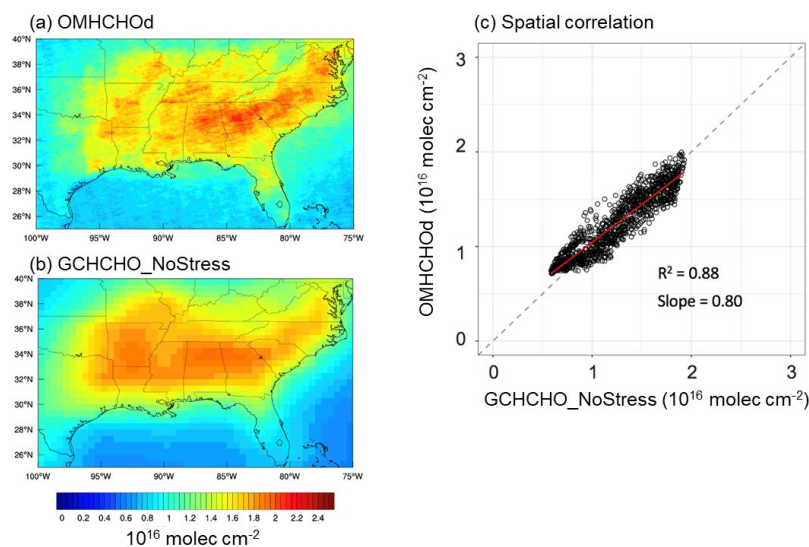
Figure 2. Mean 2005–2017 HCHO columns for June – August over the SE US of (a) OMI observation ( OMHCHOd ) and (b) GEOS-Chem simulation ( GCHCHO_NoStress ). (c) Scatterplot of spatial correlation between the two. The dashed line indicates the 1:1 agreement.
