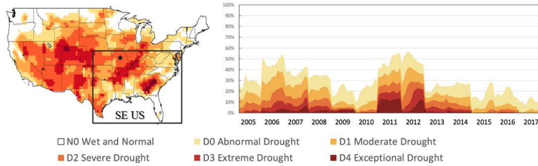
(a) USDM released on July 12,2012 (b) USDM time series for SE US
