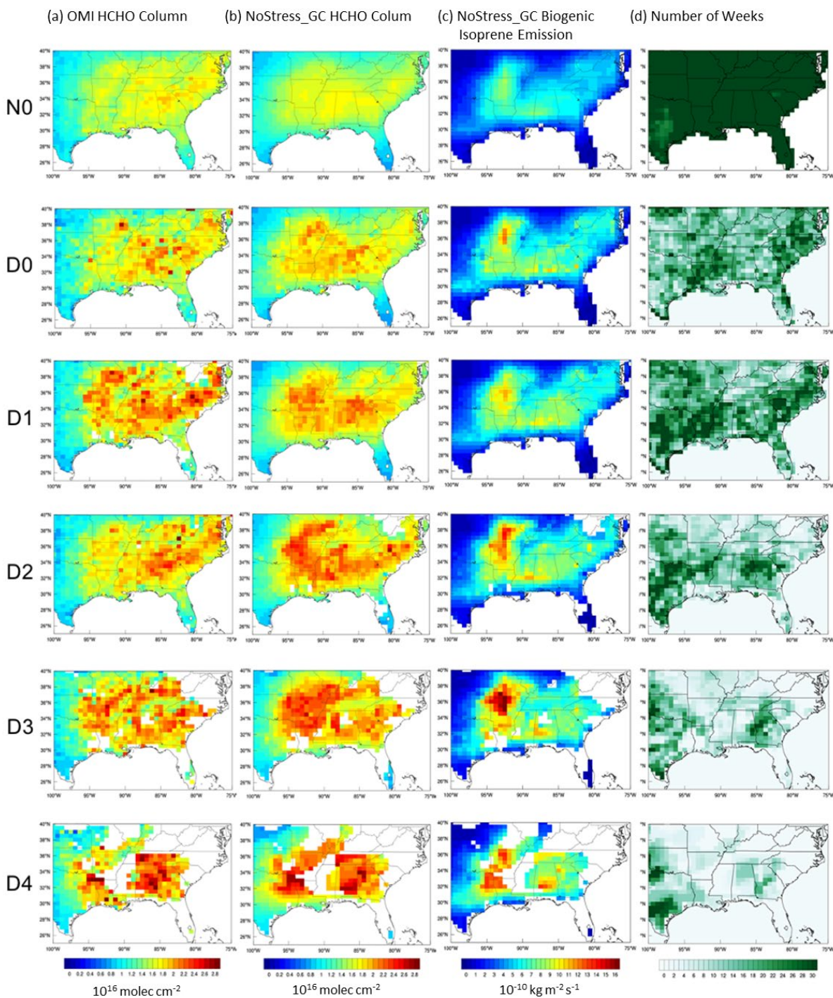
Figure 3. The mean spatial distributions of (a) OMI HCHO column density; (b) GEOS-Chem NoStress_GC HCHO column density, (c) NoStress_GC isoprene emissions, and (d) the number of weeks during JJA 2005 to 2017 in the southeast US under different USDN drought levels (N0, D0-D4).
