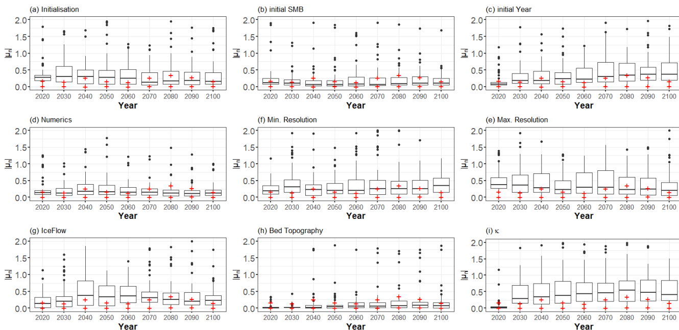
Figure 9: Statistics of |\mu_n| summarised by a boxplot at each time instant for all members of the MIROC5,RCP8.5-forced GrIS MME. The lower and upper red cross is respectively the 1 st and 3 rd quartile of the cross-validation error RAE_n . If the boxplot does not overlap with the region defined by the interval between the red crosses, this indicates that the influence measured by |\mu_n| can be considered significant with respect to the ML prediction error. For readability, the upper bound of the y-axis has been set up to 2.
