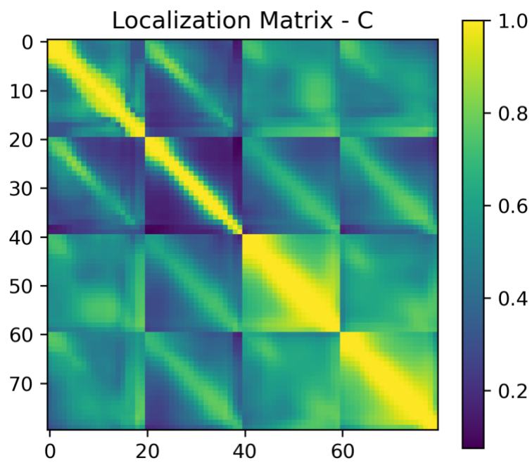
Figure 2: SPSD localization matrix constructed using non-negative eigenvalues
