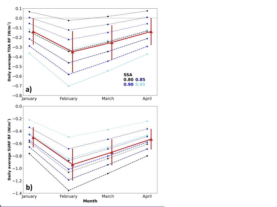
Figure 6: Time series, from January to April 2020, of the monthly means area-weighted global-equivalent TOA (panel a) and surface RF (panel b) (based on equinox-equivalent daily average RF), for the UTLS perturbation of Australian fires 2019-2020. Different shades of blue dots and lines are for different SSA values, darker the shade smaller the SSA. Dashed and dotted blue lines are for g values of 0.5 and 0.7, respectively. The red triangles and thick solid lines represent the mean TOA and surface global-equivalent RF, averaged over the whole SSA and g scenarios. Error bars represent their variability.
