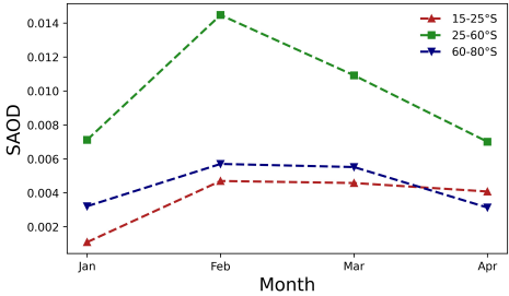
Figure 3: Monthly mean OMPS-LP stratospheric aerosol optical depth (SAOD), from January to April 2020, in the latitude interval 15-25°S (red upwards triangles and line), 25-60°S (green squares and line) and 60-80°S (blue downwards triangles and line).
