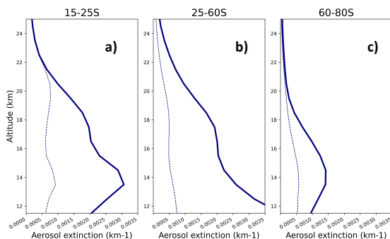
235 Figure 4: Monthly mean OMPS-LP aerosol extinction coefficient profiles at 675 nm, for the months of February 2020 (perturbed profiles, solid lines) and February 2019 (background profiles, dashed lines), in the latitude interval 15-25°S (panel a), 25-60°S (panel b) and 60-80°S (panel c).
