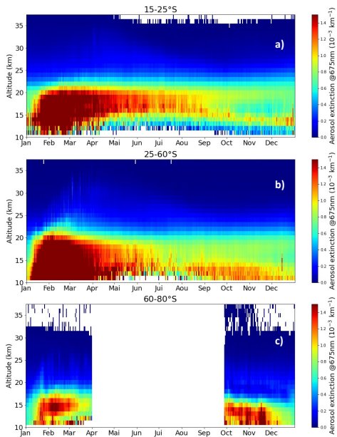
195 Figure 2: Time series of the vertical profiles of the aerosol extinction at 675 nm from OMPS-LP observations. Time series are shown as zonal averages in the latitude interval 15-25°S (panel a), 25-60°S (panel b) and 60-80°S (panel c). The period between April and September 2020 is excluded for the band 60-80°S due to limitations in the geographical sampling of OMPS-LP and its observation geometry.
