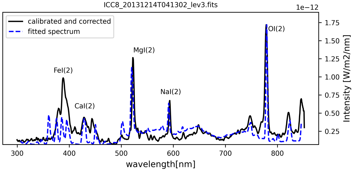
Figure 8. Calibrated spectrum (black line) and fitted spectrum (blue) of total image of event 20131214T041302
