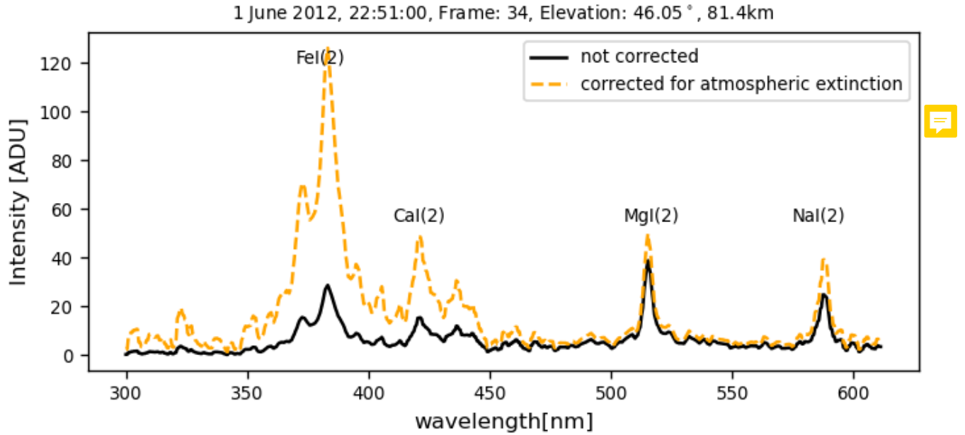
Figure 4. Example of ICC8 spectral profile before (black) and after (red) the atmospheric extinction correction.
