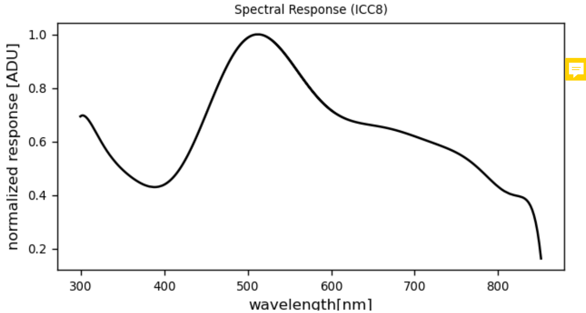
Figure 3. Normalized ICC8 spectral response curve
