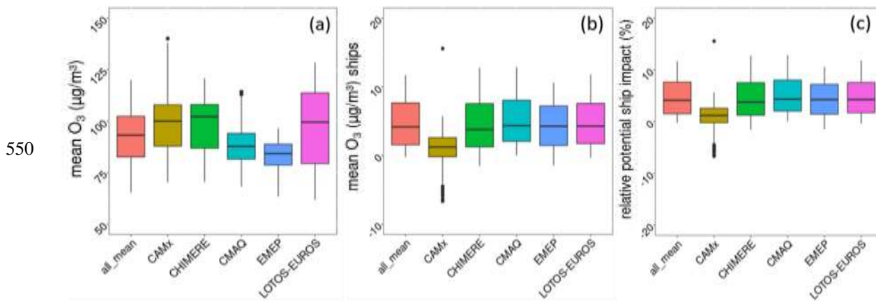
Figure 7: Annual mean for the whole model domain. (a) = mean O 3 for all emission sectors (base case), (b) = mean O 3 for shipping only, (c) = relative potential ship impact to total O 3 concentration. All_mean is the mean value of all models, with a median of (a) = 92.4 µg/m 3 , (b) = 4.0 µg/m 3 and (c) = 4.2 µg/m 3 .
