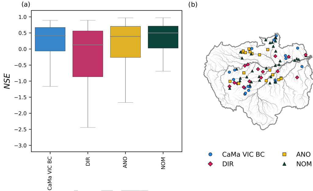
Figure 10. (a) Boxplot of Nash–Sutcliffe efficiency (NSE) for discharge simulated using CaMa-Flood with VIC bias-corrected runoff (CaMa-Flood VIC BC), ensemble mean assimilated river discharge (DIR), mean assimilated with anomaly DA (ANO), and mean assimilated with normalized value DA (NOM). (b) Spatial distribution of the best discharge estimates among CaMa VIC BC, DIR, ANO, and NOM based on NSE.
