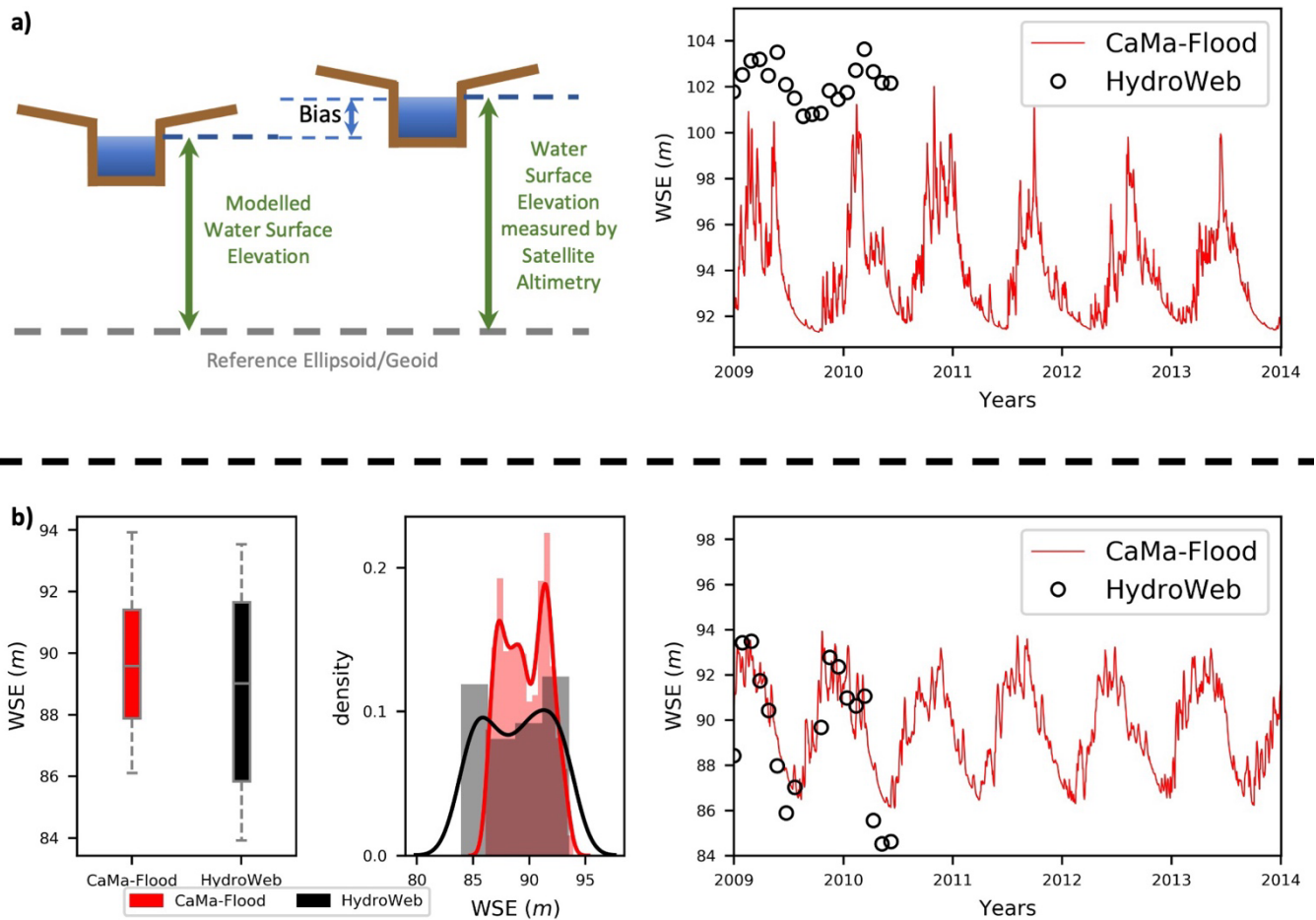
Figure 2: a) Schematic diagram of the bias between simulated and observed WSE and an example of the bias between simulated and observed water surface elevation (WSE) at the HydroWeb VS R_AMAZONAS_JARI_KM0529. b) Difference between simulation (CaMa-Flood) results and observations with distribution differences shown as a boxplot, probability distribution, and an example of difference in amplitude between simulated and observed WSE at the HydroWeb VS R_AMAZONAS_JUTAI_KM3182.
