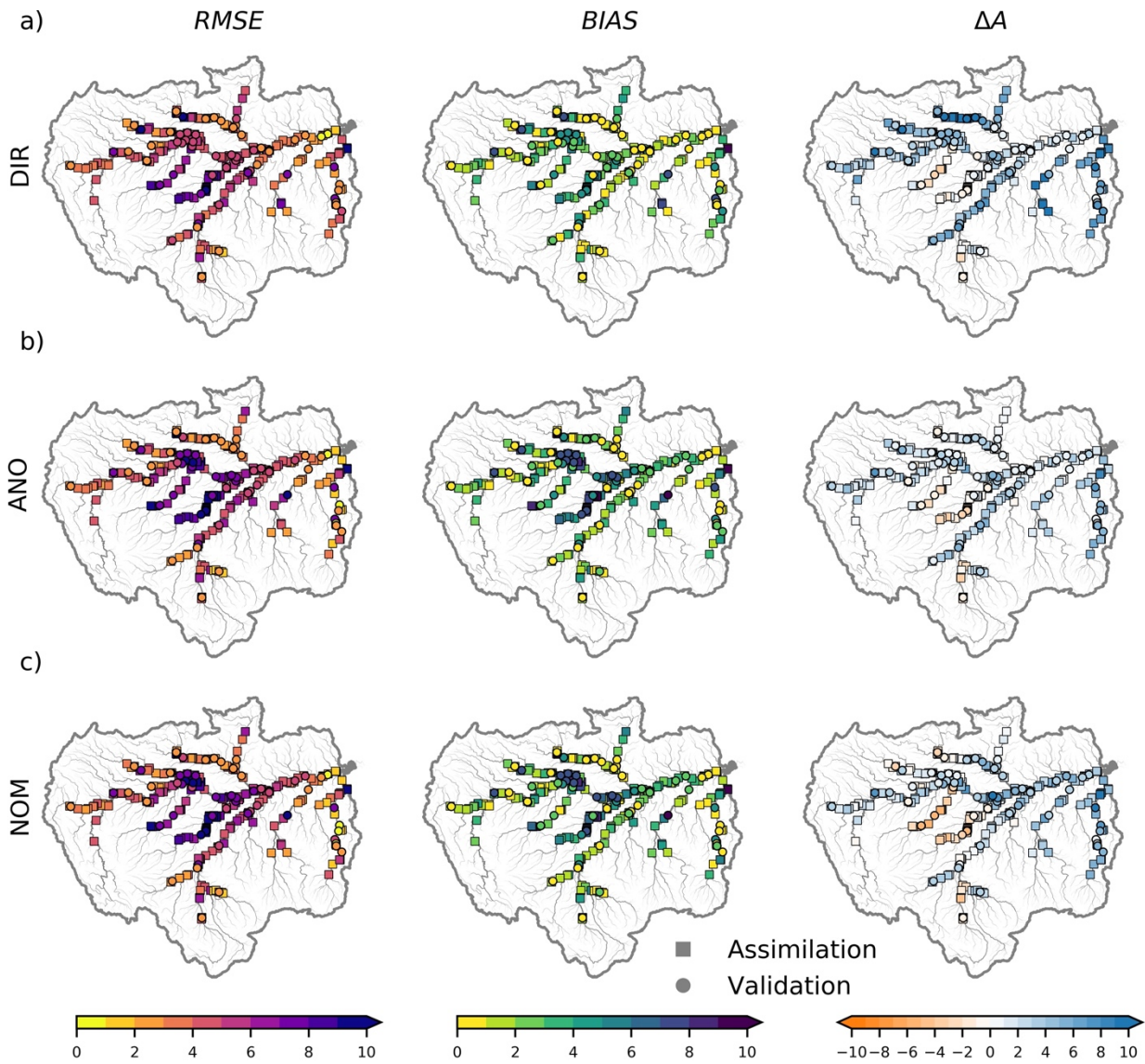
Figure 9: Performance of water surface elevation estimation in terms of the root mean square error ( RMSE ), bias between assimilation results and observations ( BIAS ), and mean differences in amplitude between assimilation results and observations ( \Delta A ) for a) DIR, b) ANO, and c) NOM.
