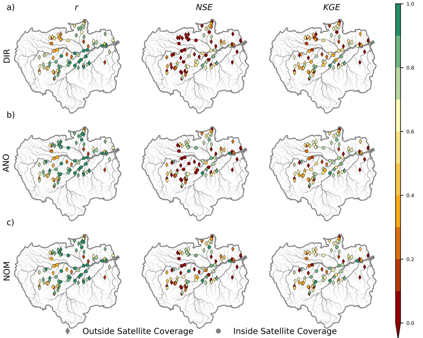
Figure 8: Performance of daily discharge in terms of the correlation coefficient ( r ), Nash-Sutcliffe efficiency ( NSE ), and Kling-Gupta efficiency ( KGE ) for a) DIR, b) ANO, and c) NOM. Diamonds and circles indicate the gauges outside and inside the satellite altimetry coverage, respectively.
