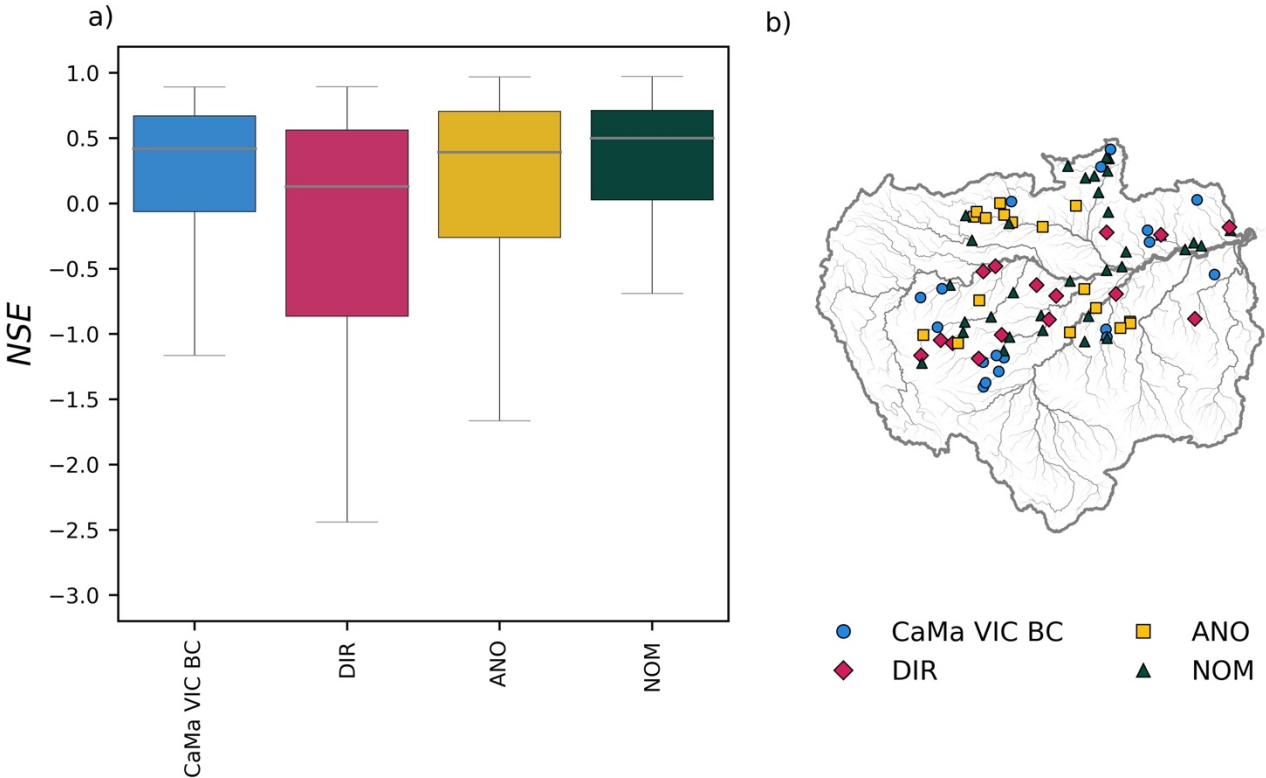
Figure 10: a) Boxplot of Nash-Sutcliffe efficiency ( NSE ) for discharge simulated using CaMa-Flood with VIC bias-corrected runoff (CaMa-Flood VIC BC), mean assimilated with direct DA (DIR), mean assimilated with anomaly DA (ANO), and mean assimilated with normalized value DA (NOM). b) Spatial distribution of the best discharge estimates among CaMa VIC BC, DIR, ANO, and NOM based on NSE .
