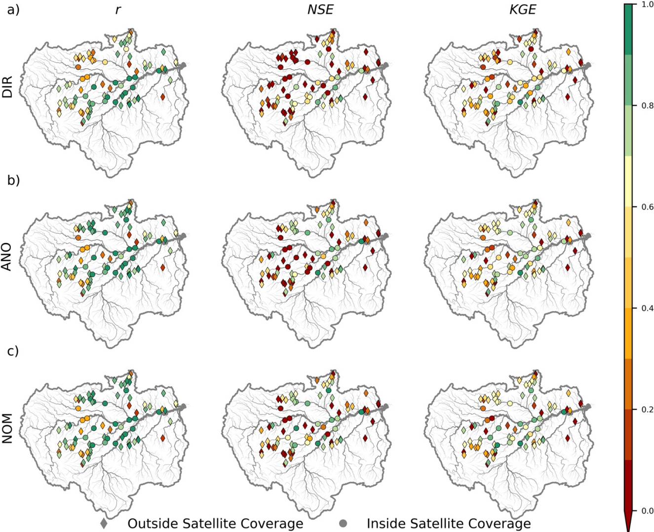
Figure 8: Performance of daily discharge in terms of the correlation coefficient ( r ), Nash-Sutcliffe efficiency ( NSE ), and Kling-Gupta efficiency ( KGE ) for a) \text{Exp-1DIR} , b) \text{Exp-2ANO} , and c) \text{Exp-3NOM} . Diamonds and circles indicate the gauges outside and inside the satellite altimetry coverage, respectively.
