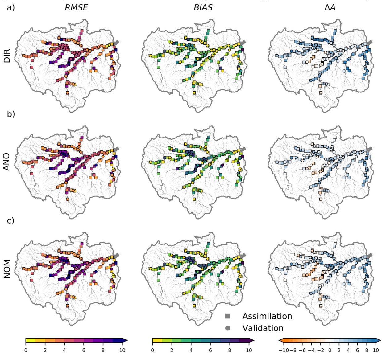
Figure 9: Performance of water surface elevation estimation in terms of the root mean square error ( RMSE ), bias between assimilation results and observations ( BIAS ), and mean differences in amplitude between assimilation results and observations ( \Delta A ) for a) Exp-1DIR , b) Exp-2ANO , and c) Exp-3NOM .
