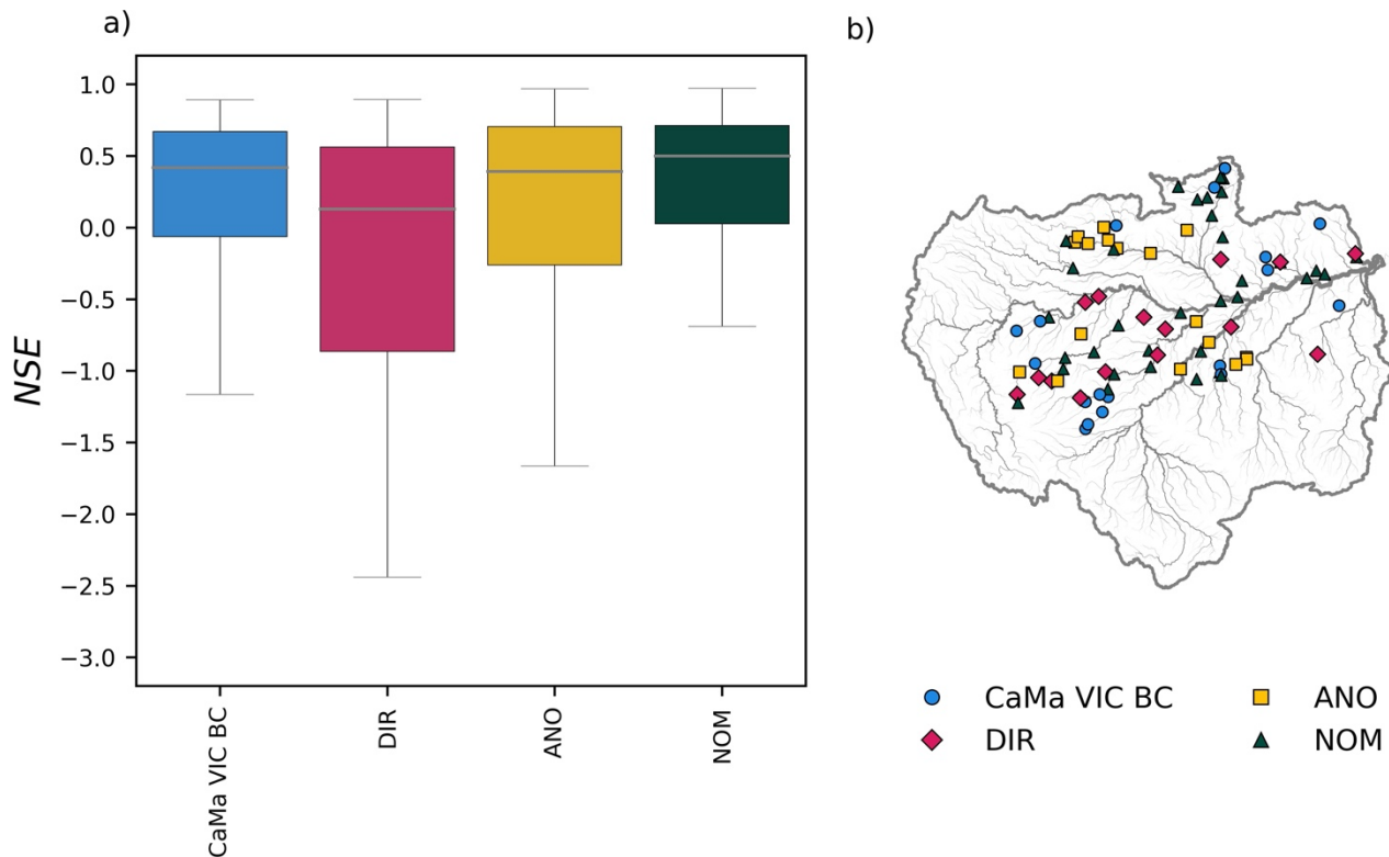
Figure 10: a) Boxplot of Nash-Sutcliffe efficiency ( NSE ) for discharge simulated using CaMa-Flood with VIC bias-corrected runoff (CaMa-Flood VIC BC), mean assimilated with direct DA ( Exp-1 DIR), mean assimilated with anomaly DA ( Exp-2 ANO), and mean assimilated with normalized value DA ( Exp-3 NOM). b) Spatial distribution of the best discharge estimates among CaMa VIC BC, Exp-4 DIR, Exp-2 ANO, and Exp-3 NOM based on NSE .
