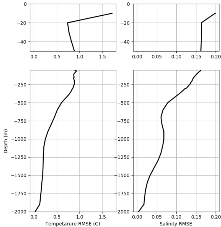
Figure 7. RMSE profiles for temperature ( ^{\circ}\text{C} ) and salinity ( \text{g/Kg} ) of the Moana Ocean Hindcast simulation in relation to the CORA5.2 observations. A zoom in of the first 50m where the larger differences are observed is provided in the upper row.
