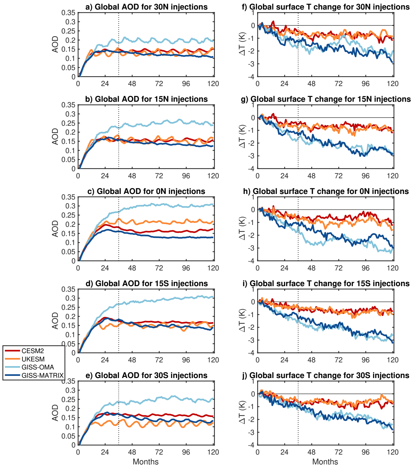
Figure 1. Timeseries of global mean monthly mean changes in stratospheric AOD (a-e) and surface temperature (f-f) resulting from the single-point injections at 30°N (a, f), 15°N (b, g), 0°N (c, h), 15°S (d, i) and 30°S (e, j) compared to the corresponding baseline SSP2-4.5 simulation in each of the models. The dashed line in all panels represent the month after which averages are performed for following figures (i.e. the last 7 years of simulations).
