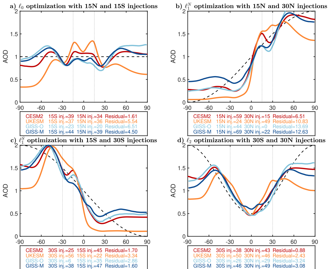
Figure 10. Linear least-squares solution to obtain an \ell_0 -shaped \ell_0 -shaped AOD (black dashed line) using only 15°N and 15°S injections (a), an \ell_0 + \ell_1 - \ell_0 + \ell_1 ( \ell_1^N , black dashed line, increased AOD in the Northern Hemisphere) one using only 15°N and 30°N injections (b), an \ell_0 + \ell_1 - \ell_0 - \ell_1 ( \ell_1^S , black dashed line, increased AOD in the Southern Hemisphere) one using only 15°S and 30°S injections (c) and a \ell_2 - \ell_2 (black dashed line, increased AOD at high latitudes compared to low latitudes) one using only 30°S and 30°S injections (d). Values at the bottom of each plot (in Tg-SO 2 /yr) indicate the required injection, assuming linearity, based on the AOD distribution in Figure 2. The residual of each solution is also included.
