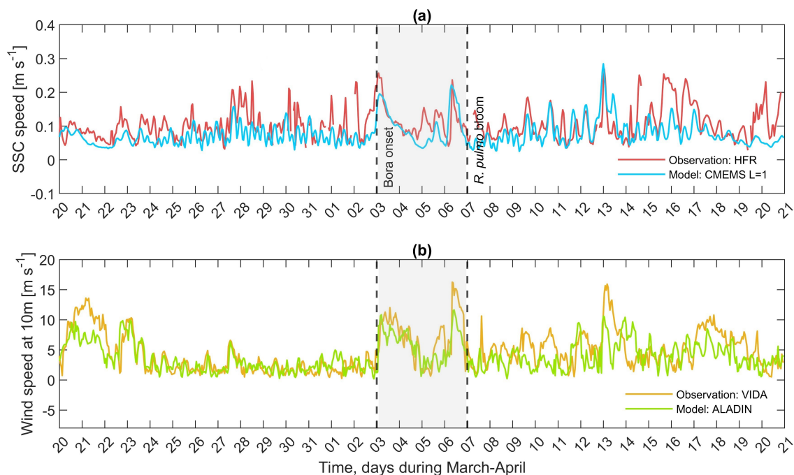
Figure 4. Times series of hourly: a) sea surface current (SSC) speed from CMEMS physical model (blue line) and HF radar (red line) spatially averaged over the extracted area; and b) wind speed from ALADIN atmospheric model (green line) and VIDA buoy (orange line) extracted at 13.55 °E, 45.55 °N and 13.55 °E, 45.63 °N respectively from the 20 March to 20 April 2021. The shadowed area represents the Bora-bloom period where the left-dashed black line delimits the starting of the Bora episode and the right-dashed black line represents the day when the jellyfish bloom was reported by the media and citizens.
