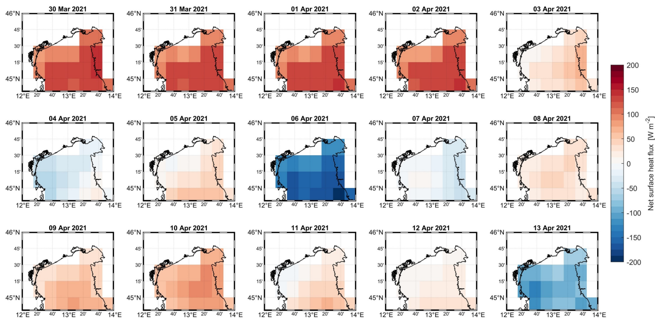
Figure 9. Spatial distribution of daily averaged net surface heat fluxes ( \text{Wm}^{-2} ) over the Northern Adriatic sea from 30 March to 13 April 2021.
