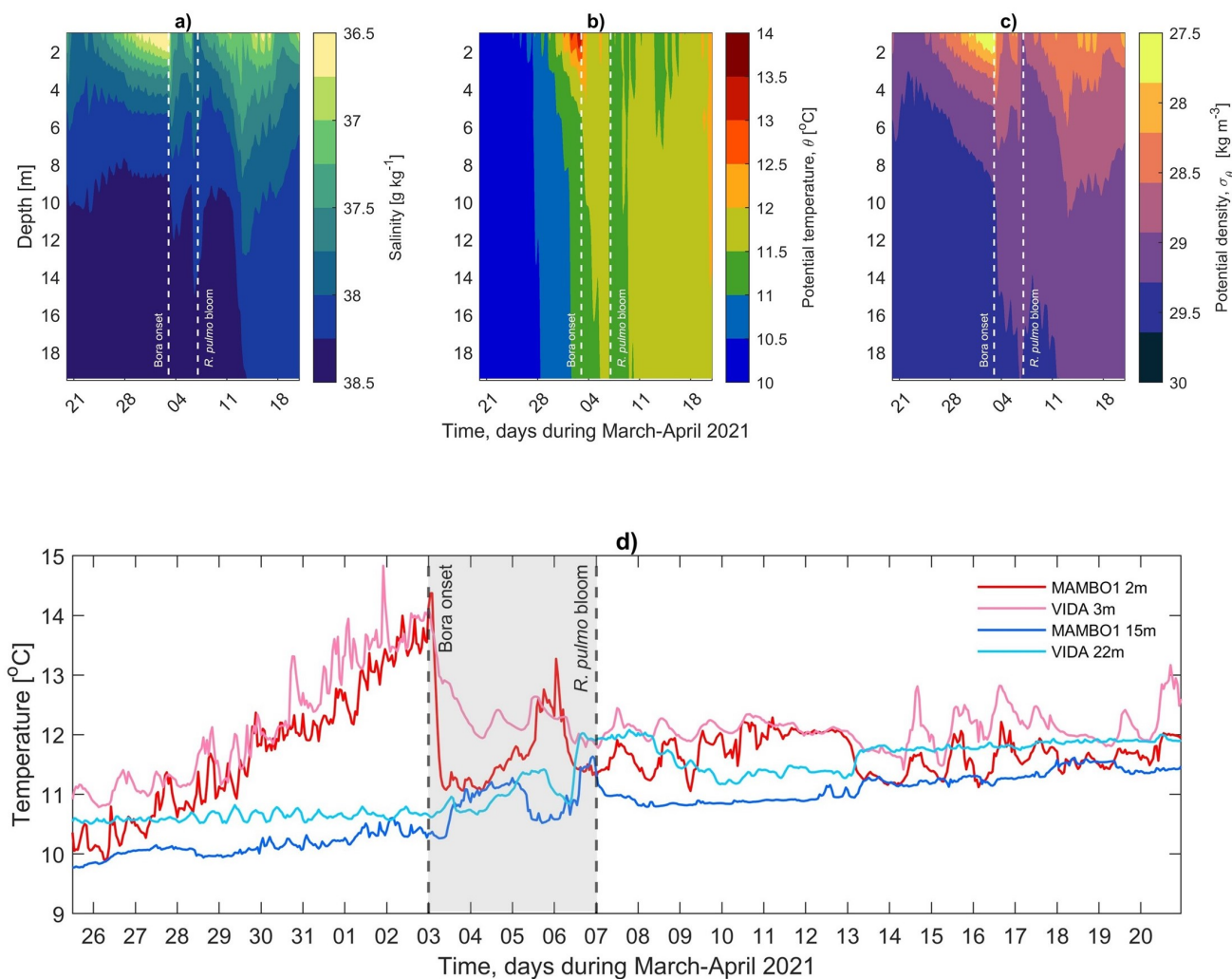
Figure 8. Hovmöller diagram of a) salinity, b) potential temperature and c) potential density extracted from CMEMS physical model for the period 20 March - 20 April 2021, d) temperature time series recorded in the MAMBO1 buoy at 2 m (red line) and 15 m (blue line), and VIDA buoy at 3 m (pink line) and 22 m (light blue line).
