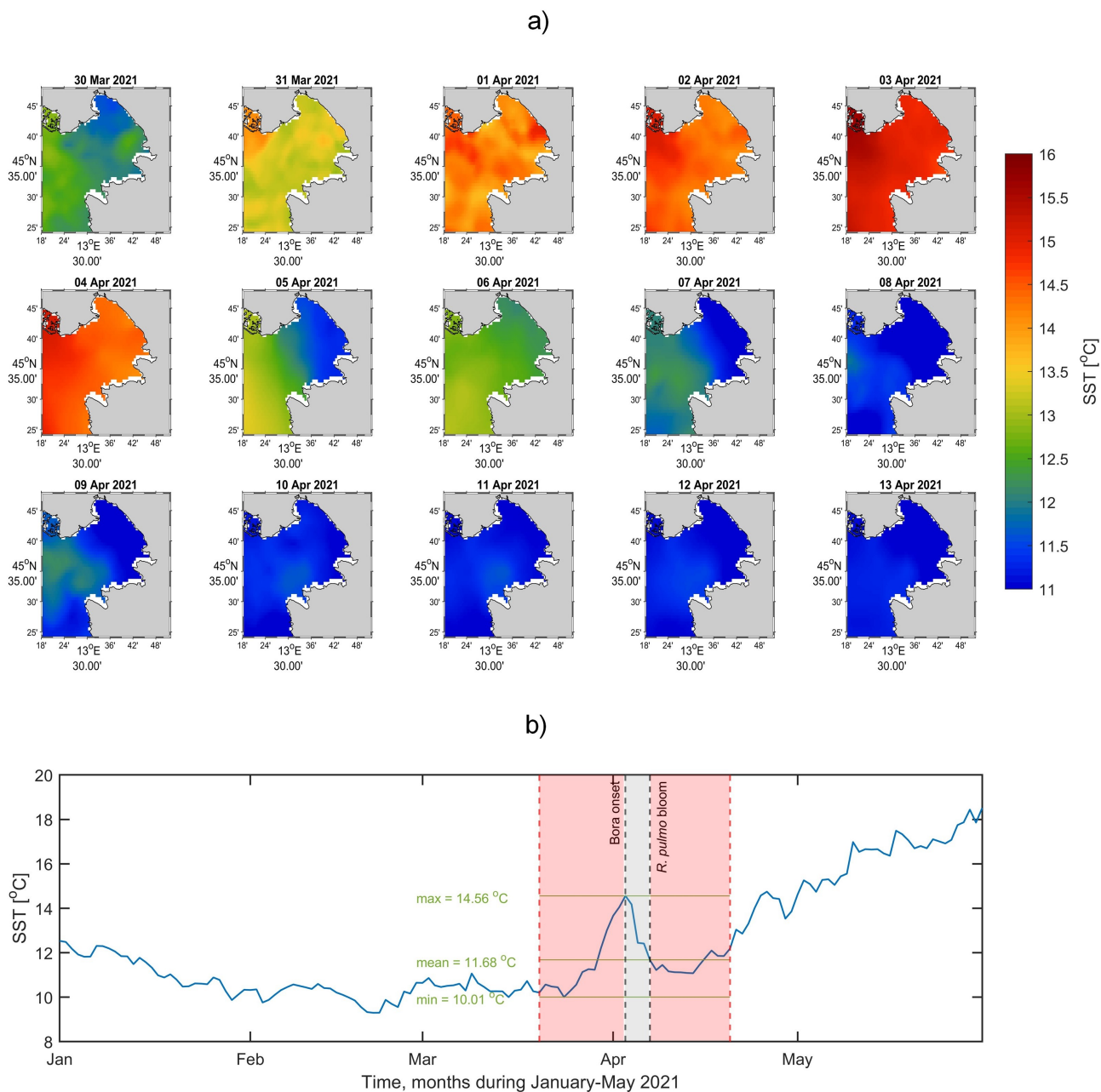
Figure 7. a) Maps of daily SST showing the evolution of the surface temperature field and the effect of the Bora wind in the GOT from 30 March to 13 April 2021. Here the colorbar represents the SST field in °C. b) Time series of the aforementioned dataset spatially averaged over the extracted area for the period 1 January to 30 May 2021. The shadowed grey area represents the Bora-bloom period where the left-dashed black line delimits the starting of the Bora episode and the right-dashed black line represents the day when the jellyfish bloom was reported by the media and citizens. The shadowed red between the dashed-vertical red lines delimits the interval 20 March - 20 April 2021 and the green lines represent the max, mean and min values during this interval.
