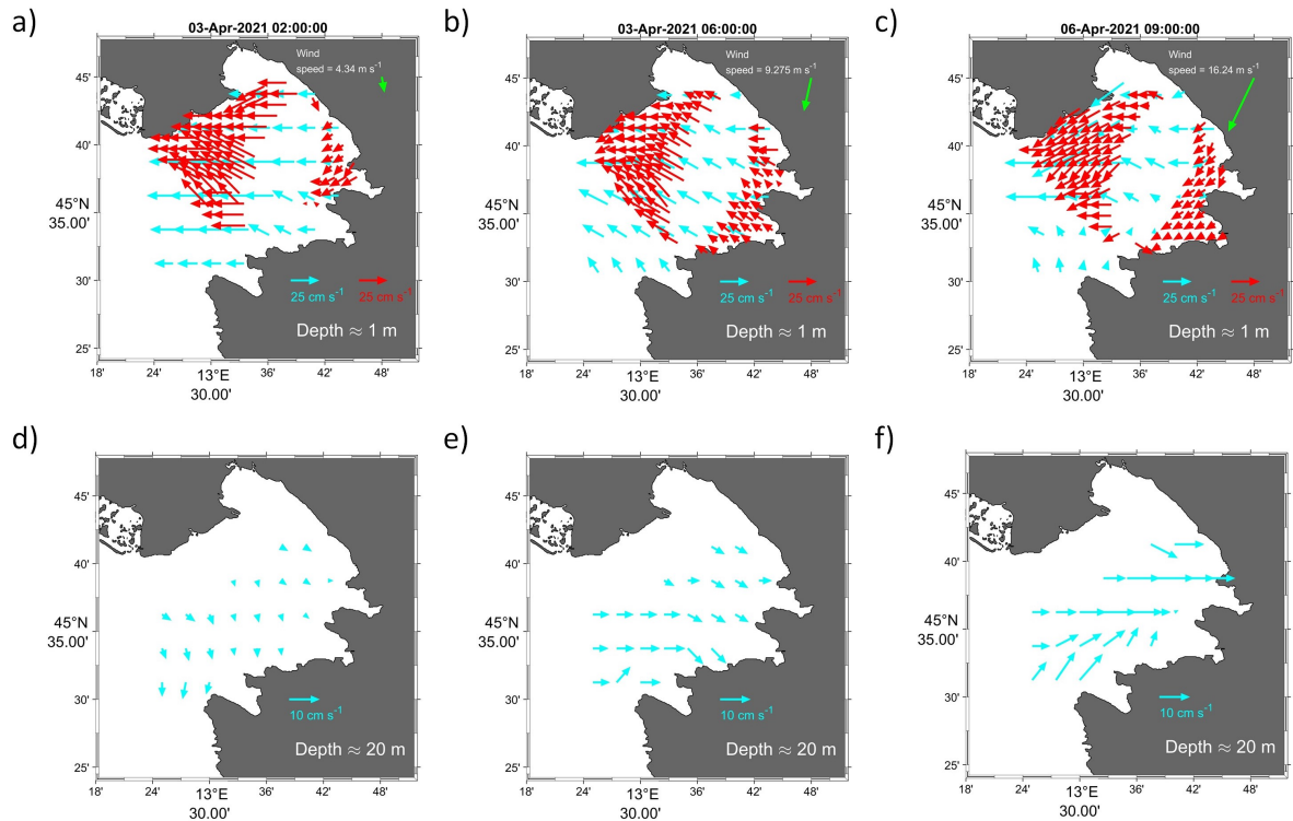
Figure 5. Maps of surface currents at \sim 1 \text{ m} from CMEMS model (blue arrows) and HFR (red arrows) on 3 April 2021 at 02:00 (a) and 06:00 (b), and on 6 April 2021 at 09:00 (c). Maps of bottom currents at \sim 20 \text{ m} from CMEMS model (blue arrows) on 3 April 2021 at 02:00 (d), 06:00 (e) and on 6 April 2021 at 09:00 (f). Green arrows represent wind speed in \text{m s}^{-1} .
