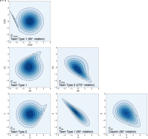
Figure 3. (a) A vine copula tree structure for atmospheric water balance components ( d = 4 ), where 1, 2, 3, and 4 represent water balance components. Note that the permutation is not unique and depends on model fitting; (b) Normalized bivariate copula contour plots of all pair copulas specified in the copula tree structure in (a). The contour colors represent the copula densities.
