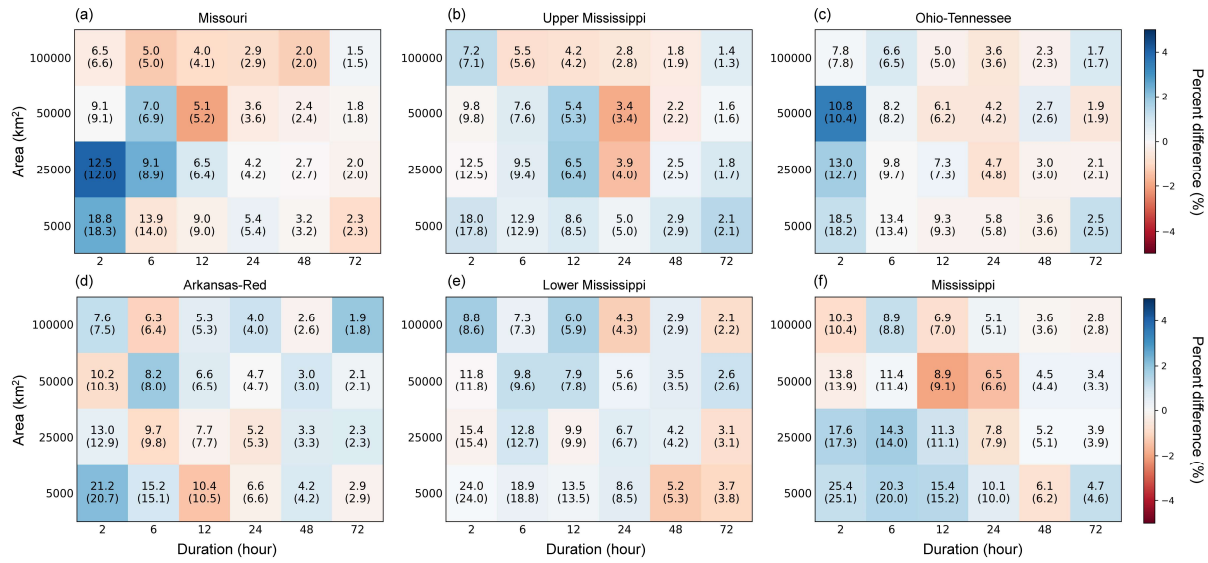
Figure A1. Estimated 10-year precipitation from vine copula and univariate GEV models. The GEV estimates are in parentheses.
