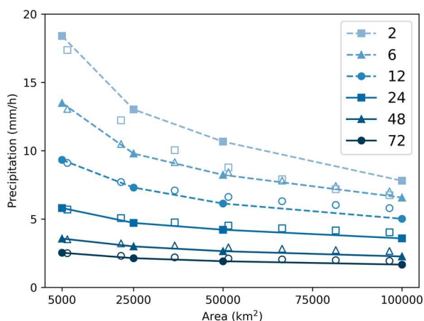
Figure C1 Comparison of DAD curves estimated from vine copulas (solid markers) and ARFs from Kao et al., 2020 (empty markers) for Ohio River Basin with 10-year ARI and 2-72 hours durations.
