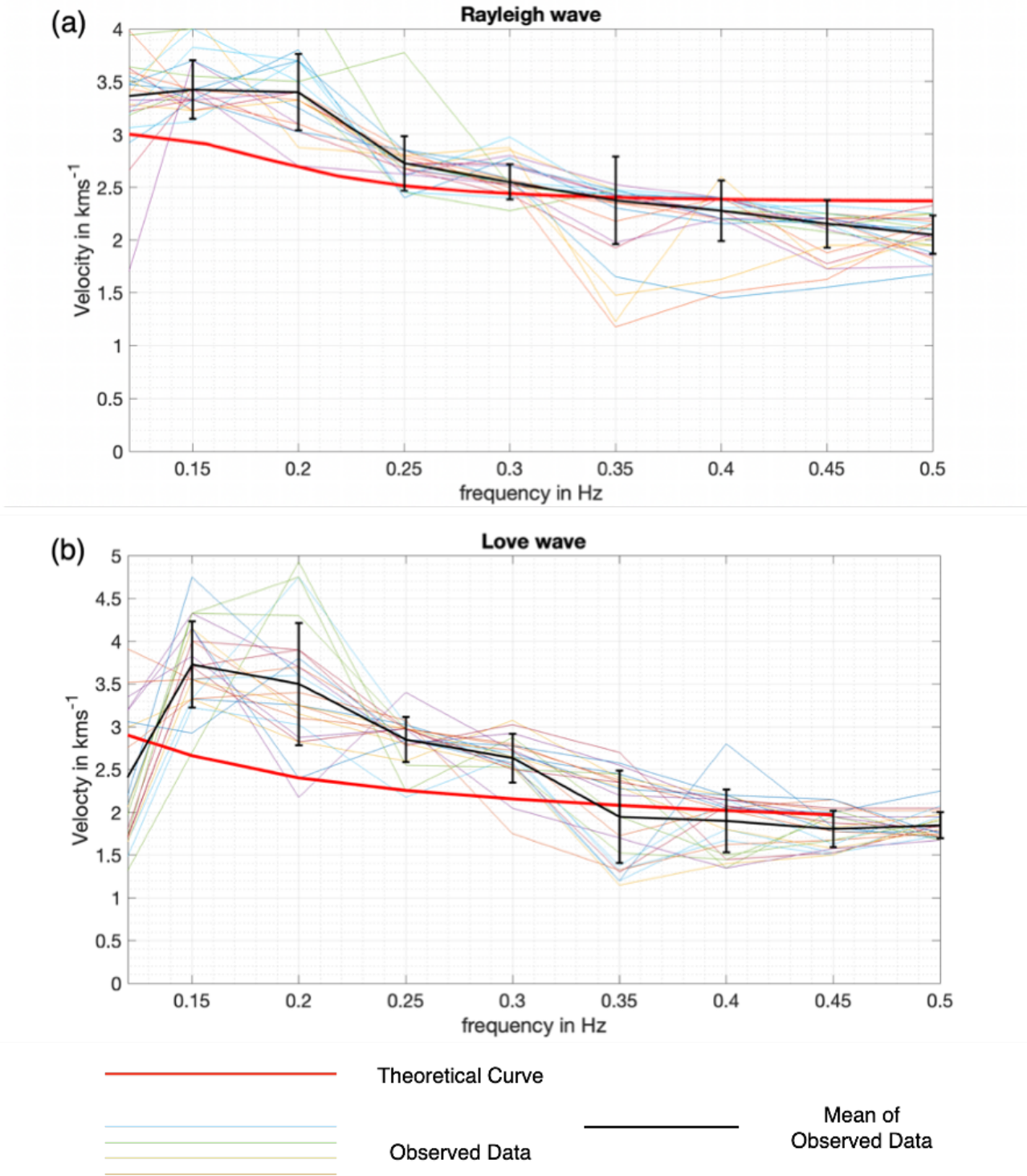
Figure 10. Dispersion curves for (a) Rayleigh waves and (b) Love waves, made using the 1-D velocity model from L  er et al. (2020). Observed dispersion curves (multi-coloured), mean observed curve (black) and theoretical curves (red), black bars represent the degree of error for the real data dispersion curves.
