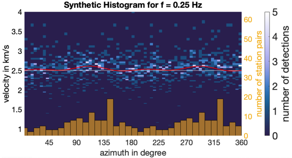
Figure 5. Histogram from synthetic data modelled from 10000-time 10000-time windows with fitted anisotropy curves from bootstrap resampling (grey) and the average curve shown in red. Bars on the bottom give the distribution of receiver-pair orientations.
