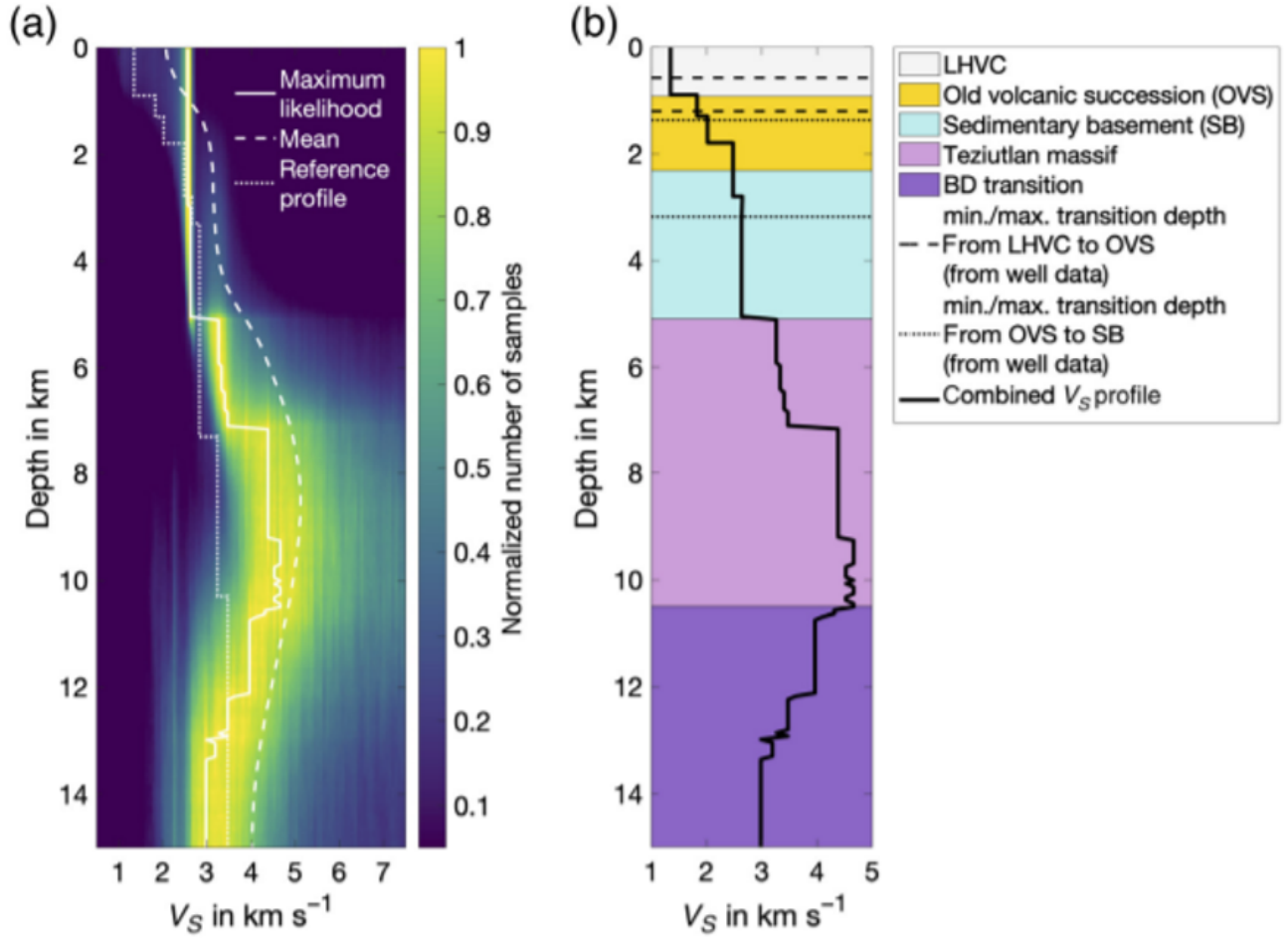
Figure B1. Velocity models used for producing fig-2 Fig. 3, from L  er et al. (2020). a) Probability density function (PDF) of shear-velocity distribution. (b) Combined shear-velocity profile (black) from the analysis of earthquake data (dotted curve in panel (a), down to 3.2 km depth) and ambient noise beamforming.
