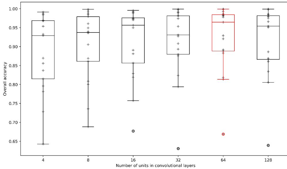
Figure 5. Temporal cross validation. Red highlights the best architecture with 64 convolutional units. The graph illustrates temporal cross validation results using box-plots. Each box-plot contains 17 overall accuracy values and if read from left to right each box-plot corresponds to 4, 8, 16, 32, 64, and 128 convolutional units in each convolutional layer. Red highlights the best architecture with 64 convolutional units.
