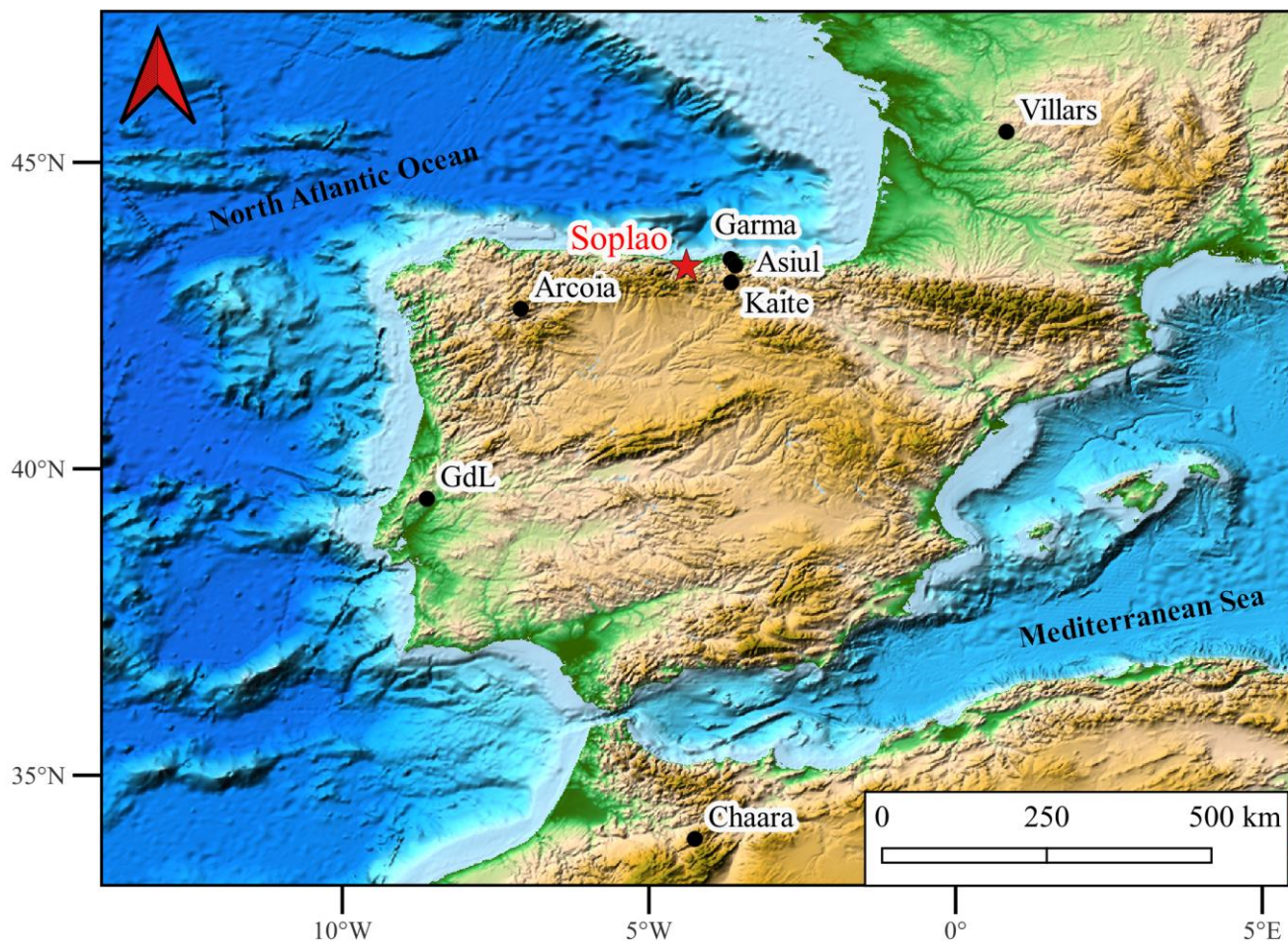
Figure 1: Location of the main palaeoclimate records discussed in the text: Soplao (El Soplo Cave: this study); Garma (La Garma Cave: Baldini et al., 2019); Kaite (Kaite Cave: Domínguez-Villar et al., 2009; 2017); GdL (Galeria das Lâminas: Benson et al., 2021); Chaara (Chaara Cave: Ait Brahim et al., 2019); Asiul (Cueva de Asiul: Smith et al., 2016); Arcoia (Cova da Arcoia: Railsback et al., 2011); Villars (Villars Cave: Ruan, 2016). Base map (ETOPO1 1 Arc-Minute Global Relief Model) collected from NOAA National Geophysical Data Center and map created in QGIS.
