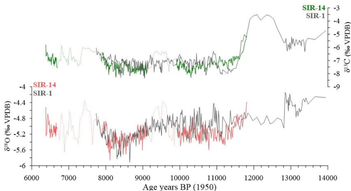
Figure S5. Comparison between stalagmite SIR-14 and SIR-1 isotope records. Overall, the \delta^{18}\text{O} and \delta^{13}\text{C} records of SIR-14 replicates well with the SIR-1 isotope records. However, SIR-1 does not replicate the oldest slow-growth interval recorded in SIR-14 (see sect. 5.1.1 in the manuscript). This is explained as a localised perturbation of infiltration at that specific drip site. The 8.2 ka event is also absent in the SIR-1 record. We hypothesize that this could be due to the fact that SIR-1 has several outliers (age-inversions) which potentially could put the record slightly out of phase, with the excursion at ~8.4 ka BP potentially recognised as the 8.2 ka event. However, this remains unknown, and cannot be resolved due to SIR-1's complex U-Th age results and derived age model.
