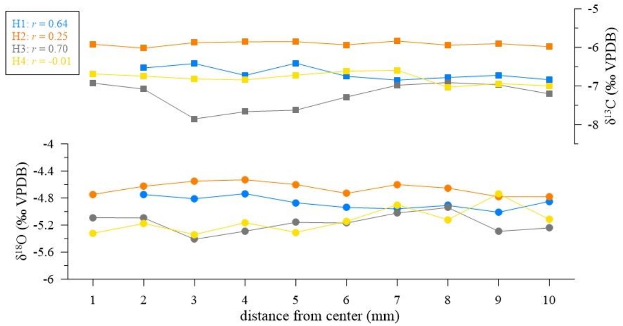
Figure S4. \delta^{18}\text{O} (circles) and \delta^{13}\text{C} (squares) measurements along single laminae in SIR-14 (Hendy test: Hendy, 1971), each plotted on their respective axes. Each lamina is shown by a unique colour (H1 = blue, H2 = orange, H3 = grey, H4 = yellow), and its location is marked with the same numbers (H1-H4) in fig. 3 (in the manuscript). Lamina H2 and H4 are not correlated; however, lamina H1 and H3 have a moderate correlation. There is a scatter of values in the \delta^{18}\text{O} within a single lamina (up to 0.6 ‰), however, there is no clear trend of enrichment from the central axis zone towards the flanks of the stalagmite.
