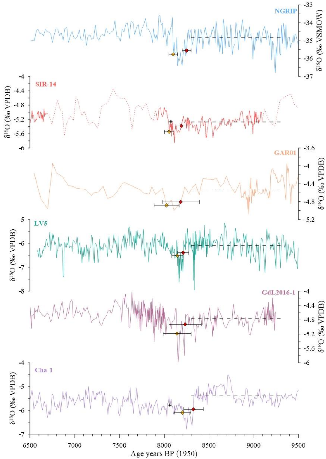
Figure S6. Identification of the 8.2 ka event in various archives. The final defined onset and end of the event is shown by red and yellow markers, respectively. Initially, we used the statistical approach by Thomas et al. (2007) to define the duration of the event, where the onset (end) of the 8.2 ka event is defined as the first (last) isotopic data point below the baseline (stapled black line) that precedes the event (Thomas et al., 2007). In cases where the position of the onset/end did not visually match the structure of the event in the NGRIP ice core, the onset/end isotopic data point was shifted to a structurally similar position. The statistically defined isotopic points for the onset (end) are marked as black circles (black crosses) to show the initial position before moving it to its position based on visual observation.
