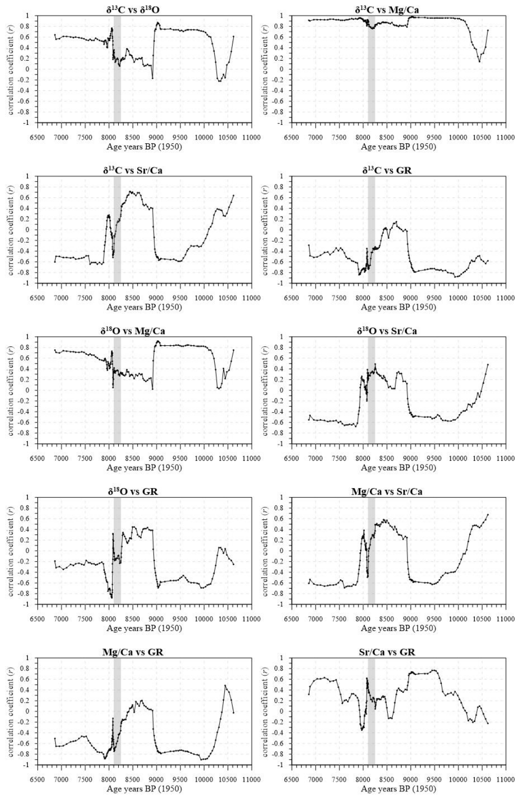
Figure S3. The 30-point running correlation coefficients for the measured proxies in stalagmite SIR-14 ( \delta^{13}\text{C} , \delta^{18}\text{O} , \text{Mg/Ca} , \text{Sr/Ca} and growth rate (GR)). This highlights time intervals of higher positive (and negative) correlation. The grey-shaded area shows the duration of the 8.2 ka event from the NGRIP ice-core record (Thomas et al., 2007).
