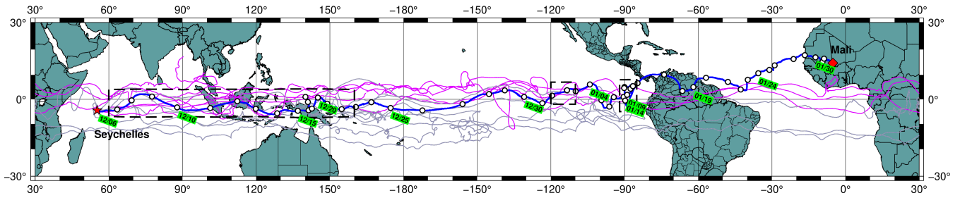
Figure 1. Trajectories of all balloons launched in the Strateole-2 2019 campaign. The thick blue line is balloon “ST2_C0_06_STR1” that carried the radio occultation receiver. \star marks the launch site in Seychelles and \diamond indicates the final landing site in Mali. Small circles over the trajectory indicate 00Z each day and are labeled at 5 day intervals. Dashed boxes along the trajectory mark the periods when BRO data were recovered. Gray lines are the 4 other balloons flying at \sim 20 km, and magenta lines are the 3 balloons flying at \sim 18 km.
