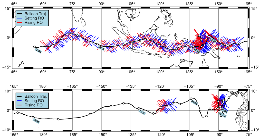
Figure 4. Plan view of the slant BRO profiles from 06 to 22 December 2019 (top), and a few selected days in January 2020 (1, 9, 11, 12, 13) (bottom). The thick black line marks the trajectory of the balloon at the altitude of \sim 20 km. Red and blue lines denote rising and setting BRO profiles, respectively, that are projections of slanted profiles with the lowest-highest tangent point on the furthest from the balloon path and the lowest point furthest away . Small circles mark 00Z each day and are labeled with the date at 5 day intervals. Galileo and GLONASS data were recovered on 15 December and Beidou data were recovered on 14 January but not included in this map.
