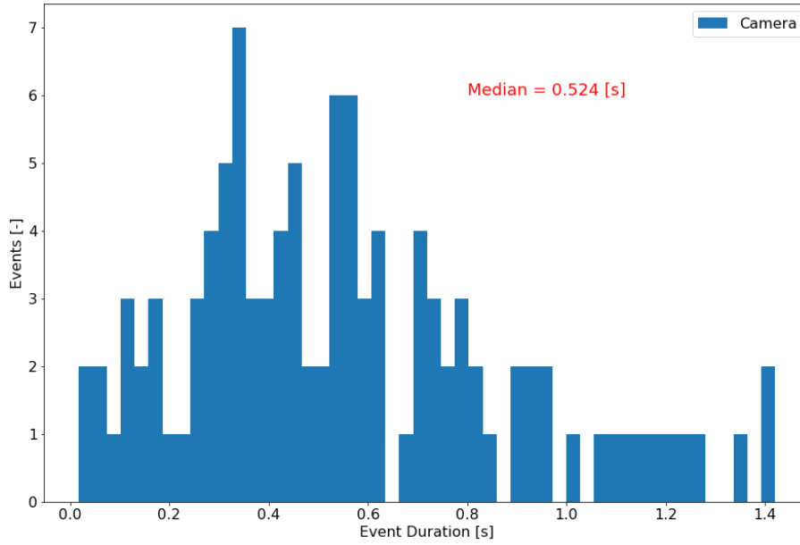
Figure 19. Histogram of the observed duration of lightning events. The histogram is based on data captured by the high-speed cameras.
