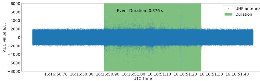
Figure 18. Example of lightning duration measurement based on radio signals captured by the UHF receiver. The time duration of lightning is marked by the green overlay.
