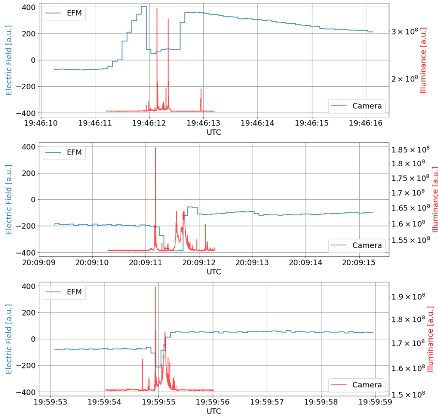
Figure 16. Detail of EFM data with a comparison with camera data.
