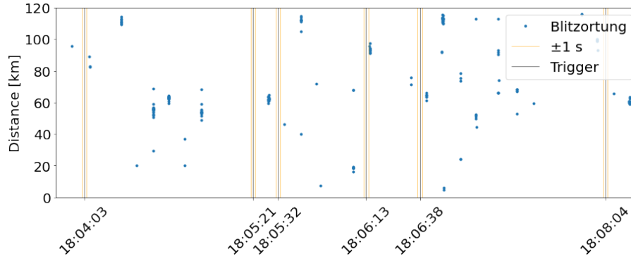
Figure 13. Correlation with “nearby” (less than 20 km) lightning detection.
