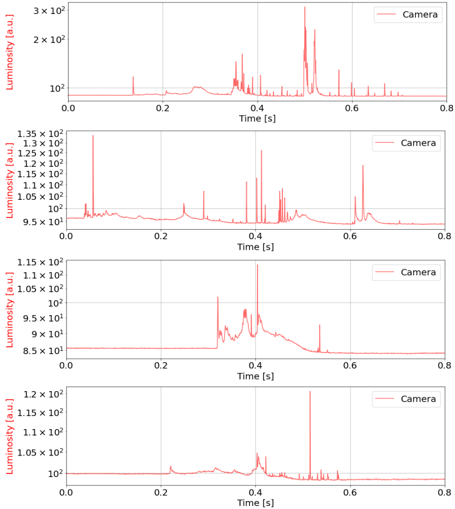
Figure 11. An example of luminosity curves for a few lightning.
