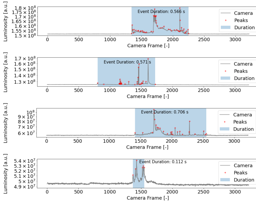
Figure 17. Examples of detection of lightning events duration. Red crosses are detected peaks in signals generated by lightning processes. The determined length of lightning duration is highlighted. The duration of the camera frame is 620 \mu s.
