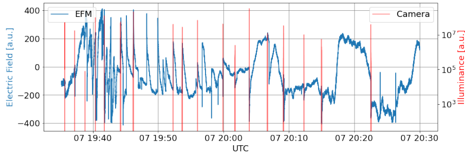
Figure 15. Example of measurement with EFM compared with records of lightning captured on the camera.
