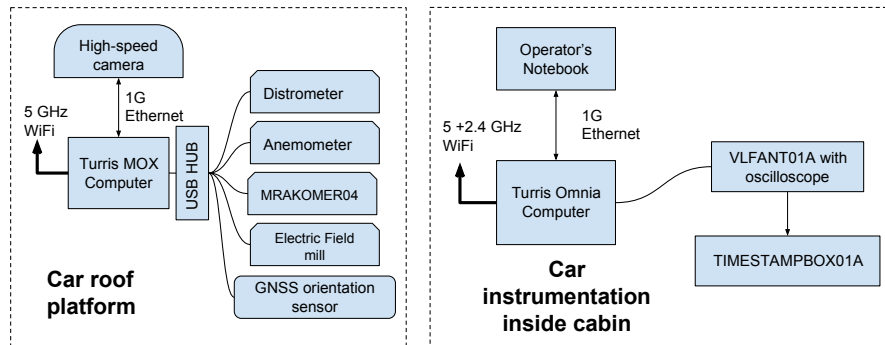
Figure 6. CRREAT CAR1 instrumentation schematic diagram.
