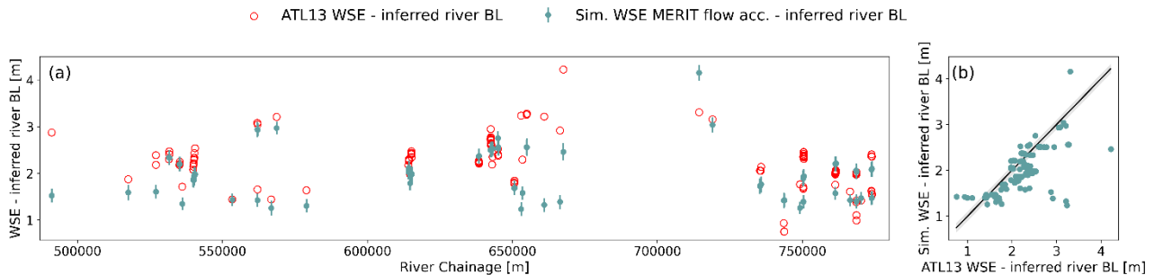
435 Figure 9. (a) Validation longitudinal profile using the steady state solver for uniform depth and MERIT flow accumulation between Jimai and Mentang. (b) Simulated vs. ATL13 WSE minus inferred BL, the shaded area correspond to the mean standard deviation in the ATL13 product, extracted from the flag stdev_water_surf .
