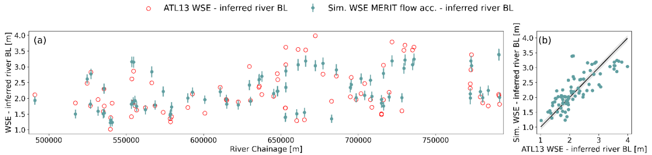
425 Figure 8. (a) Calibrated longitudinal profile using the steady state solver for uniform depth and MERIT flow accumulation between Jimai and Mentang. (b) Simulated vs. ATL13 WSE minus inferred BL, the shaded area correspond to the mean standard deviation in the ATL13 product, extracted from the flag stdev_water_surf .
