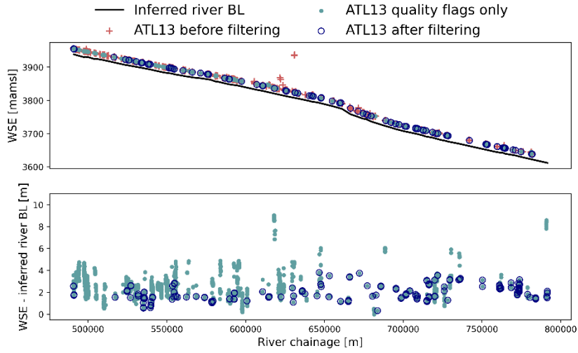
390 Figure 6. Top: ATL13 WSE along river chainage, before processing, after quality filters are applied and after filtering criteria. Bottom: ATL13 WSE minus inferred BL from the model calibration comparing the quality filters results and the filtering criteria.
