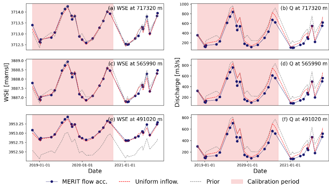
Figure 13. Simulated WSE (a), (c) and (e) and simulated discharge (b), (d) and (f) at selected chainage points. The simulated WSE and Q from MERIT flow acc. inferred parameters is compared with the results using uniform inflow and the prior guess.
