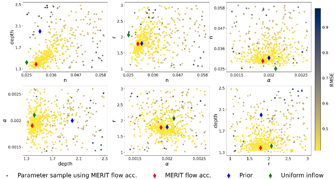
Figure 7. Sampling pattern and model performance during calibration using MERIT flow accumulation map. The objective function is lowered during calibration.
