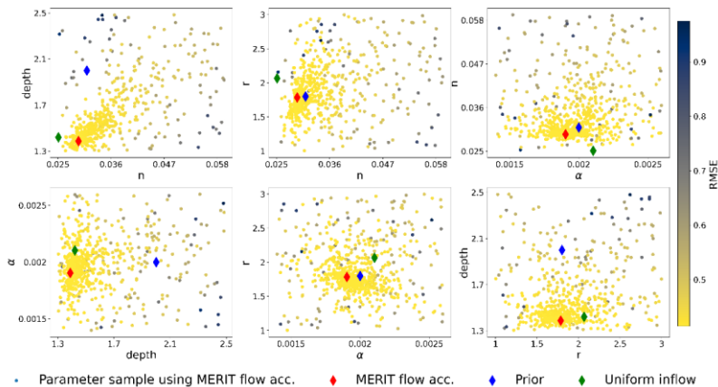
Figure 7. Sampling pattern and model performance during calibration using MERIT flow accumulation map. The objective function is lowered during calibration.
