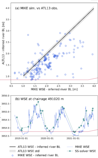
Figure 14. (a) MIKE Hydro simulated WSE vs. ATL13 WSE minus inferred BL. The shaded area corresponds to the median std. deviation of the ATL13 observations, taken from the flag stdev_water_surf. (b) Simulated WSE from the steady state solver and MIKE.
