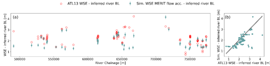
Figure 9. (a) Validation longitudinal profile using the steady state solver for uniform depth and MERIT flow accumulation between Jimai and Mentang. (b) Simulated vs. ATL13 WSE minus inferred BL, the shaded area correspond to the mean standard deviation in the ATL13 product, extracted from the flag stdev_water_surf.
