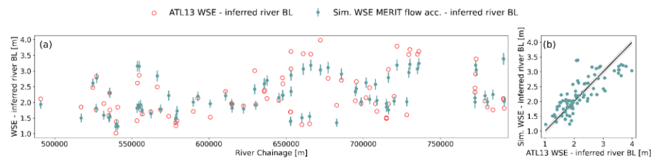
Figure 8. (a) Calibrated longitudinal profile using the steady state solver for uniform depth and MERIT flow accumulation between Jimai and Mentang. (b) Simulated vs. ATL13 WSE minus inferred BL, the shaded area correspond to the mean standard deviation in the ATL13 product, extracted from the flag stdev_water_surf .
