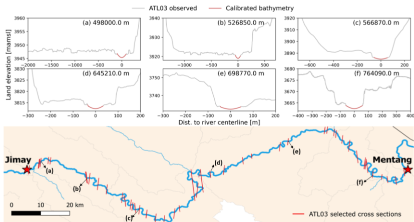
385 Figure 5. Top: Examples of cross section geometry after calibration, where the majority of points correspond to ATL03 observed data. Bottom: ATL03 selected cross-sections for river hydraulic calibration. 80 cross-section were selected after processing described in section 2.1.1. The cross-section shown in the top plot are located in the river.
