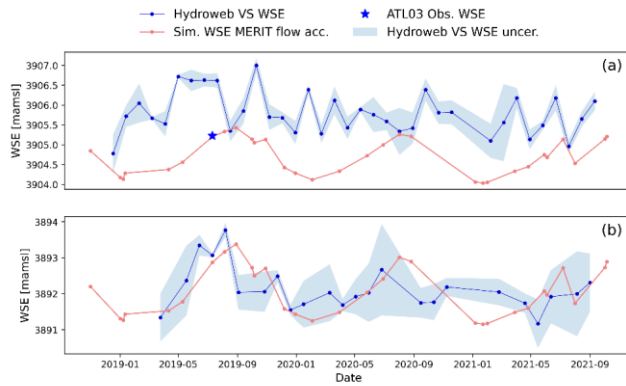
Figure 12. Comparison of estimated WSE with available Hydroweb VS it the AOL. The WSE at VS is derived from Sentinel-3A observations. (a) Simulated WSE at chainage 545030 m vs. WSE at VS 4914 km and (b) Simulated WSE at chainage 560360 m vs. WSE at VS 4901 km.
