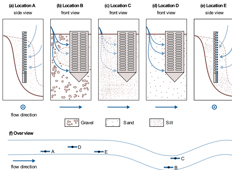
Figure 3: Schematic representation of potential hyporheic flow paths (blue arrows) at the five sampling sites. For locations A and E, a side view was chosen and for locations B, C and D a front view. Where the front view is shown, flow direction in the river is from left to right and where the side view is shown flow direction is out of the drawing plane. The color strength of the arrows corresponds to the expected magnitude of hyporheic fluxes. The sediment composition is schematically indicated. Quantitative data on the sediment composition at the five locations can be found in Supplement 1.
