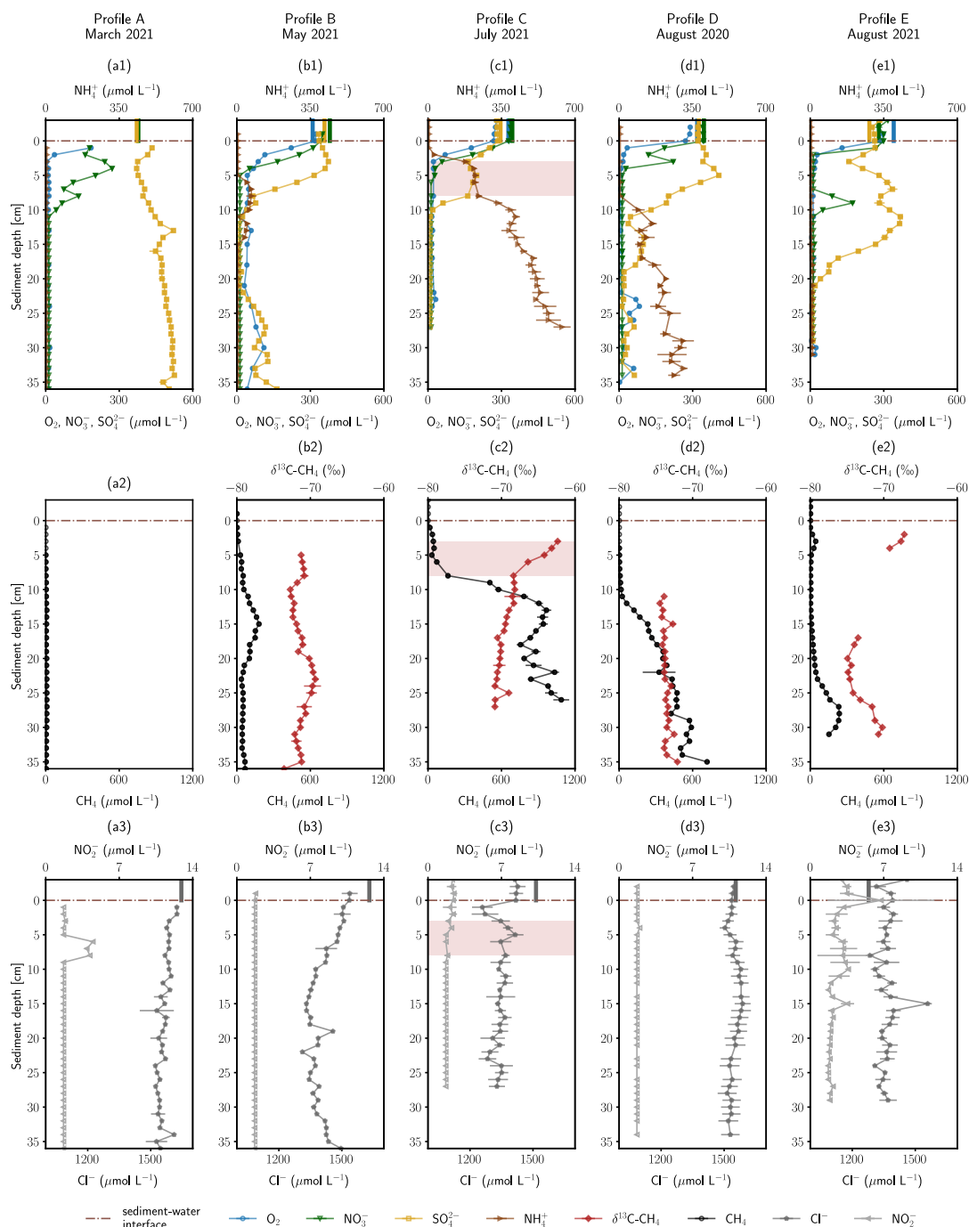
Figure 2: Depth-resolved profiles of hyporheic pore-water geochemistry at five sampling sites. Panels (a1) to (e1) show O_2 , NO_3^- , NH_4^+ and SO_4^{2-} concentrations, panels (a2) to (e2) CH_4 concentrations and \delta^{13}C-CH_4 values and panels (a3) to (e3) NO_2^- and Cl^- concentrations. Empty markers indicate values outside the range of used standards. Error bars show standard deviations of independent measurements ( n=3 ). Vertical lines above the sediment-water interface are concentrations measured in the surface water at the sampling date. Red background color highlights an enrichment in \delta^{13}C-CH_4 . Profiles are ordered by season.
