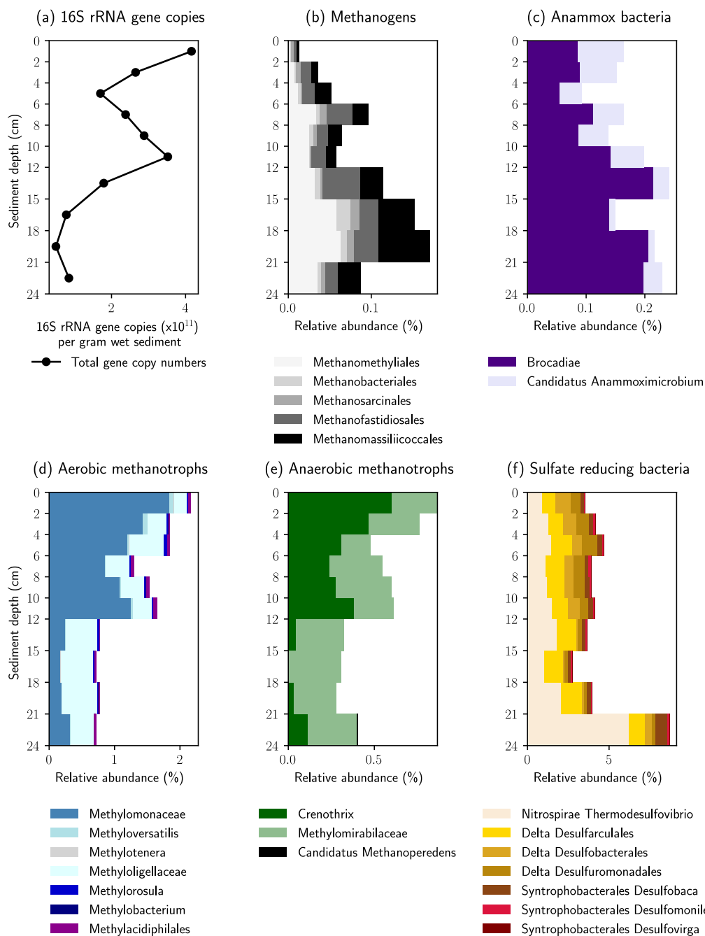
Figure 5: Relative abundance of key microbial groups detected in the 16S rRNA gene sequencing datasets. The histograms display the relative abundance (% of total reads) assigned to each group displayed. Note the increase in relative abundance of methanogenic groups below 12 cm, whereas the relative abundance of methane oxidizing groups increases above 12 cm.
