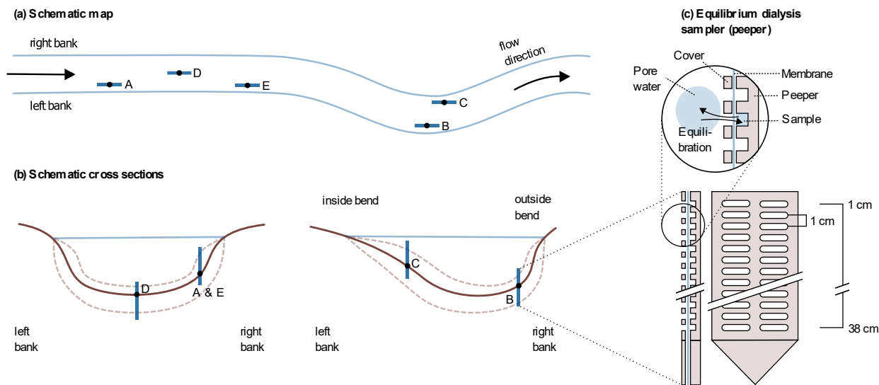
Figure 1: Schematic representation of the five sampling sites along the river (a) and across the river bed (b). In (c), the sampler is schematically drawn, modified after Teasdale et al. (1995) (top: detail, bottom left: side view; bottom right: front view; for clarity, only 12 of the 38 chambers are illustrated).
