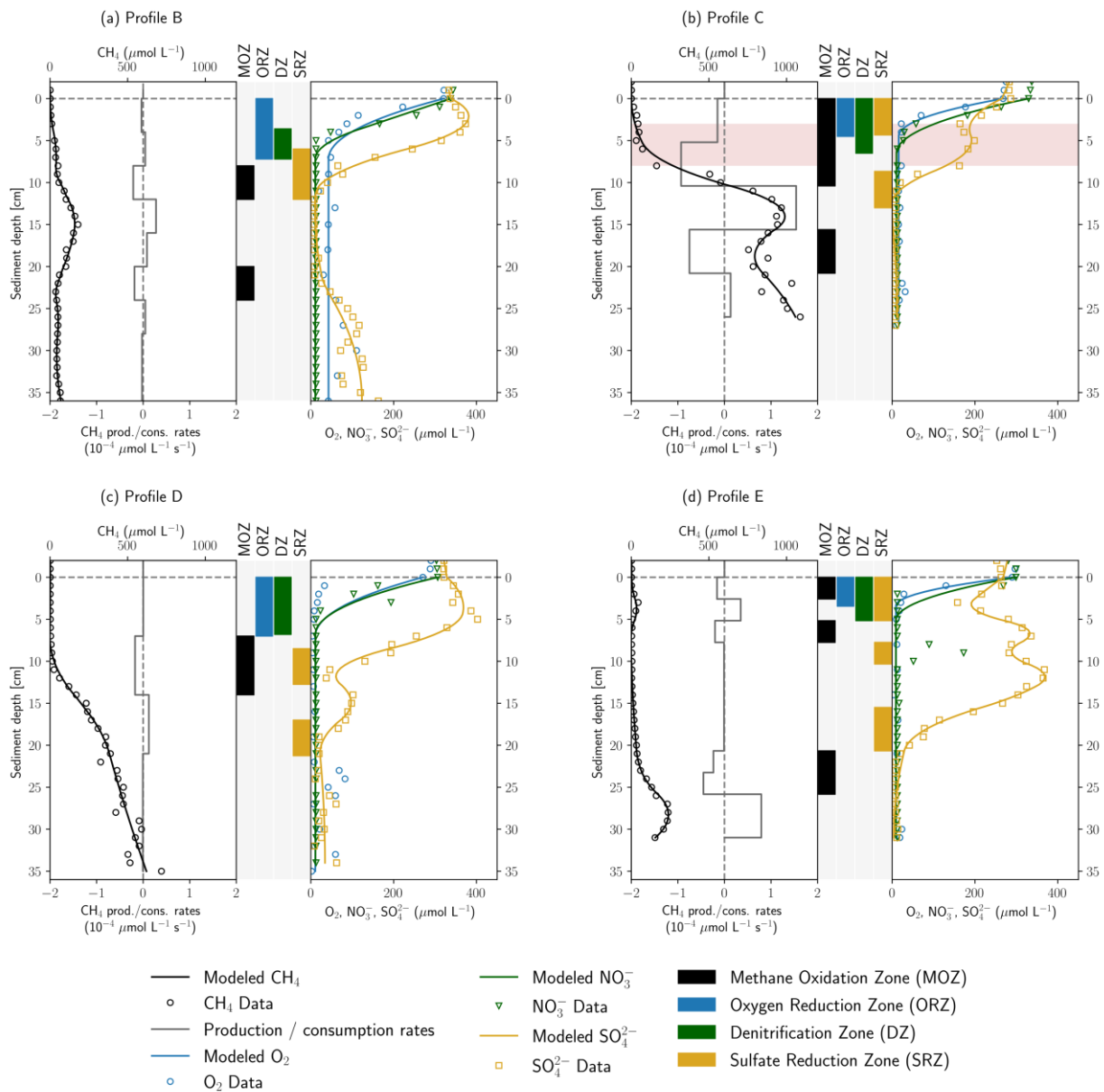
Figure 5: Results of concentration gradient modeling using the PROFILE software for profiles B-E. In each panel (a)-(d), the left side shows modeled and measured CH 4 concentrations as well as modeled CH 4 production and consumption rates. In the center, the depth ranges of MOZ, ORZ, DZ and SRZ are highlighted. Zones with very low consumption rates ( <5 \cdot 10^{-6} \mu\text{mol L}^{-1} \text{s}^{-1} ) were not identified. On the right, measured and modeled O 2 , NO 3 - and SO 4 2- concentrations are shown. Rates are not displayed for electron acceptors for reasons of clarity. Red background color in panel (b) highlights an enrichment in \delta^{13}\text{C-CH}_4 .
