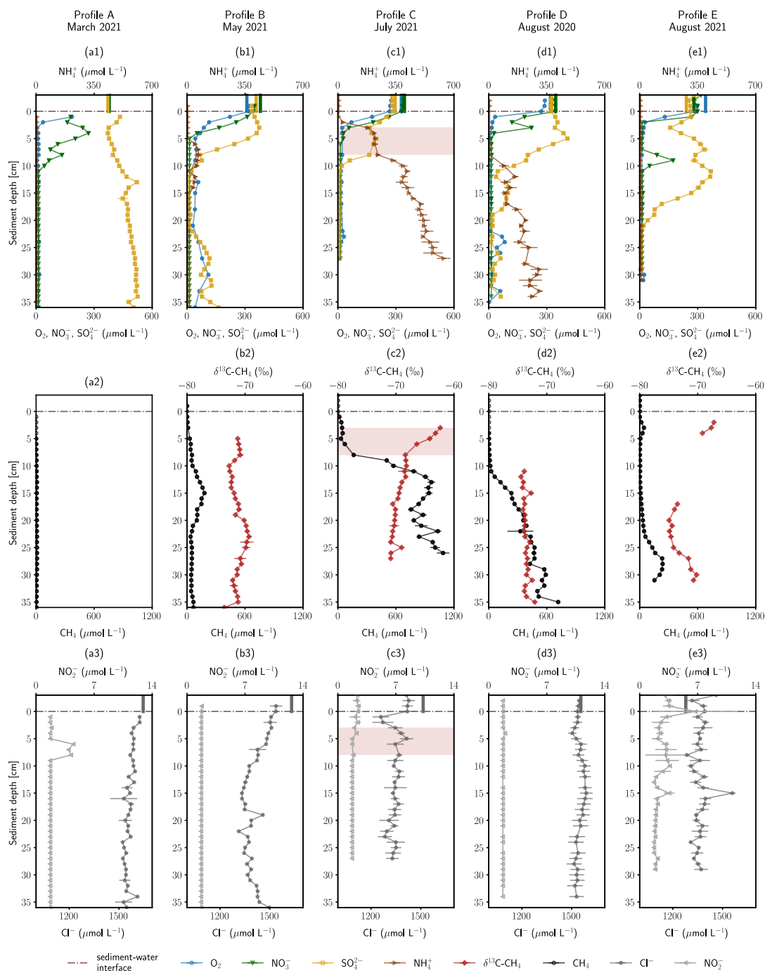
Figure 3: Depth-resolved profiles of hyporheic pore-water geochemistry at five sampling sites. Panels (a1) to (e1) show \text{O}_2 , \text{NO}_3^- , \text{NH}_4^+ and \text{SO}_4^{2-} concentrations, panels (a2) to (e2) \text{CH}_4 concentrations and \delta^{13}\text{C-CH}_4 values and panels (a3) to (e3) \text{NO}_2^- and \text{Cl}^- concentrations. Empty markers indicate values outside the range of used standards. Error bars show standard deviations of independent measurements ( n=3 ). Vertical lines above the sediment-water interface are concentrations measured in the surface water at the sampling date. Red background color highlights an enrichment in \delta^{13}\text{C-CH}_4 . Profiles are ordered by season.
