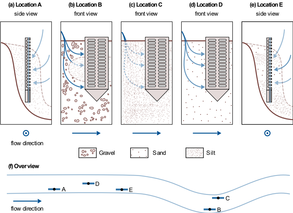
370 Figure 4: Schematic representation of potential hyporheic flow paths (blue arrows) at the five sampling sites. For locations A and E, a side view was chosen and for locations B, C and D a front view. Where the front view is shown, flow direction in the river is from left to right and where the side view is shown flow direction is out of the drawing plane. The color strength of the arrows corresponds to the expected magnitude of hyporheic fluxes. The sediment composition is schematically indicated. Quantitative data on the sediment composition at the five locations can be found in Appendix A.
