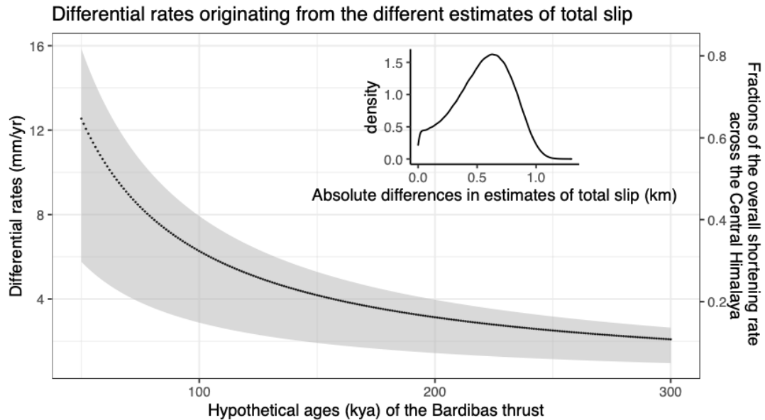
200 Figure 6: Hypothetical ages of the Bardibas thrust (horizontal axis), the corresponding fractions of the shortening rates across the Central Himalaya (right axis, overall shortening rate is \sim 19.4 mm/yr based on Stevens and Avouac, 2015), and the corresponding differential rates (left axis). These differential rates originate from the varying estimates of the total slip by Almeida et al. (2018) and this study. The black dots show the most probable values, and the grey shaded area shows the 68% confidence interval.
