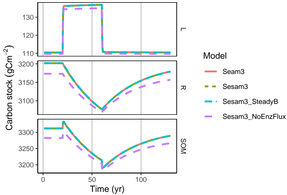
Figure 3. SOM Stocks, here approximated by the sums-sum of litter, L, and residue, R, develop in the same way with the "Increased C input" simulation with the different model version. All model variants could simulate the liberation of N from organic R stocks with the stoichiometric imbalance with increased C inputs.
