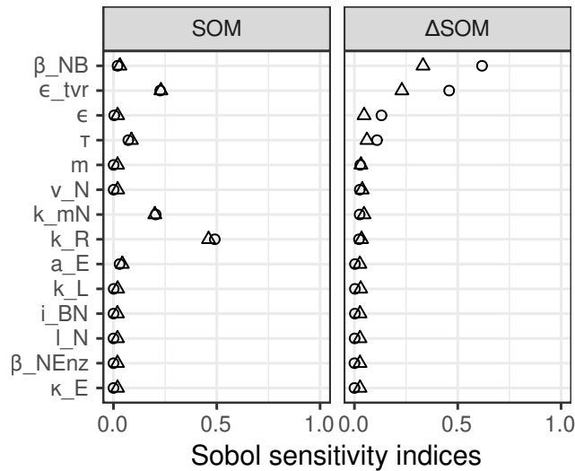
Figure 5. Simulated stock change with increased C litter input ( \Delta SOM), was most sensitive to C/N ratio of microbial biomass ( \beta_{NB} ), while initial steady state stocks (SOM) was were most sensitive to turnover rate of residue pool ( k_R ). Both were sensitive to parameters of microbial turnover. While effects on stocks were mostly direct (indicated by first order effects (triangles) were similar to total effect (circles)), the stock changes were mostly sensitive to interactions of parameters.
