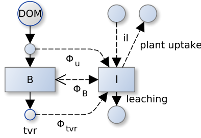
Figure A1. Several component fluxes sum to total mineralization flux in SESAM: \Phi = \Phi_u + \Phi_B + \Phi_{tvr} . A negative mineralization flux, \Phi_B corresponds to N immobilization of inorganic pool, I , by microbial biomass, B . In addition there is mineralization during microbial turnover, \Phi_{tvr} , and mineralization during uptake, \Phi_u . Fluxes across the system boundary are inputs of inorganic N, iI , inputs of organic N with litter, plant uptake of inorganic N, and leaching.
