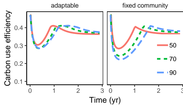
Figure 4. Variation of Carbon use efficiency (CUE) over time with the substrate pulse simulation is more conserved-dampened, i.e. is not changing as much with changing substrate stoichiometry, if microbial community adaptable can adapt enzyme allocation than with compared to fixed allocation- . This was true for both, across time (x-axis), and across initial substrate C/N ratio (line color and line type).
