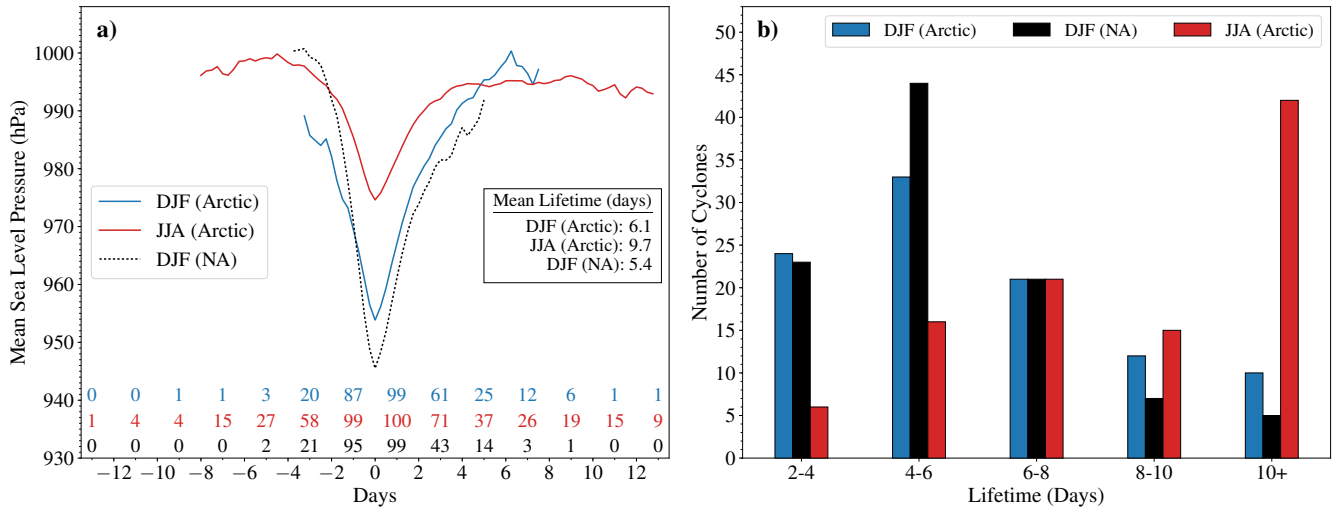
Figure 1. Life-eyes-Lifecycles of the 100 most intense winter (DJF) and summer (JJA) Arctic cyclones and winter North Atlantic (NA) Ocean extra-tropical cyclones between 1979 and 2020. a) The mean composite life-eye-le-lifecycle development in intensity (MSLP), when cyclones are centred at the time of their maximum intensity (minimum MSLP) and where at least 10 cyclones exist at each time interval. The numbers indicate how many cyclones exist at each time interval. b) The distribution in the lifetimes of the 100 most intense winter and summer Arctic cyclones and winter North Atlantic (NA) Ocean extra-tropical cyclones.
