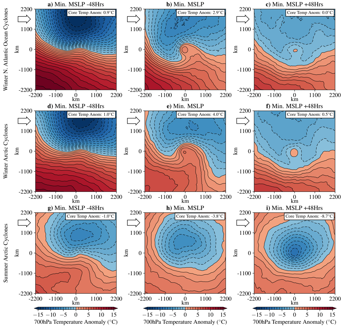
Figure 6. Horizontal 700 hPa temperature anomaly ( ^{\circ}\text{C} ) composite structure 48 hours before the time of maximum intensity (minimum MSLP) (left panel), b) at the time of maximum intensity (middle panel), and 48 hours after the time of maximum intensity (right panel), of winter (DJF) North Atlantic Ocean extra-tropical cyclones (top panel), winter Arctic cyclones (middle panel), and summer (JJA) Arctic cyclones (bottom panel). The large arrow indicates the direction of storm propagation.
