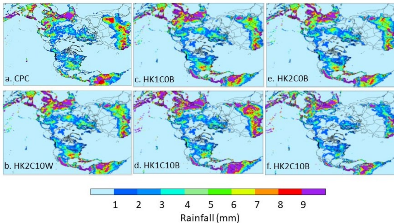
858 Figure 8. CPC rainfall (a) and simulated (b-f) mean daily precipitation during July 2016 over the 859 hemispheric domain. The LTA configuration is represented by one case (b. HK2C10W) since all 860 the LTA cases with different cumulus parameters produced similar results. All BASE cases are 861 shown here (c-f) because the cumulus parameters do impact the simulated precipitation when not 862 using LTA.
