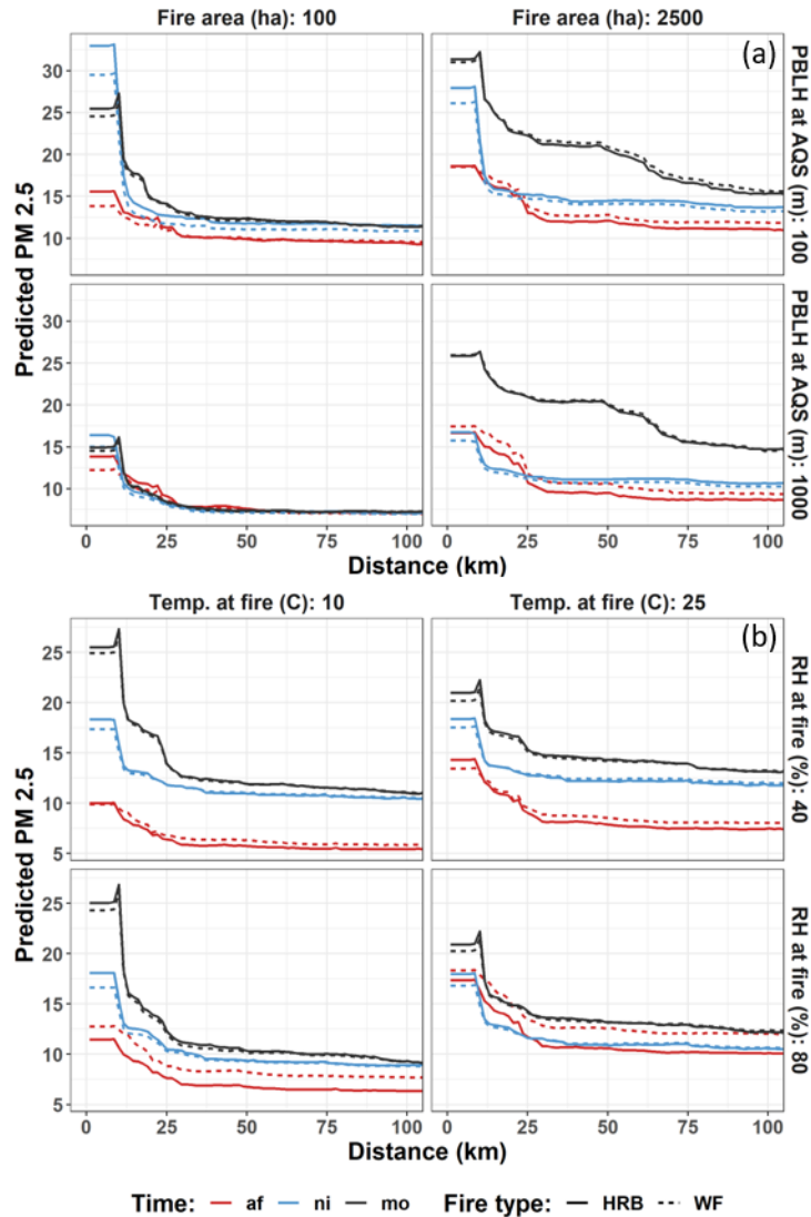
430 Figure 8: Predicted effects of selected variables on mean PM_{2.5} . Colours are time periods, line types are fire types and grid squares are combinations of the daily active fire area and planetary boundary layer height at the air quality monitoring station (a) and relative humidity and temperature at the fire (b).
