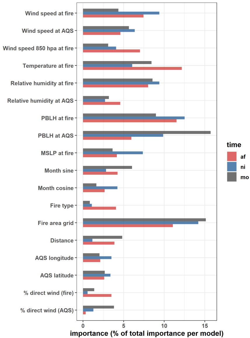
Figure 5: Variable importance for each model. A common x scale was assigned for clarity, which is the % of the total permutation importance attributable to each variable (i.e. \text{importance} / \sum(\text{importance}) * 100 ).
