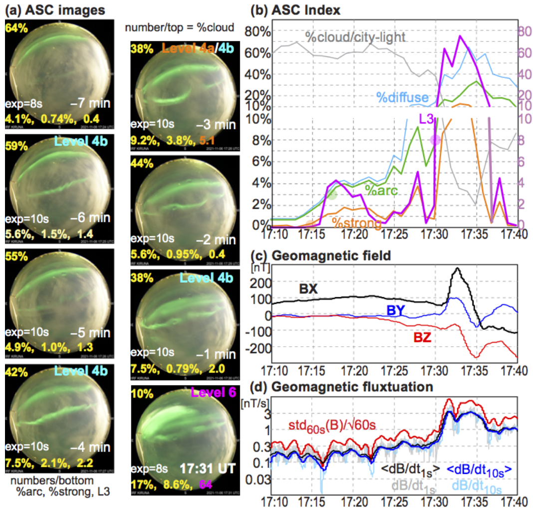
Figure 7. ASC and magnetometer data around 17:31 UT on 6 November 2021: (a) Auroral images (the same coordinate as Fig. 2); (b) ASC auroral index values; (c) DC geomagnetic deviation from the baseline values (X=north, Y=east, Z=downward); and (d) AC geomagnetic variation |dB/dt| measured by three different methods. In each image, the ASC auroral index values of %arc, %strong, and L3 are given at the bottom, above which the automatic exposure time and UT are given. The cloud coverage (%cloud) and the activity level (Level 6, Level 4a, and Level 4b) are given at the top. The timing of Level 6 detection is the same as the onset of the Local-Arc-Breaking. In the auroral index panel (b), the scaling is changed between below 10 and above 10 (therefore the graph has a gap in between). The three methods of |dB/dt| are: (1) using 1-sec values (black), (b) using 10 sec running average values (blue), respectively, and (3) standard deviation of magnetic field over 60 sec using 1-sec values and normalized to nT/s unit (red). These variations are first calculated for each vector component, and then taken the absolute values.
