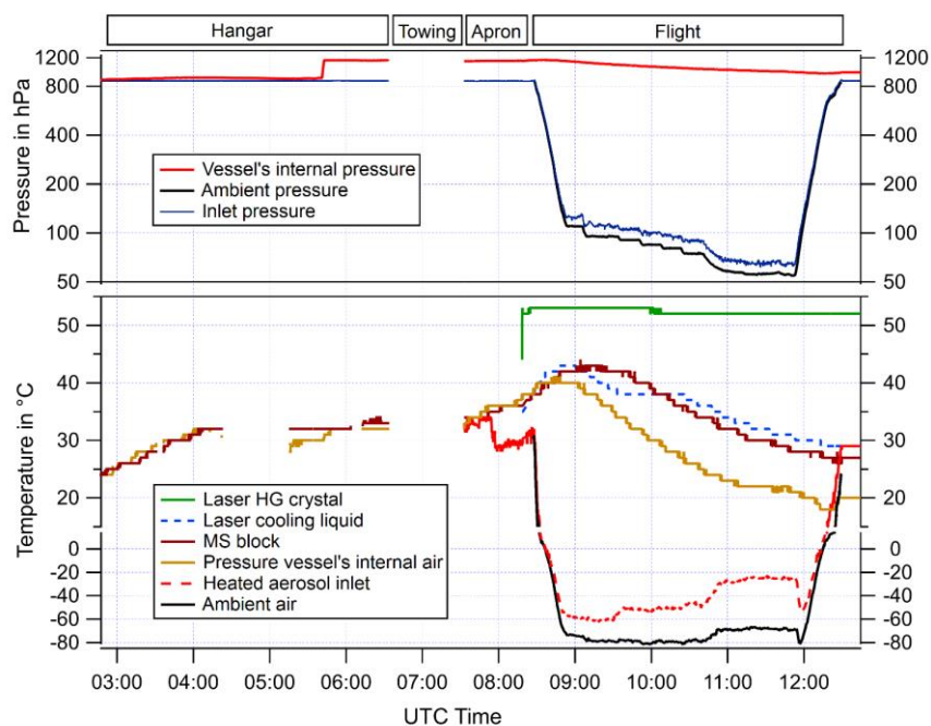
Figure 7—Temperature and pressure information during KTM 4 flight operations in Nepal on 02 August 2017. The graph includes the flight preparation time in the hangar and at the apron. The ambient pressure information is provided by the aircraft sensors via
