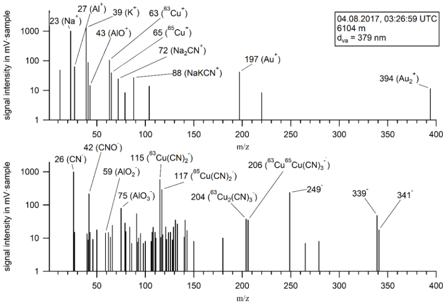
Figure 9 Bipolar spectrum from a single particle sampled at a barometric altitude of 6104 m during KTM 5 flight from Kathmandu, Nepal on 04 August 2017 indicating gold contamination. Only signals above the ion area peak threshold (7 mV-sample; Hünig et al., 2021) are shown.
