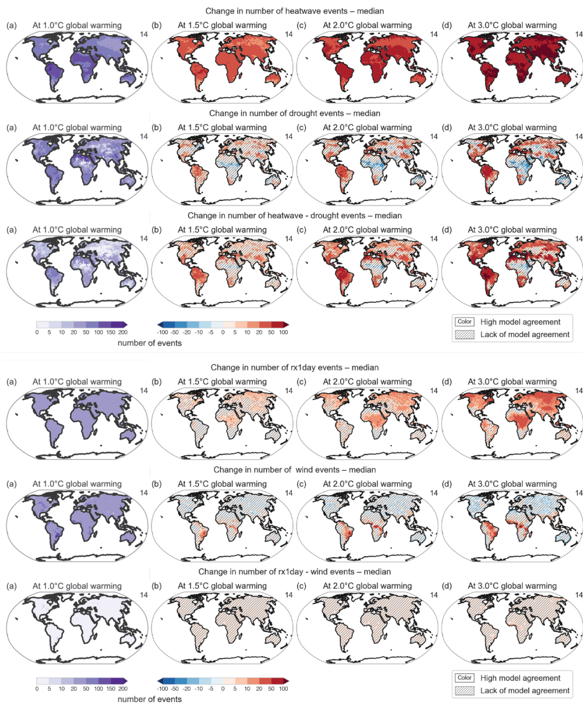
535 Figure B2. Number of individual and concurrent extremes (a) at +1°C and (b, c, d) change at +1.5°C, +2°C and +3°C with respect to +1°C. Colours refer to high model agreement and hatched areas refer to lack of model agreement.
