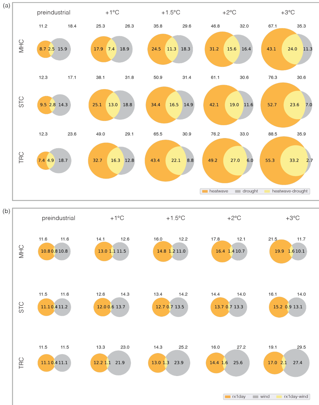
215 Figure 3. Venn diagrams of (a) heatwave-drought and (b) Rx1day-wind storm events at global warming levels. The values show the individual and concurrent frequency of events in MHC, STC and TRC in preindustrial period and at +1°C, +1.5°C, +2°C and +3°C GWLs. Areas of the circles are proportional to the frequencies [%] and represent the multi-model mean. The numbers above the Venn diagrams represent the total share of individual events including the ones occurring during concurrent events.
