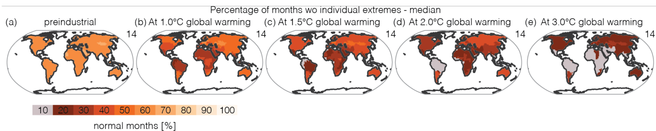
375 Figure 8. Percentage of non-event months (months without individual extremes) at warming levels (+1°C, +1.5°C, +2°C and +3°C).
