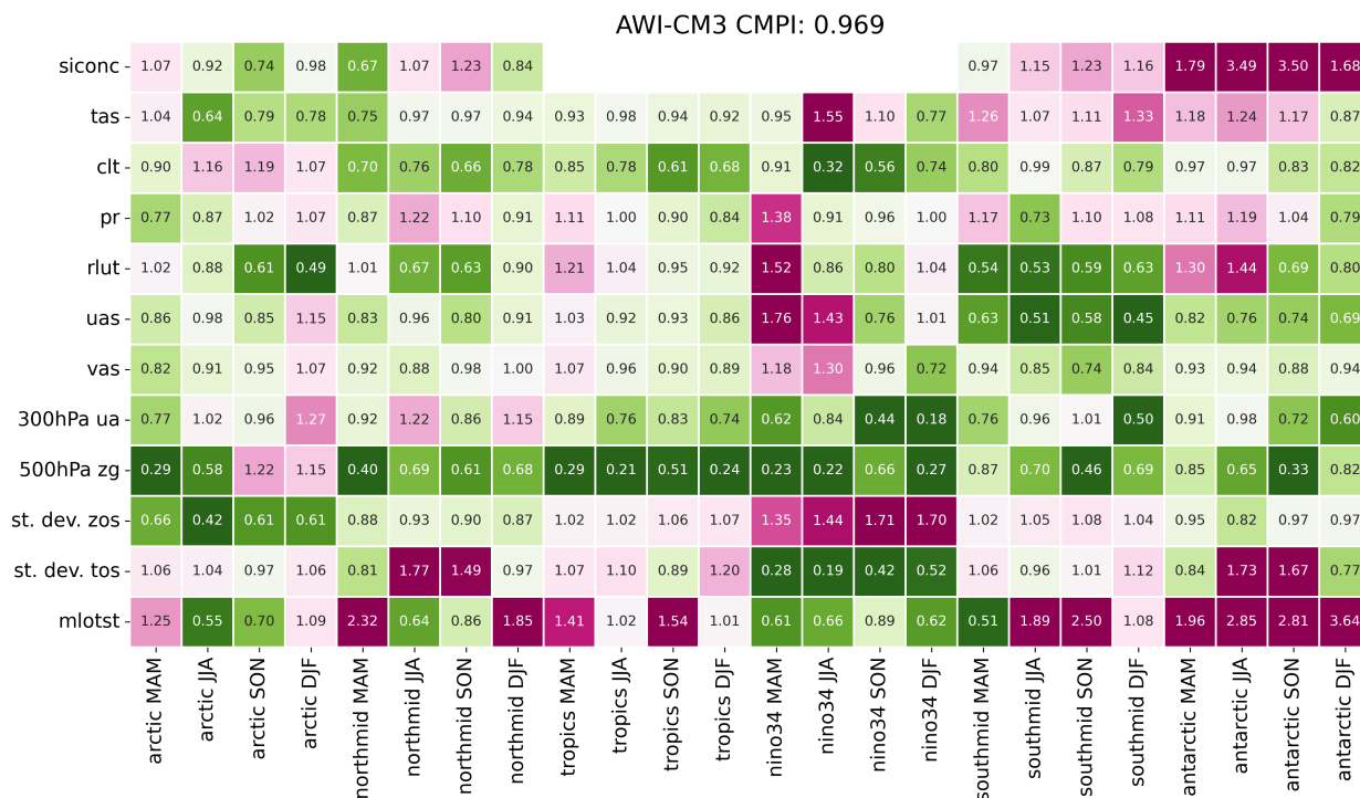
Figure B1. HIST biases as figure 4 , but using NCEP-DOE2 re-analysis by Kistler et al. (2001) instead of ERA5 for near-surface air temperature (tas), eastward near-surface wind (uas), northward near-surface wind (vas), 300 hPa eastward wind (ua), 500 hPa geopotential height. Note that ERA5 was created using IFS CY41R2, a model closely related to the OpenIFS CY43R3 atmosphere employed in AWI-CM3.
