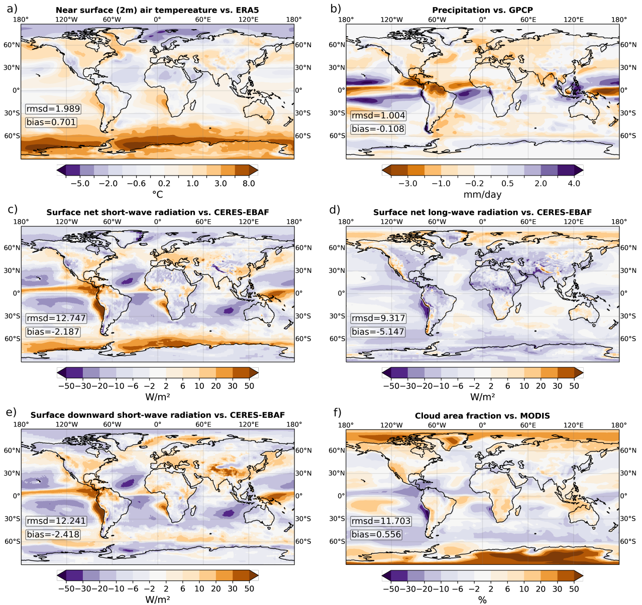
Figure 7. Annual mean a) Near surface (2m) air temperature bias with respect to ERA5. b) Precipitation bias with respect to GPCP. c) Surface net shortwave radiation bias with respect to CERES (2001-2014). d) Surface net longwave radiation bias with respect to CERES (2001-2014). e) Surface downward shortwave radiation bias with respect to CERES (2001-2014). f) Total cloud cover fraction bias with respect to MODIS. For each variable rmsd gives the area weighted root mean square distance between observations and model data, and bias gives the area weighted mean distance.
