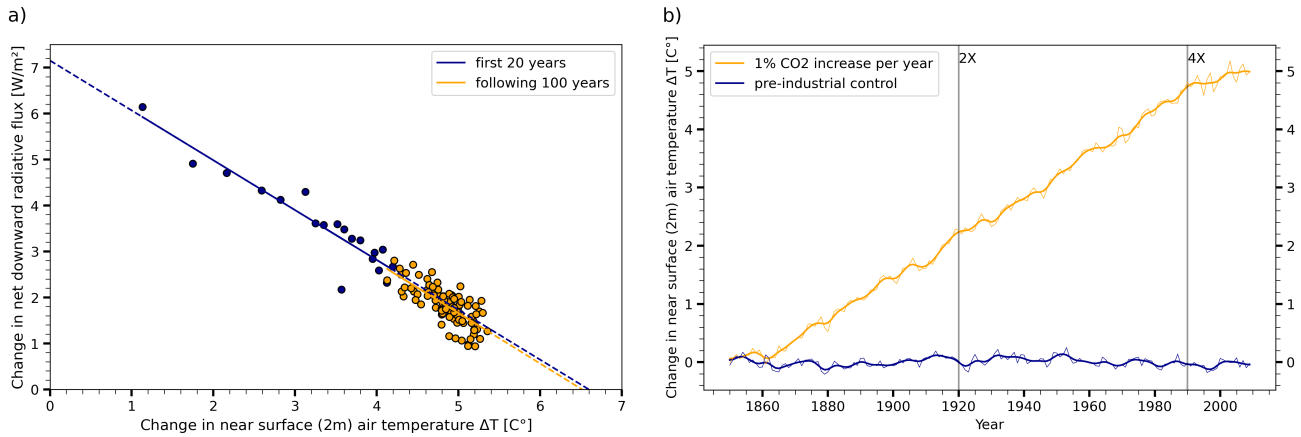
Figure 14. a) Gregory regression plot from the abrupt 4xCO 2 experiment in comparison to the pre-industrial control. We construct the linear regression of near surface (2m) air temperature ( \Delta T ) change against the downward net radiative flux change ( \Delta F ). From its axis intersection points we obtain the radiative forcing \Delta F = 7.06 \frac{W}{m^2} , and the Equilibrium temperature difference \Delta T = 6.49^\circ C . The climate response parameter of AWI-CM3 is then \alpha = \frac{\Delta T}{\Delta F} = 0.92 \frac{K}{W} and the Equilibrium Climate Sensitivity ECS = \frac{\Delta T}{2} = 3.24^\circ C . The first 20 years already result in a linear regression almost identical to the following 100 years. b) As Figure 11 b), but for the experiment with 1% increase of CO 2 per year. Vertical lines indicate doubling and quadrupling of CO 2 concentrations. The estimated Transient Climate Response is 2.1°C.
