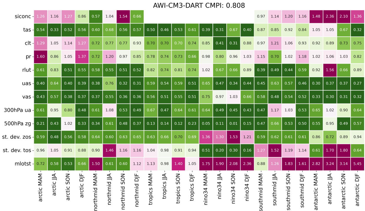
Figure 15. Same as figure 4 but for the last 10 years of a 50-year-long TCo319L137-DART simulation under constant 1990 forcing. Biases to observations are not only smaller than in our TCo159L91-CORE2 simulations, but also smaller than those of all but two (HadGEM3MM & NOAA-GFDL) of the CMIP6 models listed in A (Performance indices for CMIP6 models not shown).
