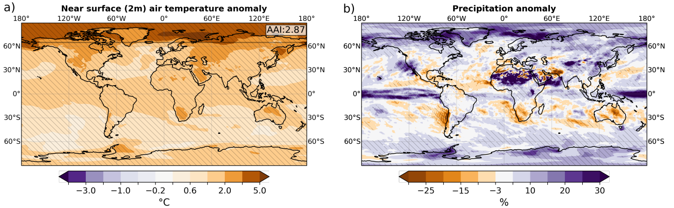
Figure 12. a) Temperature anomaly between last 25 years of the historic simulations and the equivalent period of the pre-industrial control run. The Arctic Amplification index, defined as the ratio of warming north of 65°N expressed as a fraction of global warming, is 2.87. Significant temperature anomalies are hatched and the 95% significance is obtained via bootstrap test. b) Same as a) but for relative precipitation changes.
