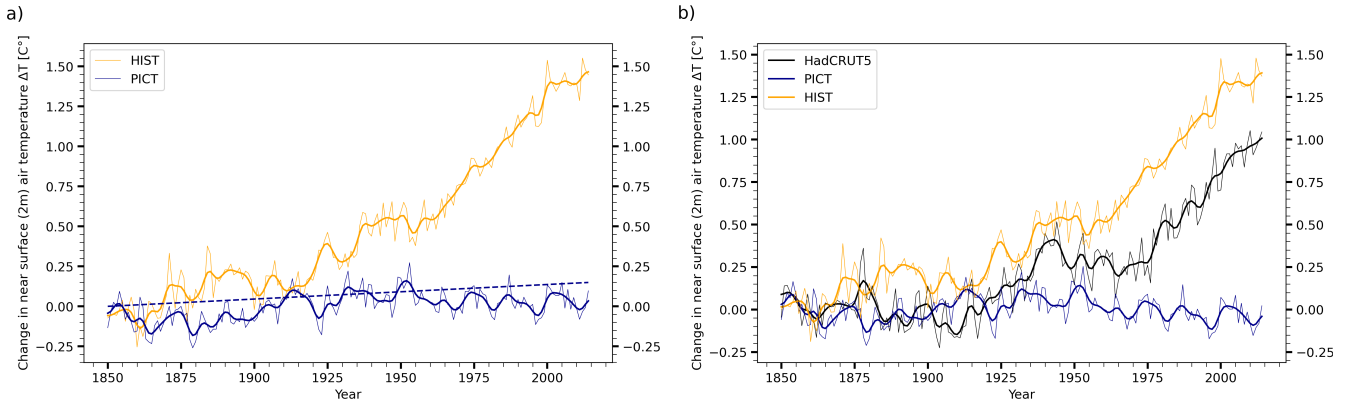
Figure 11. a) Near surface (2m) air temperature changes over the historic period and in the pre-industrial control simulation. Thick lines show the 10 year running means. The pre-industrial control simulation shows a residual drift of 0.00091 \frac{^{\circ}\text{C}}{\text{Year}} obtained from linear regression. b) Both simulations have been corrected by subtracting the residual drift. The resulting simulated global warming over the period 1850 to 2014 is 1.4^{\circ}\text{C} . In comparison to observational estimates from HadCRUT5 (Morice et al., 2021) warming is overestimated by 0.4 K, likely due to fixed aerosols in the AWI-CM3 prototype.
