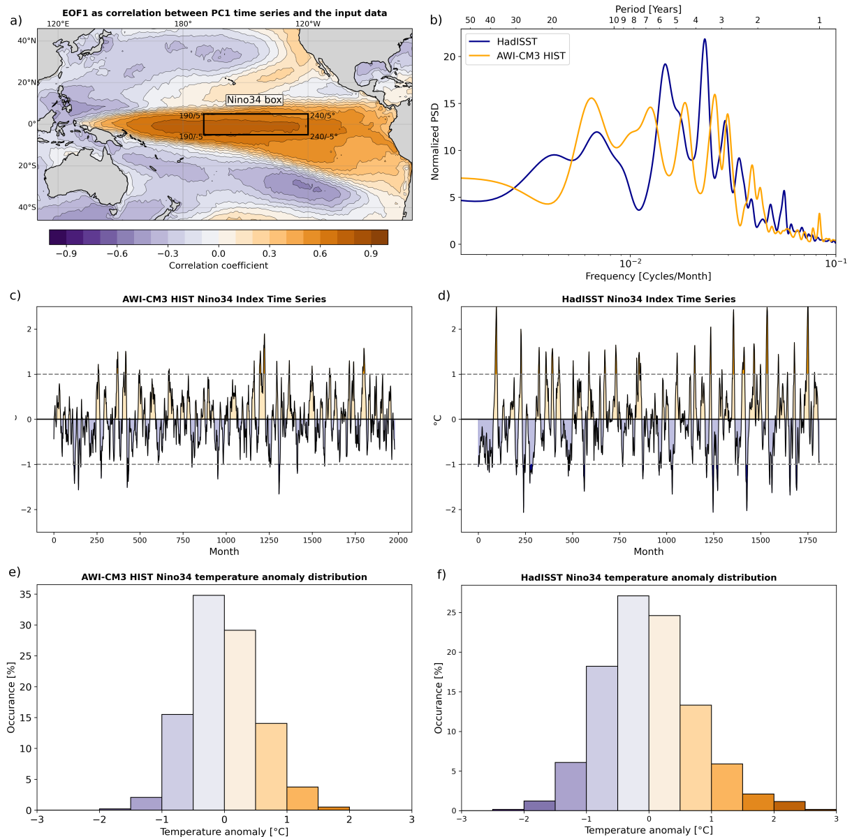
Figure 10. a) Extent of the Nino3.4 box, as well as the first empirical orthogonal function expressed as the correlation between the first principle component and the input data set at each point in space. Calculated from the entire HIST simulation using the EOFs toolbox (Dawson, 2016). b) Normalized power spectrum density of simulated ENSO within the Nino3.4 box in comparison to HadISST observational estimates for the years 1850 to 2014. c) & d) Nino3.4 SST index defined as the detrended, seasonal cycle removed and 3-months running mean timeseries of SST averaged over the Nino3.4 box. The results from AWI-CM3 HIST and HadISST observational estimates are shown, respectively. e) & f) As c) & d) but depicting occurrence of temperature anomalies in bins with a width of 0.5°C.
