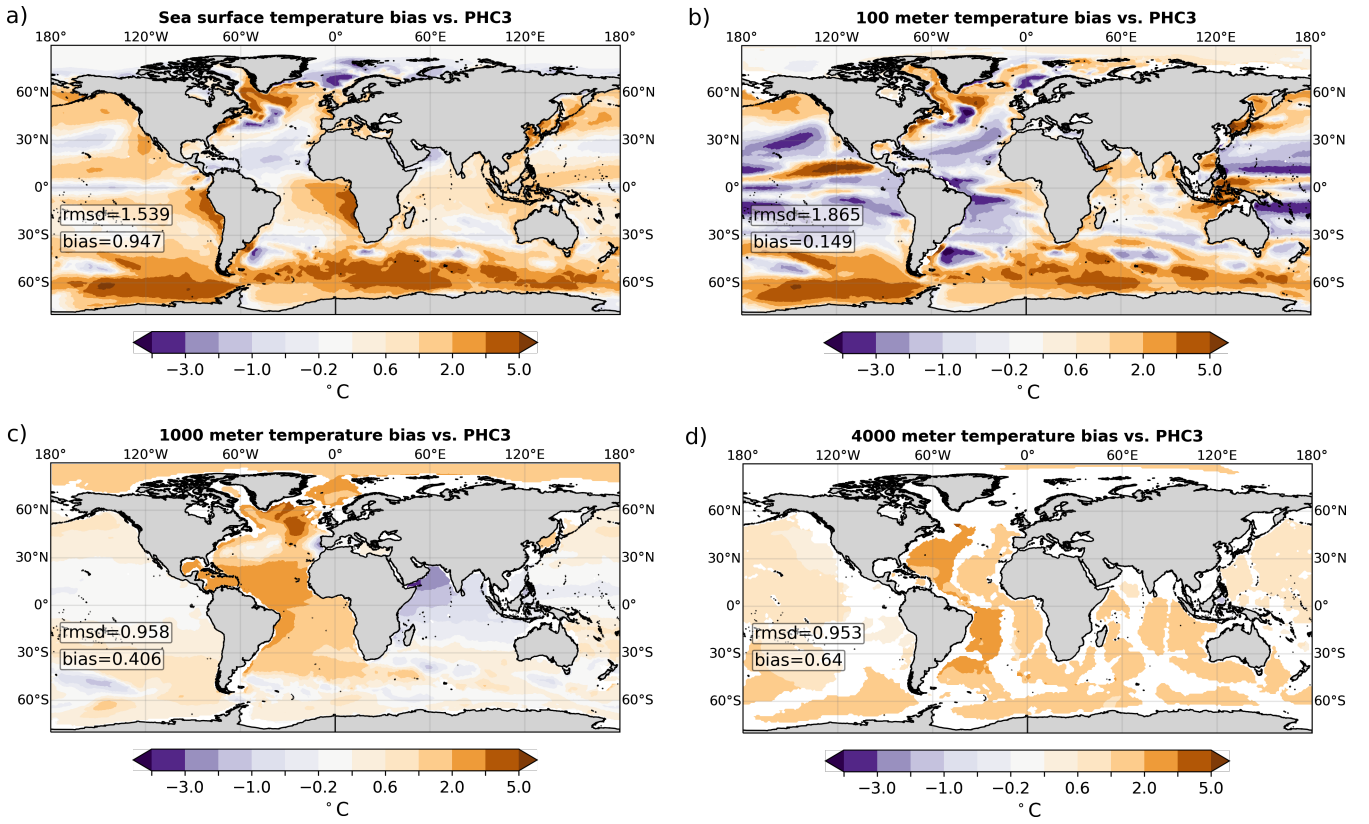
Figure 9. Mean ocean temperature bias of the last 25 years of the historical simulation with respect to PHC3 at a) 0, b) 100, c) 1000 and d) 4000 meters depth. For each depth rmsd gives the area weighted root mean square distance between observations and model data, and bias gives the area weighted mean distance. At the surface the ocean-resolution-specific warm biases in upwelling regions and western boundary currents can be seen, in addition to a pronounced Southern Ocean warm bias. At depth, a warm bias is dominating in the Atlantic.
