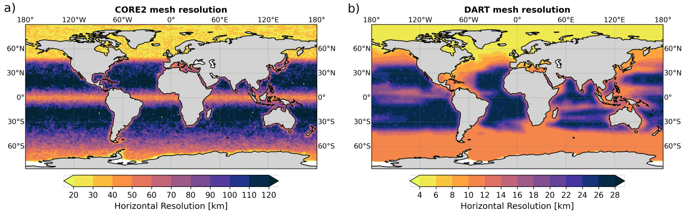
Figure 2. a) Horizontal resolution of the CORE2 mesh used for the main simulations presented in this work. b) As a) but for the DART mesh with higher resolution, which is based on a mix of local Rossby radius of deformation and local sea surface height variability. The DART mesh is used in Section 5.1 for an outlook of high resolution applications.
