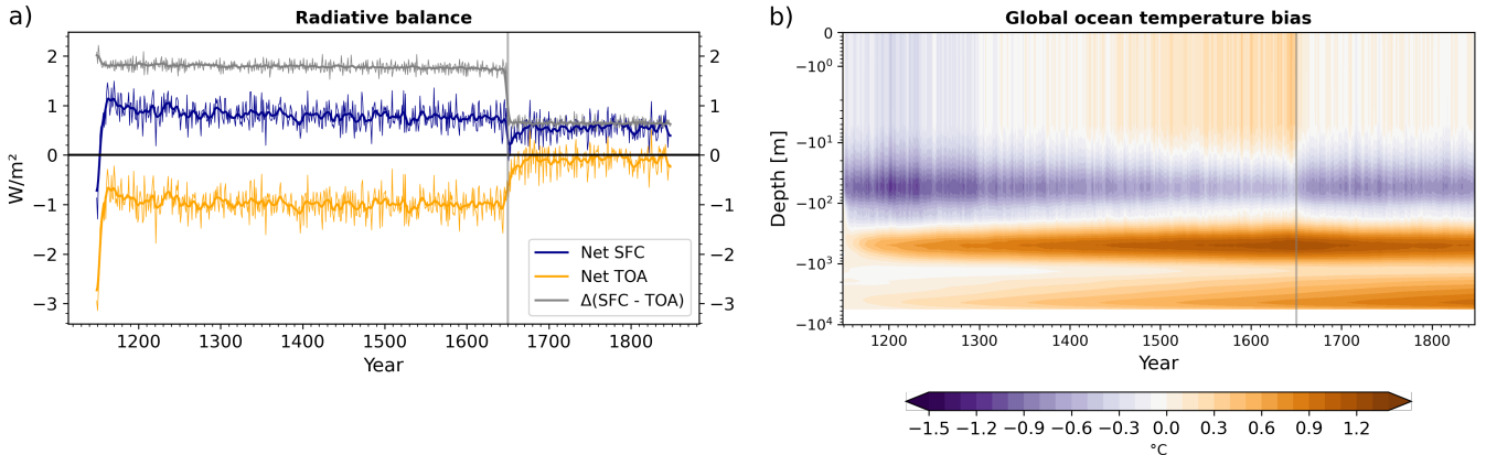
Figure 3. a) Net radiative imbalance at the top of atmosphere (TOA) and at the surface (SFC) in the spinup simulation. Positive (negative) values indicate downwards (upwards) net heat flux. The difference results from spurious energy production in the atmosphere. b) Semi-logarithmic depth Hovmöller diagram of the evolution of the global mean ocean temperature bias over the spinup period with respect to PHC3 climatological values (Steele et al., 2001). Switching from dry to total mass fixer after 500 years reduced spurious heat production in the atmosphere and halted the ocean warming trend in the upper 1000 meters. Warming at depth continued.
