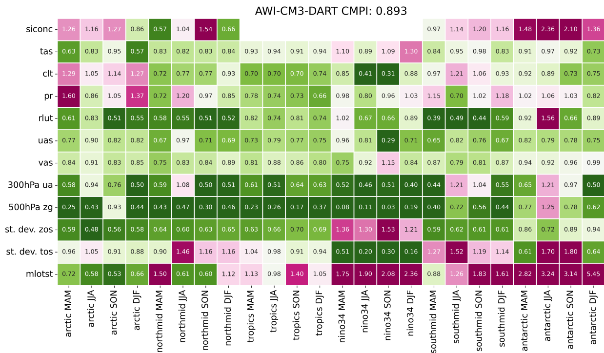
Figure B2. TCo319L137-DART biases as figure 15, but using NCEP-DOE2 re-analysis by Kistler et al. (2001) instead of ERA5 for near-surface air temperature (tas), eastward near-surface wind (uas), northward near-surface wind (vas), 300 hPa eastward wind (ua), 500 hPa geopotential height. Note that ERA5 was created using IFS CY41R2, a model closely related to the OpenIFS CY43R3 atmosphere employed in AWI-CM3.
