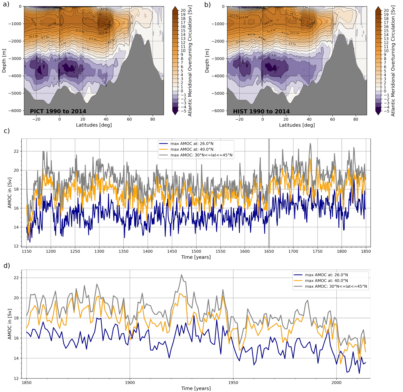
Figure 13. a) Atlantic Meridional Overturning Circulation (AMOC) streamfunction averaged over the last 25 years in the pre-industrial control (PICT) simulation. b) as a) but for the historic (HIST) simulation. c) Evolution of the AMOC maximum at different latitudes throughout the spinup simulation (SPIN) that precedes both PICT and HIST. d) Evolution of the AMOC during HIST.
