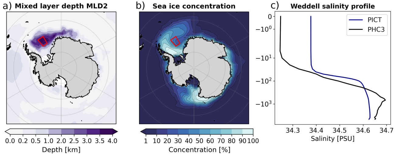
Figure 6. a) Austral winter mean mixed layer depth (MLD) where the potential density over depth differs by 0.125 \frac{kg}{m^3} from the surface density (Monterey and Levitus, 1997) averaged over the last 25 years of the PICT simulation. b) High MLD values in the Weddell and Ross seas contribute to the persistent polynyas visible in the mean austral winter sea ice concentration over the same time period. c) Salinity profile over the region marked in red in comparison to PHC3 climatology (Steele et al., 2001).
