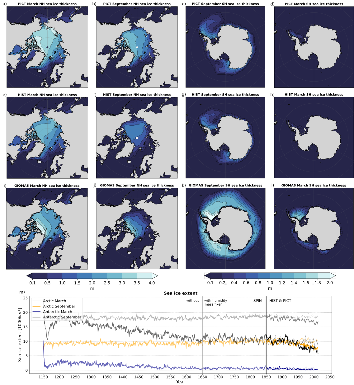
Figure 5. a-d) Mean sea ice volume per unit area over last 25 years of PICT simulation. e-h): Same as top row but for the HIST simulation. i-l): Same as top row but for GIOMAS sea ice thickness reanalysis product. (Zhang and Rothrock, 2003). m): Evolution of sea ice extent over SPIN, as well as HIST and PICT simulations. Mass fixer switched from dry to total in years 1650. HIST and PICT forcing applied from 1850 onwards.
