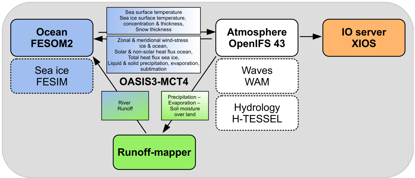
Figure 1. Schematic of the coupling between AWI-CM3 model components. Two hourly parallel communication in AWI-CM3 is implemented via the OASIS3-MCT 4.0 library. Heat, mass and momentum fluxes are sent from OpenIFS to FESOM2, while ocean and ice surface state variables are sent back. The precipitation minus evaporation over land is handled with a runoff mapper that generates river runoff at basin discharge points. OpenIFS output is written in parallel with optional online postprocessing via XIOS.
