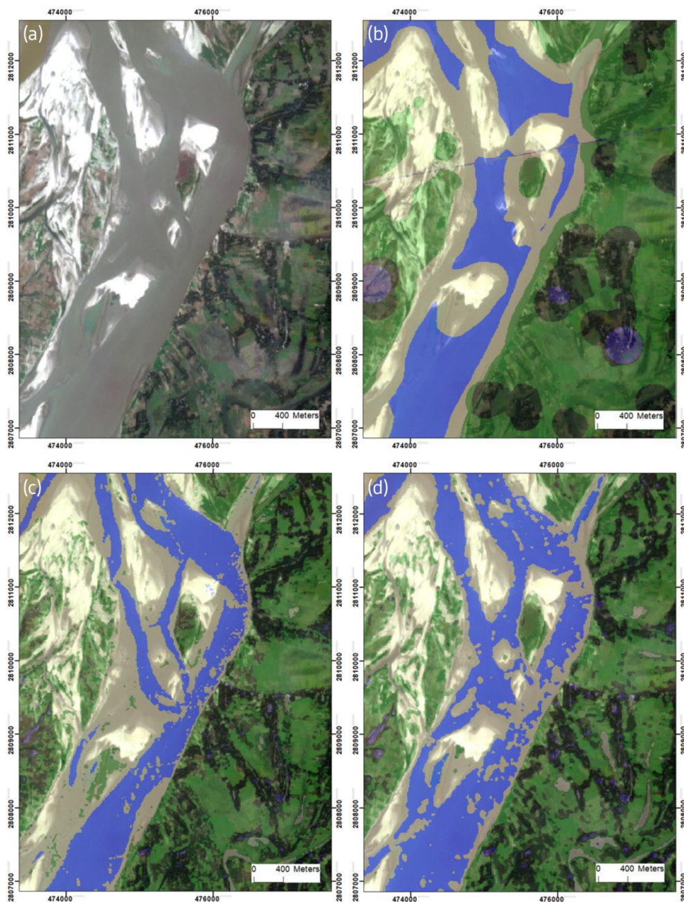
295 Figure 6: (a) Sentinel-2 image of a stretch of the eastern riverbank of Jamuna River, taken in November 2019. Image dimensions: ca. 4.5x6 km. (b), (c) and (d) Classification result for a sampling duration of two weeks/25x25 boxcar filter, six months/no filter and one month/3x3 boxcar filter, respectively. Blue – water, sand – sand, light green – fields, dark green – trees. Source of optical background image: Sentinel-2. The location of the patch is shown in Fig. A1 (patch 1). Coordinates in this and all other maps are in “Gulshan 303 Bangladesh TM” (EPSG 3106).
