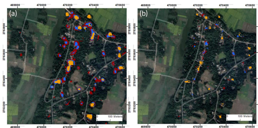
325 Figure 7: Influence of classification thresholds on settlement detection. Shown are dispersion index thresholds of 0.4 (panel (a)) and 0.25 (panel (b)) – the lower the threshold, the more stable a pixel has to be for it to be classified as a PS candidate. Colors correspond to different values of the amplitude threshold: -4 dB (red), -2 dB (blue), 0 dB (orange) – the lower the threshold,
