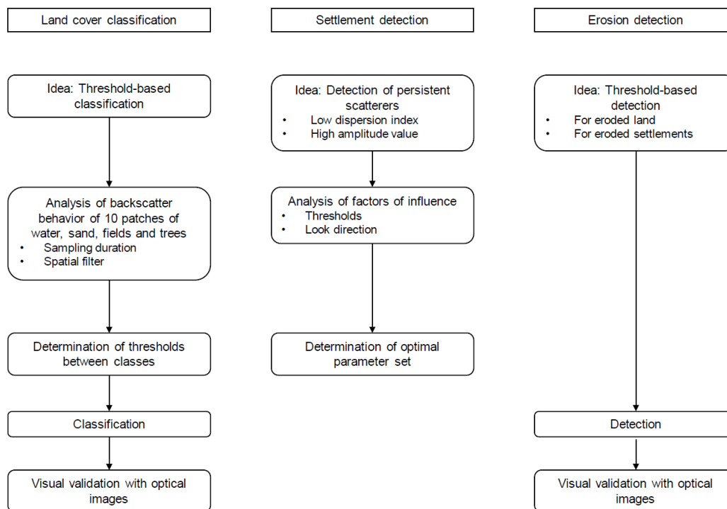
Figure 1: Overview of the analytical strategy to develop an algorithm detecting eroded land and settlement.
