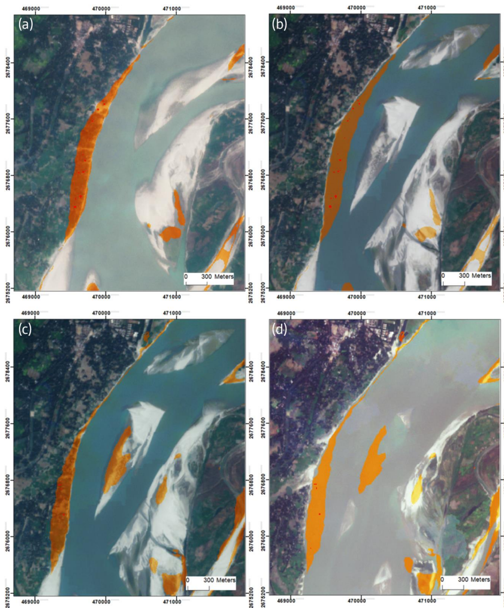
Figure 8: Validation of erosion detection. Shown are eroded land (orange) and eroded settlements (red) for 2018 ((a) and (b)) and 2019 ((c) and (d)). Baseline: optical Sentinel-2 images from before ((a) and (c)) and after the monsoon ((b) and (d)). The location of the patch is shown in Fig. A1 (patch 3).
