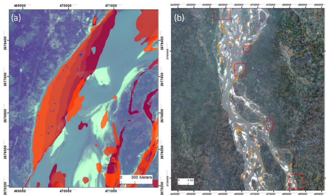
360 Figure 9: (a) Detected erosion for the monsoon seasons 2015 (dark red) to 2019 (light red). Blue: eroded settlements. (b) Locations of land eroded during the 2019 monsoon (orange). The red rectangles are the locations for which CEGIS (2018) predicted severe erosion. Source of optical background images: Sentinel-2.
