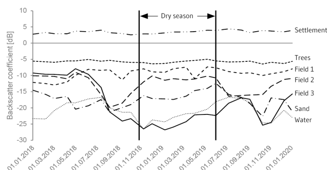
235 Figure 3: Mean monthly backscatter of different land cover types (one patch per type; the location of the patches is shown in Fig. A1) between January 2018 and February 2020, obtained from C-band of Sentinel-1. Per month, between one and six images are averaged.
