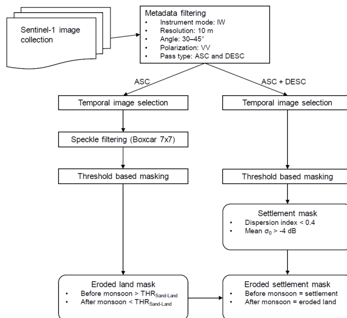
200 Figure 2: Flow chart of the final implementation to detect eroded land and settlement. THR = threshold.
