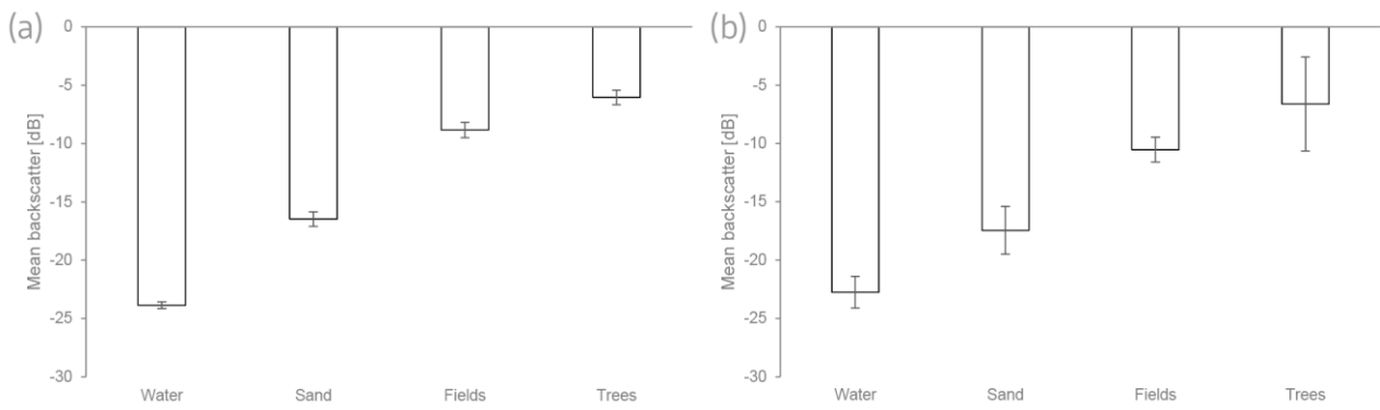
470 Figure A4: Average backscatter for four land cover classes (a) for a sampling duration of 0.5 months and a 25x25 boxcar filter and (b) for a sampling duration of 7 months and no filter. Bars indicate the mean \pm 2 standard deviations. If images are available only from two weeks, strong spatial filtering (25x25 pixels) reduces the standard deviation enough to separate all four classes even at the level of two standard deviations around the mean (panel (a)). If, by contrast, images are available from seven 475 months, water, sand and fields can be separated even if no spatial filter is applied (panel (b)). In this setting, fields and trees can be distinguished only at the level of one standard deviation around the mean (not shown in the graph).
