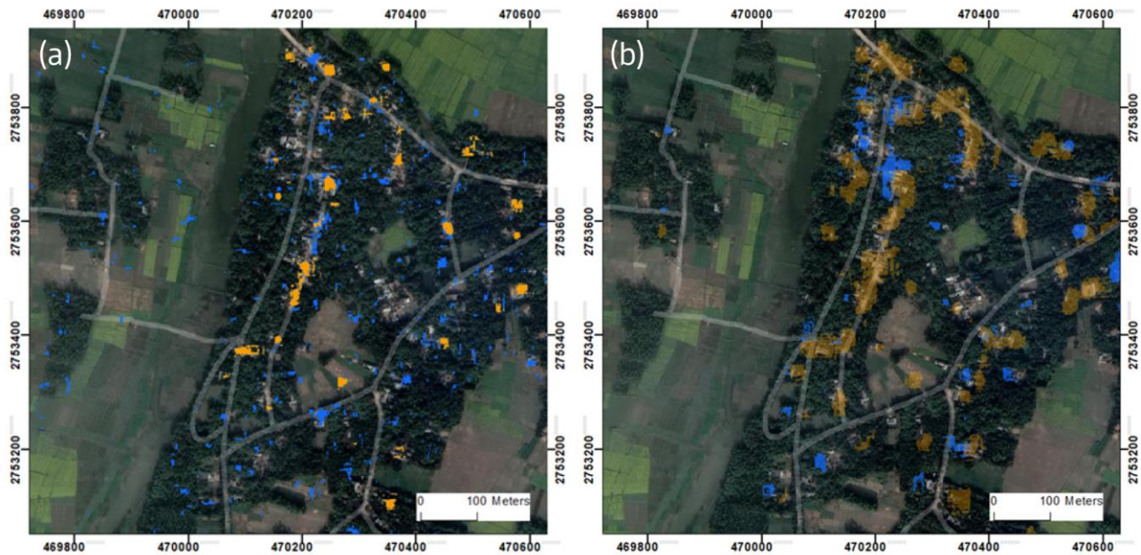
480 Figure A5: (a) Classification of settlements using the dispersion index only (blue) or the combination of dispersion index and amplitude threshold (orange). Thresholds: 0.25 (dispersion index), -2 dB (amplitude). (b) Settlement detection for ascending (orange) and descending (blue) orbit. Thresholds: 0.4 (dispersion index), -4 dB (amplitude). Sampling duration for both panels: six months. The location of the patch is shown in Fig. A1 (patch 2). Source of optical background image: Google, ©2020 Maxar Technologies, CNES/Airbus.
