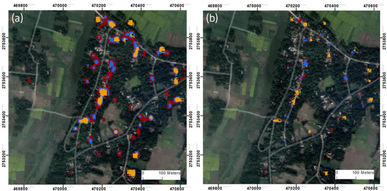
Figure 7: Influence of classification thresholds on settlement detection. Shown are dispersion index thresholds of 0.4 (panel (a)) and 0.25 (panel (b)) – the lower the threshold, the more stable a pixel has to be for it to be classified as a PS candidate. Colors correspond to different values of the amplitude threshold: -4 dB (red), -2 dB (blue), 0 dB (orange) – the lower the threshold,
