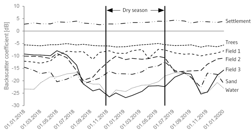
Figure 3: Mean monthly backscatter of different land cover types (one patch per type; the location of the patches is shown in Fig. A1) between January 2018 and February 2020, obtained from C-band of Sentinel-1. Per month, between one and six images are averaged.
