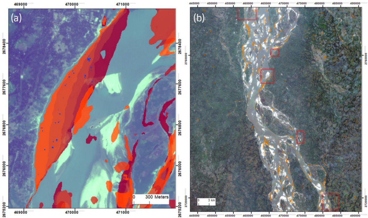
370 Figure 9: (a) Detected erosion for the monsoon seasons 2015 (dark red) to 2019 (light red). Blue: eroded settlements. (b) Locations of land eroded during the 2019 monsoon (orange). The red rectangles are the locations for which CEGIS (2018) predicted severe erosion. Source of optical background images: Sentinel-2.
