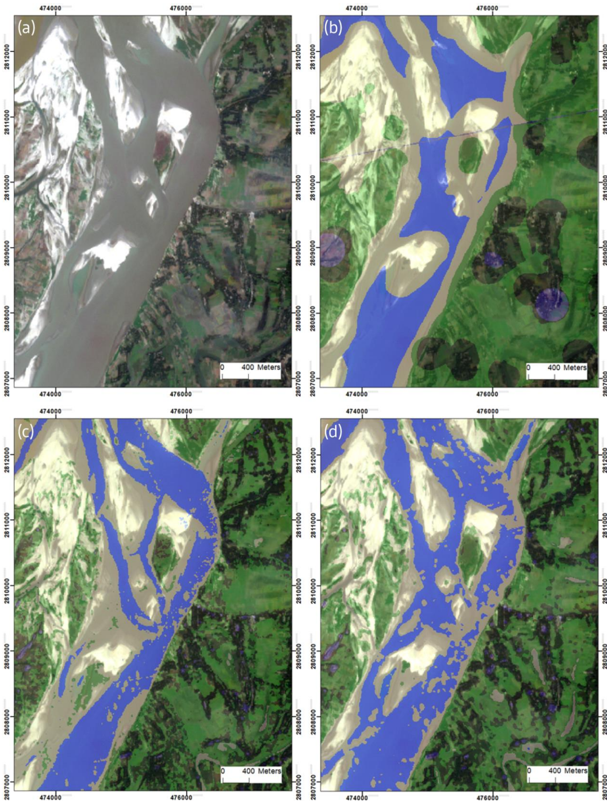
305 Figure 6: (a) Sentinel-2 image of a stretch of the eastern riverbank of Jamuna River, taken in November 2019. Image dimensions: ca. 4.5x6 km. (b), (c) and (d) Classification result for a sampling duration of two weeks/25x25 boxcar filter, six months/no filter and one month/3x3 boxcar filter, respectively. Blue – water, sand – sand, light green – fields, dark green – trees. Source of optical background image: Sentinel-2. The location of the patch is shown in Fig. A1 (patch 1). Coordinates in this and all other maps are in “Gulshan 303 Bangladesh TM” (EPSG 3106).
