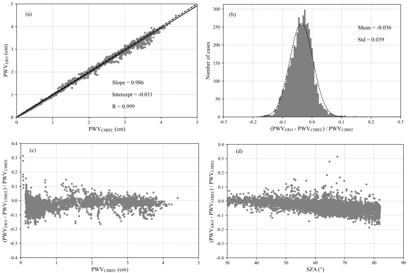
235 Figure 10. PWV retrievals from EKO using the spectral approach in the 880–1000 nm region compared to the synchronous data of CE-318 in the measuring period (a), histogram of relative difference among PWV EKO and PWV CIMEL (b), and the relative difference plotted against PWV CIMEL (c) and solar zenith angle (d).
