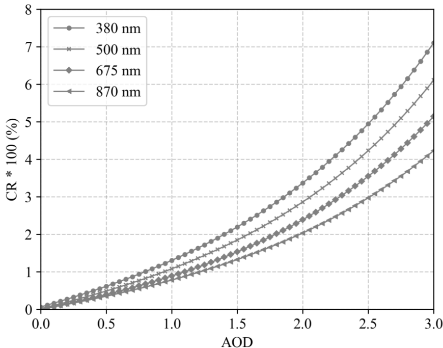
195 Figure 7. Simulations of CR * 100 (%) for SZA 30^\circ with AOD values from 0 to 3, at 380 nm, 500 nm, 675 nm, and 870 nm, for 2020 annual average MERRA2 aerosols data in the Beijing area with FOV between 1.2^\circ and 5^\circ .
