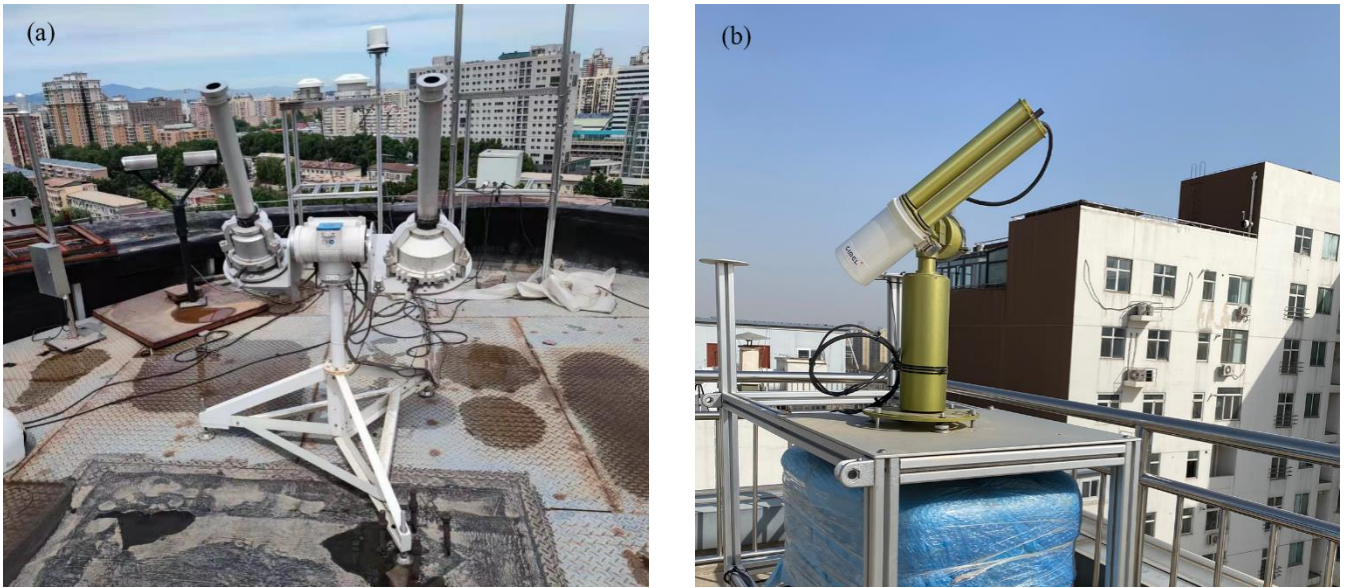
Figure 1. The EKO spectroradiometers (a) and CE-318 sun photometer (b) are collocated at the top of IAP’s building.
