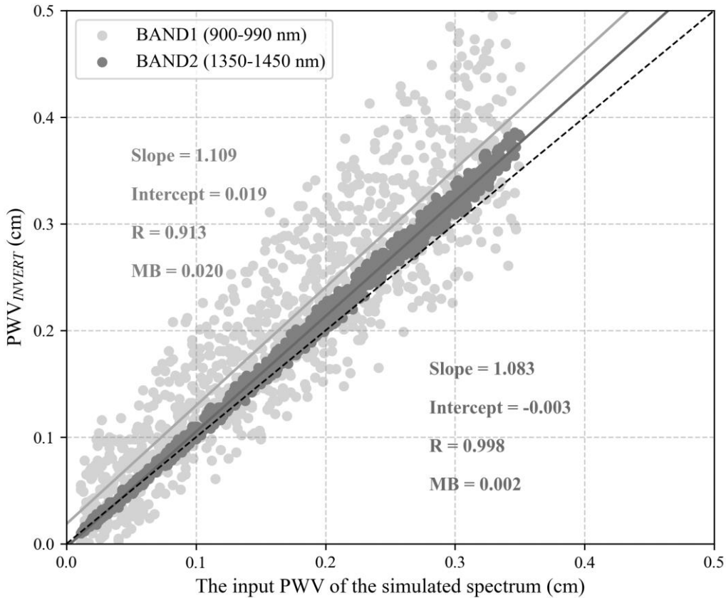
160 Figure 5. Scatter plot of the PWV retrievals obtained from BAND1 and BAND2 of the test spectrum versus the input PWV of the simulated spectrum and their linear fits.
