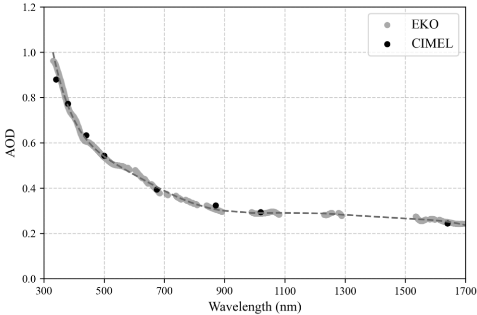
260 Figure 12. The AOD was retrieved from EKO and CE-318 on 06 June 2020 (15:22 UTC+8), the dashed line is the spectral AOD obtained by the AOD_{EKO} high-order fitting.
