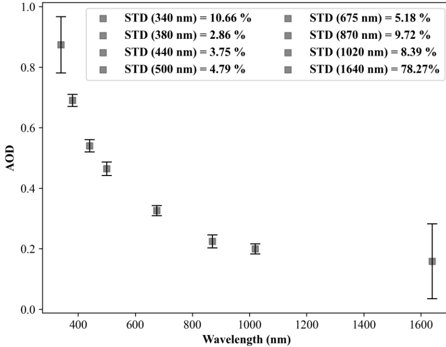
Figure 8. Mean and error bars of AOD at the wavelengths corresponding to the CE-318 filters obtained using the method described in Section 3.3 for the spectral curves after overlaying the calibration uncertainties.
