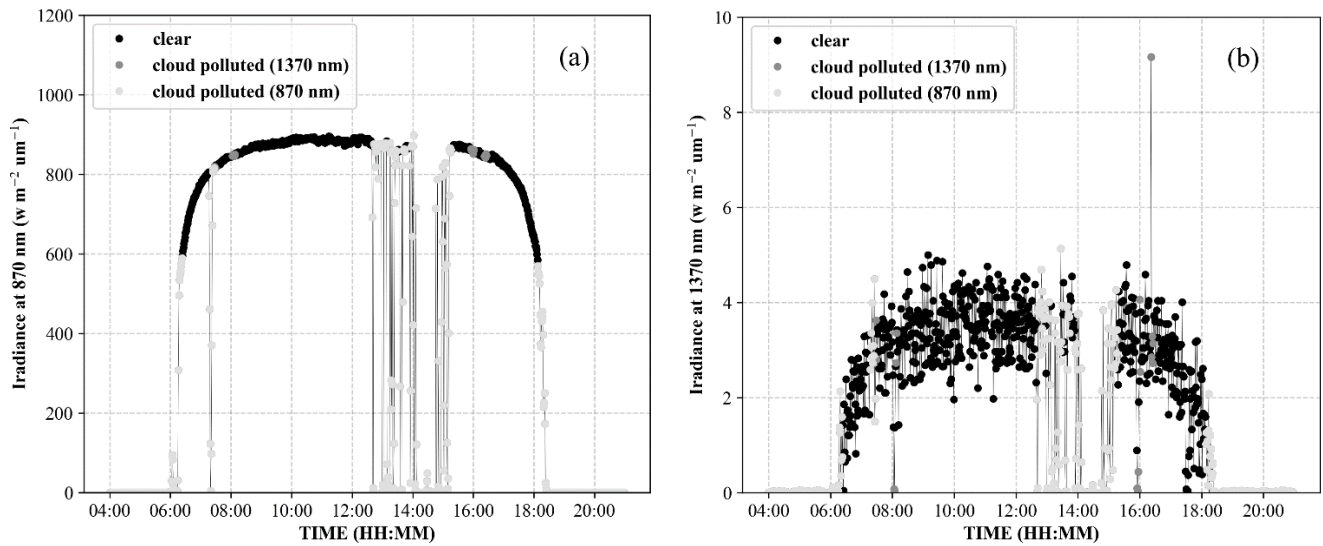
95 Figure 2. Direct normal irradiances measurements of EKO instruments at 870 nm (a) and 1370 nm (b) on 8 September 2020 at IAP. Cloudy parts and very small measurements are shown in grey, with light grey and dark grey filtered out using 870nm and 1370nm measurements respectively, and clear-sky parts shown in black.
