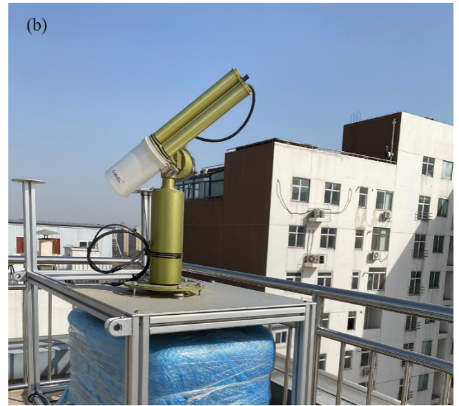
80 Figure 1. The EKO spectroradiometers (a) and CE-318 photometer (b) are collocated at the top of IAP's building.
