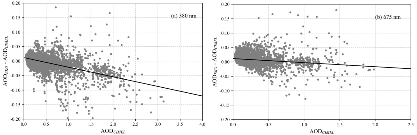
Figure 13. The Bias between synchronous AOD_{EKO} and AOD_{CIMEL} against AOD_{CIMEL} at 380 nm (a) and 675 nm (b).
