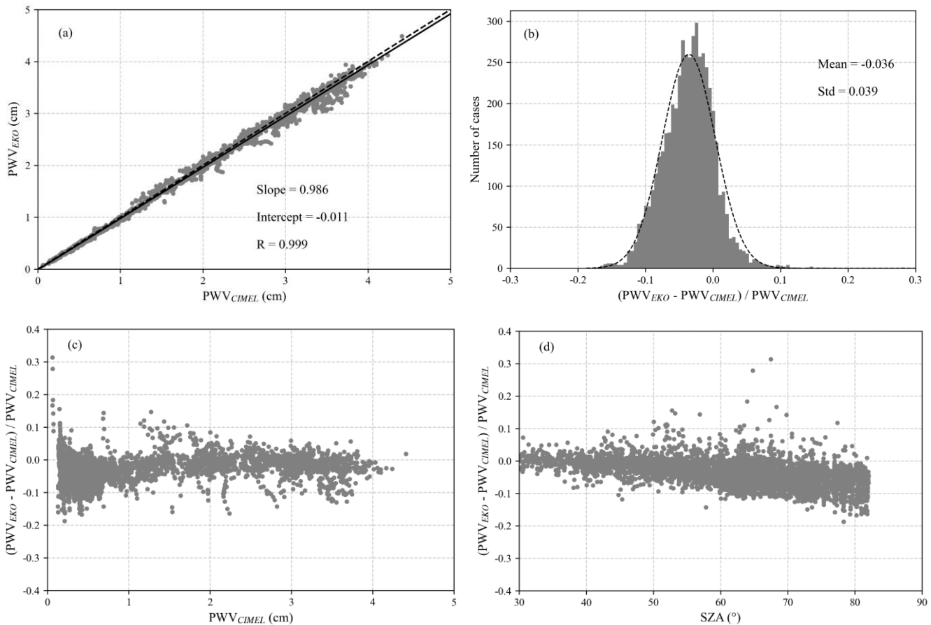
Figure 9. PWV retrievals from EKO using the spectral approach in the 880–1000 nm region compared to the synchronous data of CE-318 in the measuring period (a), histogram of relative difference among PWV_{EKO} and PWV_{CIMEL} (b), and the relative difference plotted against PWV_{CIMEL} (c) and solar zenith angle (d).
