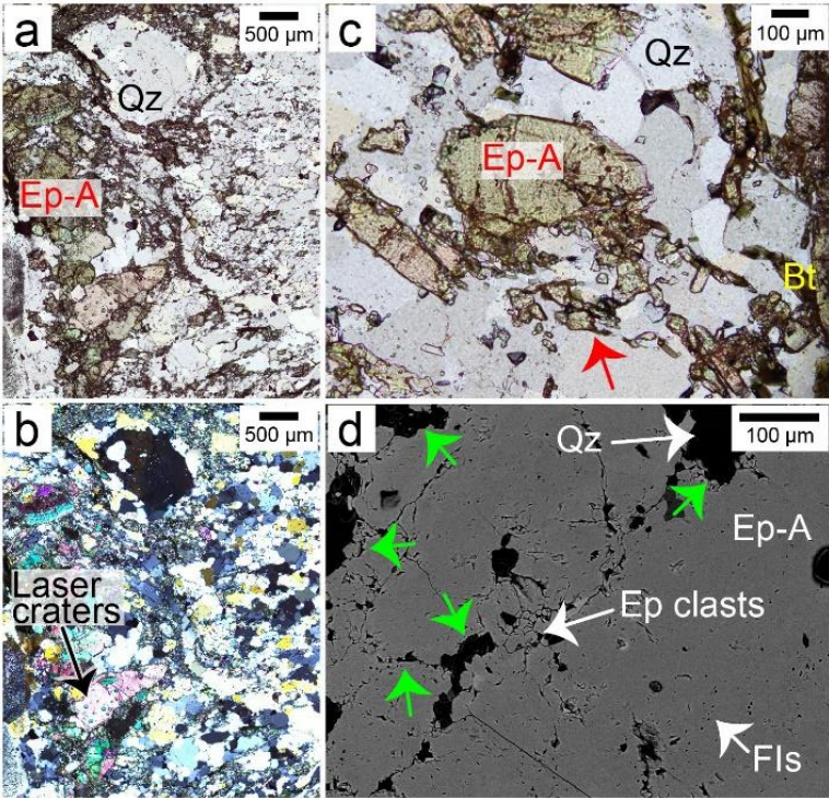
Figure 3: Details of epidote in layer 1. (a–b) Transmitted light microphotographs of epidote and quartz in plane-polarized (a) and cross-polarized (b) light. (c) One isolated epidote grain surrounded by epidote clasts (red arrow). (d) Backscattered electron image of one epidote grain showing lobate grain boundaries and microporosity suggested by the presence of fluid inclusions (FIs). Bt = biotite; Ep = epidote; Qz = quartz. Anomalous birefringence in panels a and c is due to the thickness of the thin section (ca. 60 µm).
