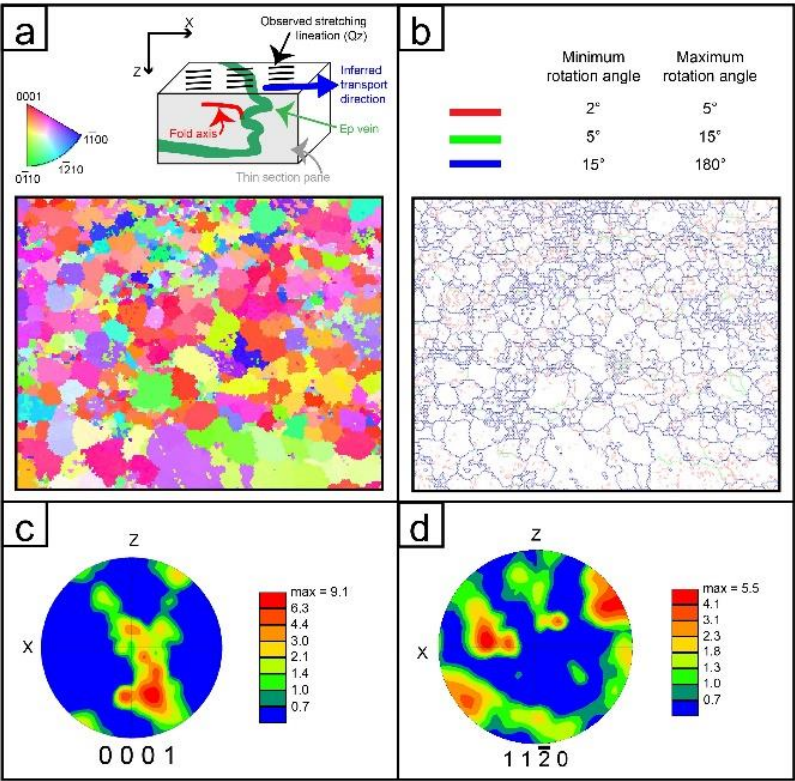
Figure 6: Crystallographic data of quartz in layer 3. (a, top part) The transpressional deformation produces shearing with some lineation (interpreted as transport direction); the related fold axes are oblique (and possibly curved) to the transport direction and cannot be properly described in 3D; the sketch should illustrate the orientation of the presented axes as shown in panels c and d. (a) Orientation of quartz grains in layer 3 of pure quartz area; colors correspond to the inverse pole figure showing on top. (b) Misorientation data of the area of panel a; note the dominant high angle grain boundaries and some minor low angle boundaries as developed after complete recrystallization, which is indicated by the CPO (shown in c and d) (c) Pole figure of quartz <c> axis, indicating a single girdle with relicts of a cross-girdle. (d) Related <a> axes to panel c showing the classical distribution of rhomb and basal glide.
