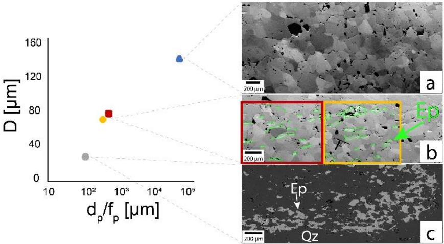
Figure 5: Correlation between quartz grain size ( D ) and Zener parameter (ratio between size and abundance of the second phase, here epidote, p ; d_p/f_p ) of epidote as the second phase determined in the FSE and BSE images of the microstructures in the microfold of layers 2–3. The green lines in the central BSE image contour epidote grains. Ep = epidote; Qz = quartz. Panels a, b and c correspond, respectively, to panels c, a and b of Fig. 4.
