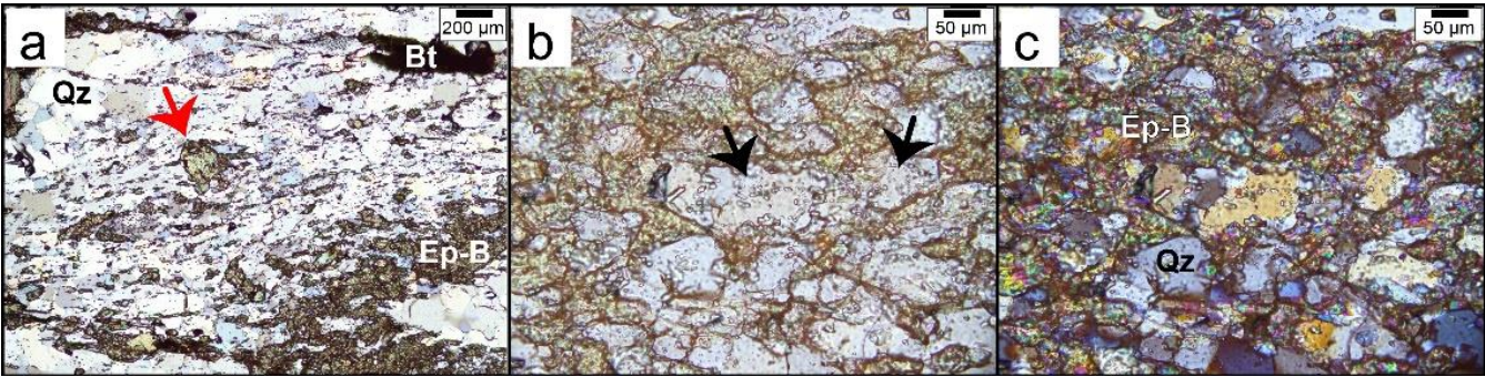
Figure 4: Transmitted light microphotographs of layer 2. (a) Detail of the epidote microfold, with oval epidote grains hosted by dynamically recrystallized quartz and their long axes oriented consistently with the microfold axial planes; red arrow: euhedral epidote grain. Overlapped imaged in plane-polarized and cross-polarized light. (b–c) Details of quartz enclosures among epidote grains in plane-polarized (b) and cross-polarized (c) light; the black arrows point at epidote and fluid inclusions in quartz. Bt = biotite; Ep = epidote; Qz = quartz.
