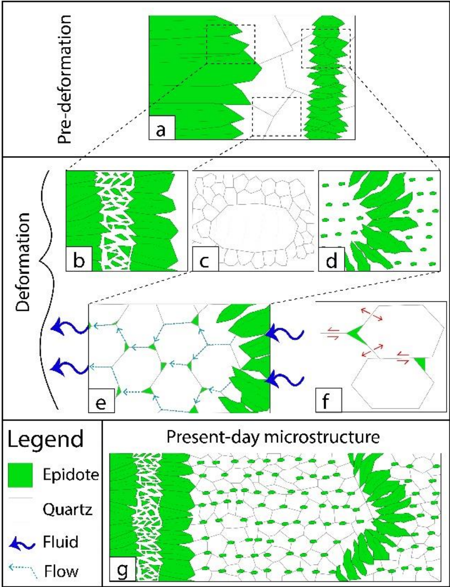
Figure 9: Sketches of the sequence of events affecting the studied epidote vein. (a) Original microstructure formed upon veining. (b) Detail of the fracturing occurring in Epidote-A in layer 1. (c) Dynamic recrystallization of quartz by subgrain rotation. (d) Folding of the epidote band in layer 2 and dissolution–precipitation forming Epidote-B. (e) Detail of the viscous granular flow process, cavitation and formation of nucleation sites (“dynamic granular fluid pump” of Fusses et al., 2009) allowing Epidote-B to precipitate in creep cavities along quartz grain boundaries. (f) Detail of quartz grain boundary sliding allowing dynamic granular fluid pump (modified from Fusses et al., 2009). (g) Present-day microstructure. Not to scale.
