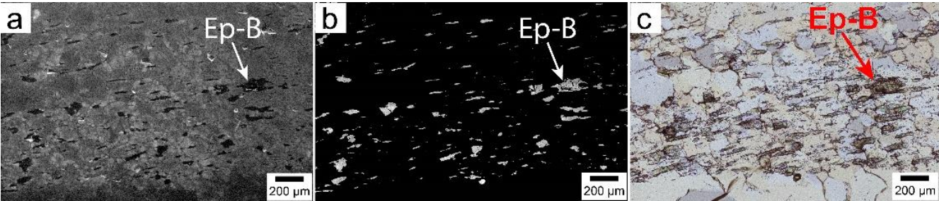
Figure 7: Cathodoluminescence (CL; a) and backscattered electron images (b) of the microstructural domain in the transmitted light microphotograph of panel c. The only minerals in the images are epidote (Ep) and quartz (unlabeled grains). The different CL contrasts in quartz (a) are due to variable trace element contents. The anomalous birefringence in panel c is due to the thickness of the thin section (ca. 60 µm).
