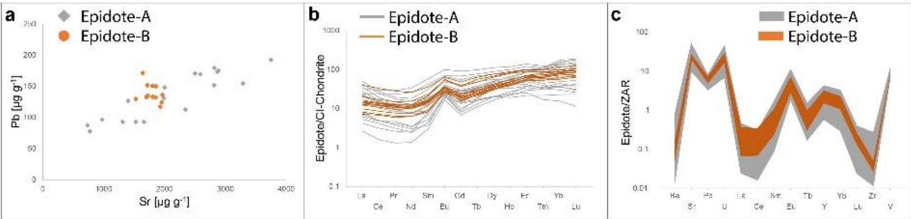
Figure 11: Epidote LA-ICP-MS data of (a) Pb and Sr mass fractions, (b) CI-chondrite normalized (McDonough and Sun, 1995) rare earth element patterns (REE), and (c) mass fractions of selected trace elements in epidote normalized to the Central Aar Granite (ZAR; Schaltegger & Kr henb hl, 1990).
