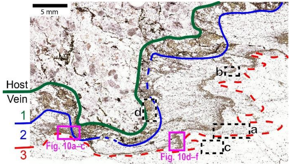
Figure 3: Transmitted-light microscope scan of the studied epidote-quartz (±biotite) vein and the host Central Aar Granite. The numbers 1–3 refer to the vein layers described in Sect. 3. Dashed rectangles a–d indicate the locations of the microstructural domains shown in Fig. 4a–d. The pink rectangles indicates the location of Fig. 10a–c (rotated by 90° clockwise) and Fig. 10d–f (rotated by 180°). Plane-polarized light.
