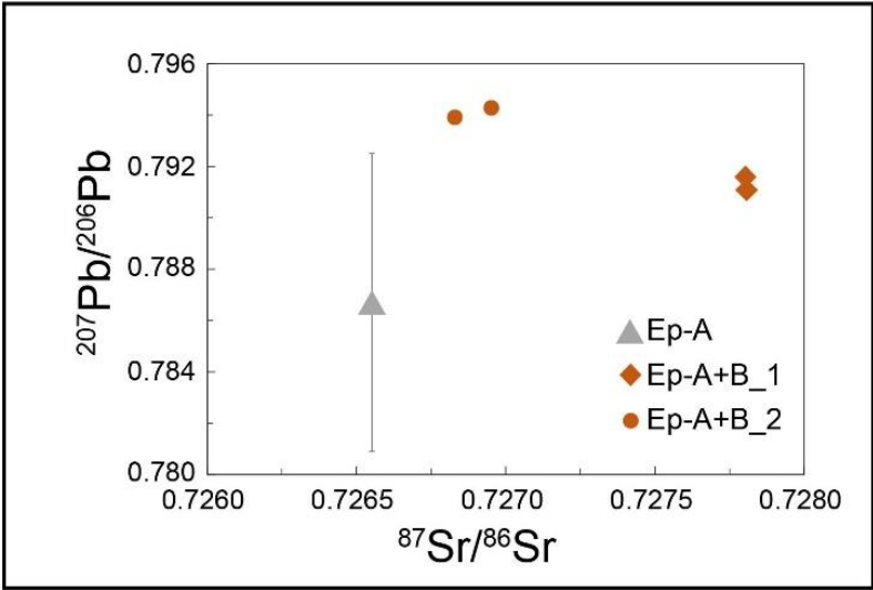
Figure 83: Total ^{207}\text{Pb}/^{206}\text{Pb} and initial ^{87}\text{Sr}/^{86}\text{Sr} data of Epidote-A and epidote micro-separates; the ^{207}\text{Pb}/^{206}\text{Pb} ratio of Epidote-A is by LA-ICP-MS (analysis #10 of Peverelli et al., 2021; their Table 5); all other ^{207}\text{Pb}/^{206}\text{Pb} ratios are by solution ICP-MS; ^{87}\text{Sr}/^{86}\text{Sr} ratios are by TIMS; error bars are smaller than the symbols where not shown.
