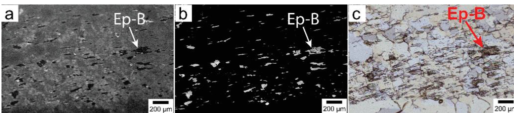
Figure 12: Cathodoluminescence (CL; a) and backscattered electron images (b) of the microstructural domain in the transmitted light microphotograph of panel c. The only minerals in the images are epidote (Ep) and quartz (unlabeled grains). The different CL contrasts in quartz (a) are due to variable trace element contents. The anomalous birefringence in panel c is due to the thickness of the thin section (ca. 60 \mu\text{m} ).
