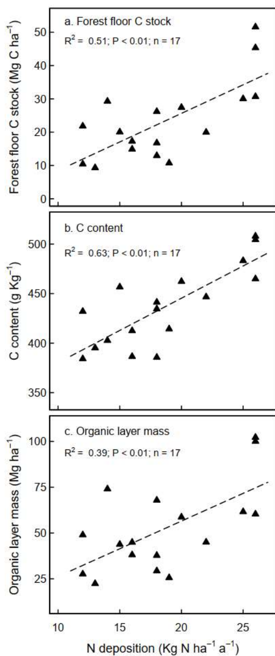
548 Figure A3: : Effects of N deposition on (a) SOC stock (b) C content and (c) dry mass of the L/O r horizon 550 in unlimed coniferous forests. There was no significant correlation evident with broadleaf forests sites.
