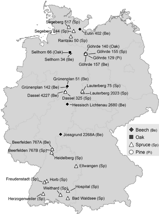
538 Figure A1: Location of the 28 paired liming experiment sites in Germany where soil organic carbon 540 samples were collected.
