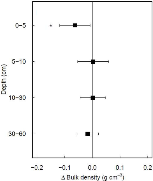
542 Figure A2: Differences in soil bulk density between limed and control plots. Error bars indicate the 95 544 % confidence intervals based on Student's T distribution. Statistical significance was tested using LME models for each respective soil depth / layer at P \leq 0.05 (*) and P \leq 0.01 (**).
