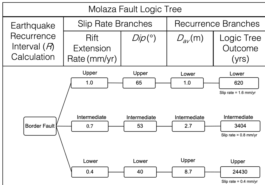
Figure S2. Logic tree outcome for the Molaza Fault.
