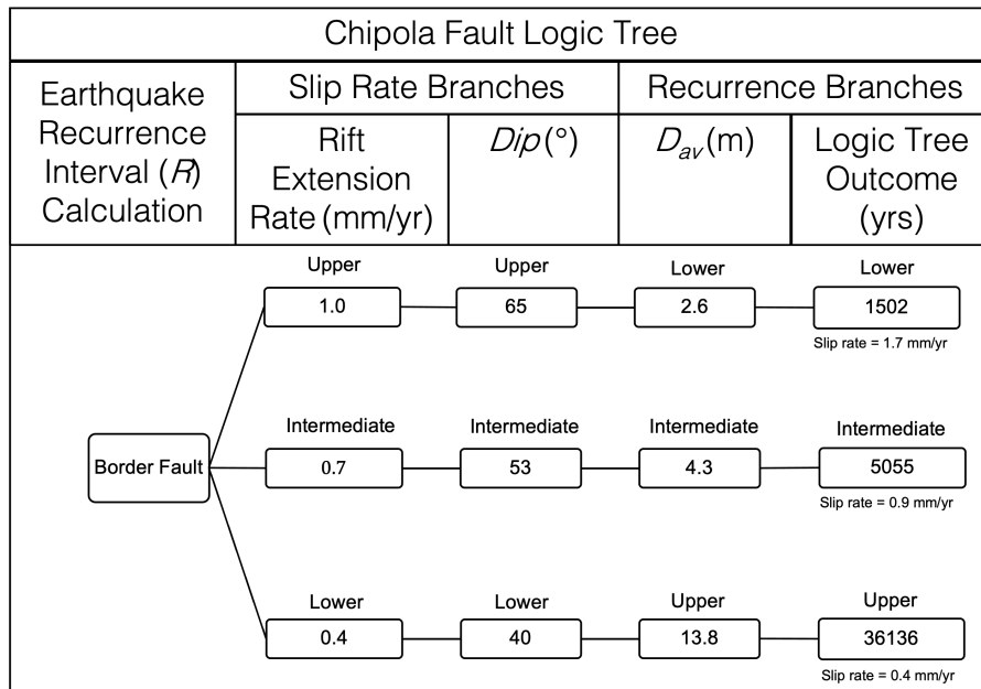
Figure S1. Logic tree outcome for the Chipola Fault.
