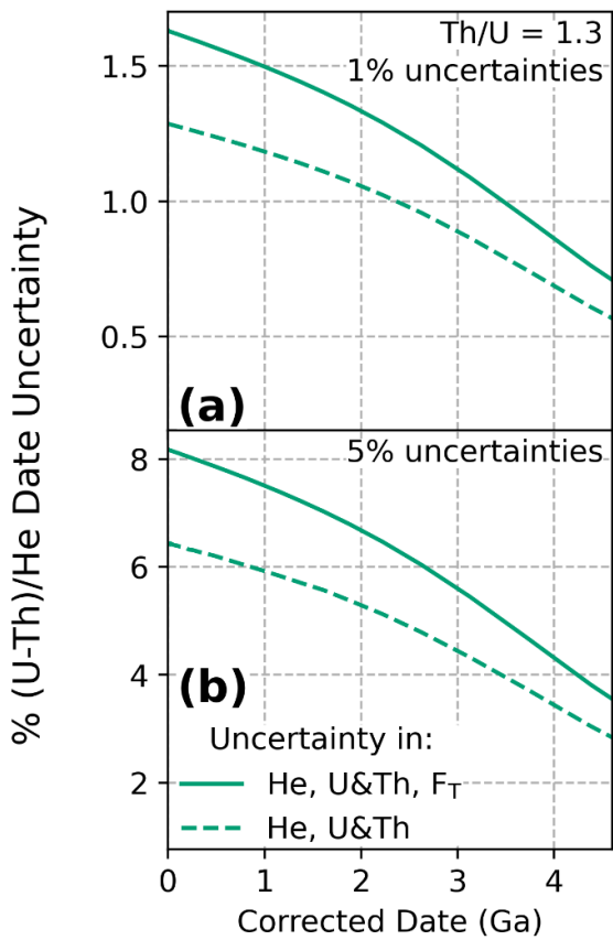
530 Figure C2: Corrected (U-Th)/He date uncertainties for dates of 0 to 4.6 Ga with uncertainty in multiple input parameters. Plots of percent reative uncertainty in the corrected date vs. corrected date for the combination of (a) 1% uncertainty and (b) 5% uncertainty in ^4\text{He} and radionuclides, as well as in all input values. Calculations assume fully correlated uncertainty in isotope-specific F_T values ( r = 1 ) for a Th/U ratio of 1.3 (derived from the Fish Canyon Tuff zircon reference standard).
