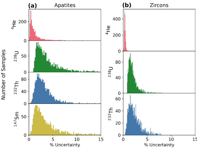
Figure 2: Histograms of percent relative uncertainty in ^4\text{He} , ^{238}\text{U} , ^{232}\text{Th} , and ^{147}\text{Sm} absolute amounts for (a) apatite (N = 1,978) and (b) zircon (N = 1,753). Note that the y-axis scales differ for these plots.
