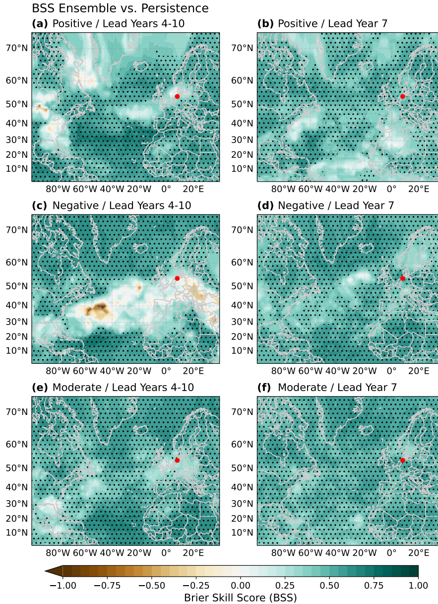
Figure 6. Prediction skill of probabilistic forecasts of positive (a,b) , negative (c,d) , and moderate (e,f) winter mean (DJF) MSLP anomalies, expressed as the Brier Skill Score ( BSS ) of the 64 member ensemble evaluated against a persistence prediction as a baseline for lead years 4-10 (a,c,e) and lead year 7 (b,d,f) . Thresholds for event detection are set to -1 and 1. The German Bight is marked by a red dot. Stippling marks areas with a BSS significantly different from 0 ( p \leq 0.05 ).
