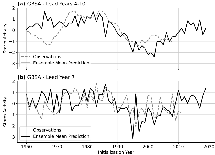
Figure A1. Exemplary time series of ensemble mean predictions (black, solid) and corresponding observations (grey, dashed) of German Bight storm activity (GBSA) for lead years 4-10 (a) and lead year 7 (b) .
