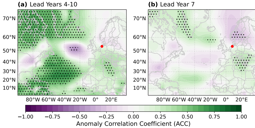
Figure 4. Gridpoint-wise anomaly correlation coefficient ( ACC ) between the deterministic hindcast ensemble mean prediction of winter mean (DJF) MSLP anomalies and ERA5 reanalysis data for lead years 4-10 (a) and lead year 7 (b) . The German Bight is marked by a red dot. Anomalies are calculated for each member individually and averaged over the entire ensemble afterwards. Stippling indicates significant correlations ( p \leq 0.05 ).
