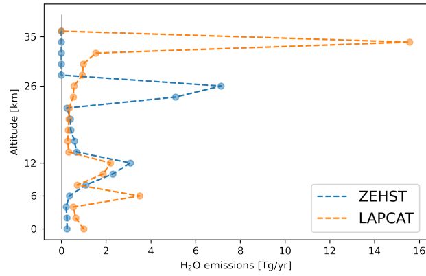
Figure A1. Vertical distribution of annual H_2O - H_2O emission for ZEHST and LAPCAT. The peak at 6 km altitude comes from hypersonic boost of the LAPCAT aircraft. The vertical distribution was aggregated for a better comparability (with a 2 km bin size). For the total amount of emission, see Tab. Table 2 .
