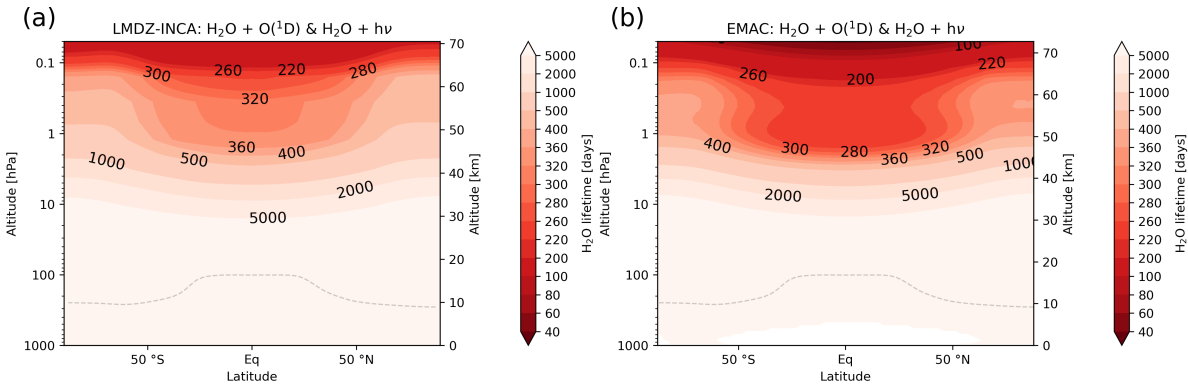
Figure 6. Zonal mean (photo-)chemical H_2O -H 2 O lifetime in days dependent on photolysis and reaction with O(^1D) -O( 1 D) for LMDZ-INCA (a) and EMAC (b). Figure A5, showing both reactions independently, can be found in the appendix.
