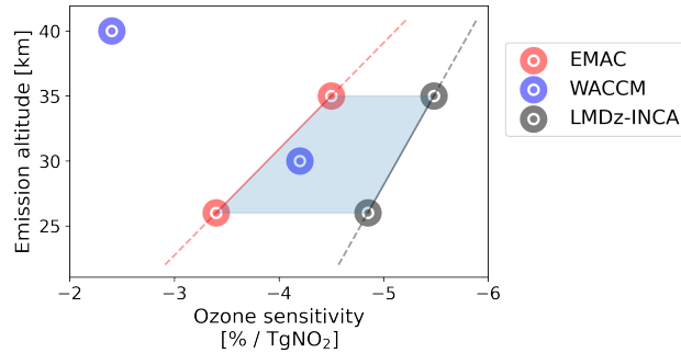
Figure 10. Ozone sensitivity from three different models WACCM, EMAC and LMDZ-INCA dependent on altitude. Results from this work were calculated using values from Tab. Table 2 and Tab. Table 4 . Results for WACCM were published by Kinnison et al. (2020, Tab. 2) Kinnison et al. (2020, Table 2) . The shaded area highlights the good agreement of LMDZ-INCA and EMAC results with WACCM results for the region from approximately 26-35 km altitude.
