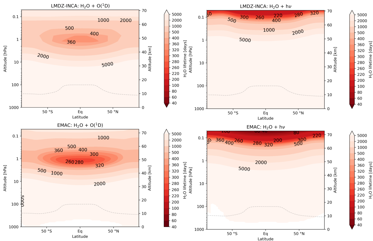
Figure A5. Zonal mean (photo-)chemical H_2O - H_2O lifetime in days for photolysis (right column) and reaction with O(^1D) - O(^1D) (left column) for LMDZ-INCA (upper row) and EMAC (lower row).
