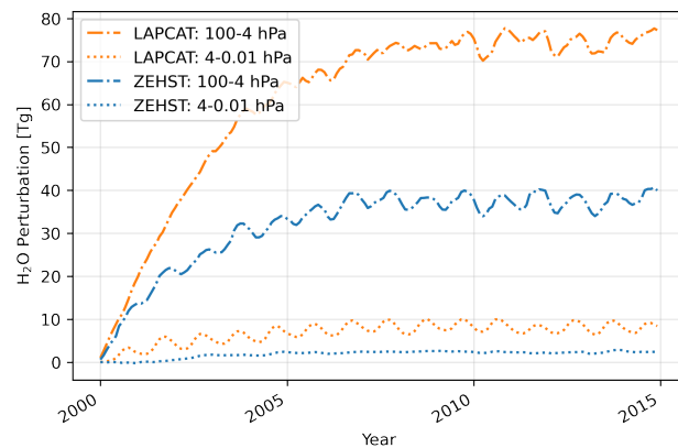
Figure A2. Timeline plot of accumulated trace gas H_2O - H_2O in teragram, based on monthly mean values. Blue lines represent scenario ZEHST and orange lines represent scenario LAPCAT. Shown is the H_2O - H_2O perturbation over time above 4 hPa (dotted) and from 4-100 hPa (solid-dotted).
