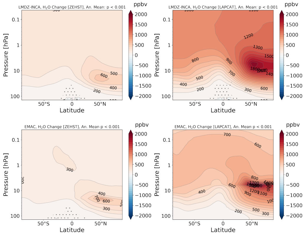
Figure 5. Multi-annual mean (2010-2014) of H_2O -H 2 O perturbations (ppbv) for the ZEHST scenario (left) and the LAPCAT scenario (right) for both models LMDZ-INCA (upper) and EMAC (lower) after approximately thirteen years of continuous emission. Cruise altitudes are approximately at the respective perturbation maxima. The dotted region corresponds to the grid points where the mean perturbations are not significant at a 99.9 % level.
