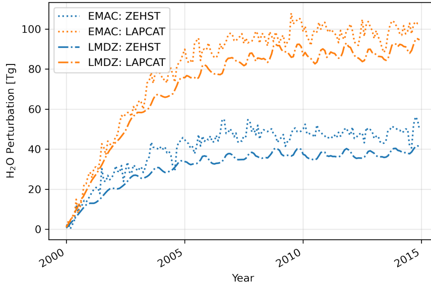
Figure 3. Temporal evolution of mass perturbation of H_2O - H_2O in Tg above the tropopause. Blue and orange lines represent scenario ZEHST and LAPCAT, respectively. The annual amount of emitted trace gases is listed in Tab. Table 2 .
