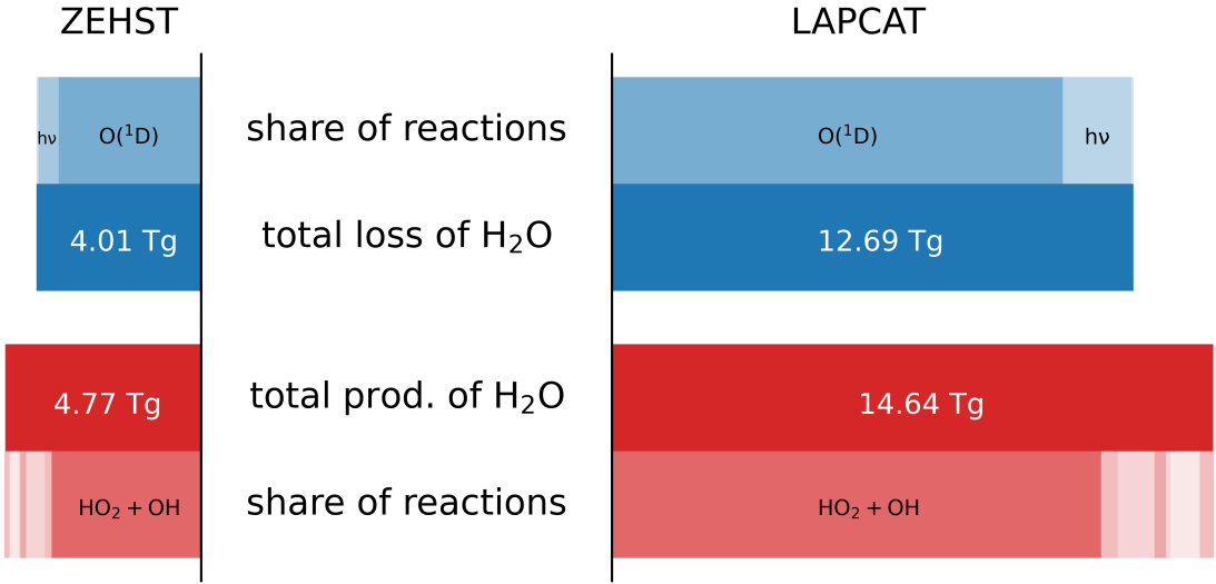
Figure 7. Bar plot of annual chemical loss and production perturbation of H_2O at stratospheric altitudes (100-0.1 hPa) for the ZEHST (left) and the LAPCAT (right) scenarios due to emitted trace gases (scenario-reference). This diagnosis includes a total of five H_2O destroying and 45 H_2O producing chemical reactions. The most relevant reactions of loss and production are shown as bright red and blue bars. Additionally, all dominant reactions of production are presented in detail in Fig. 8.
