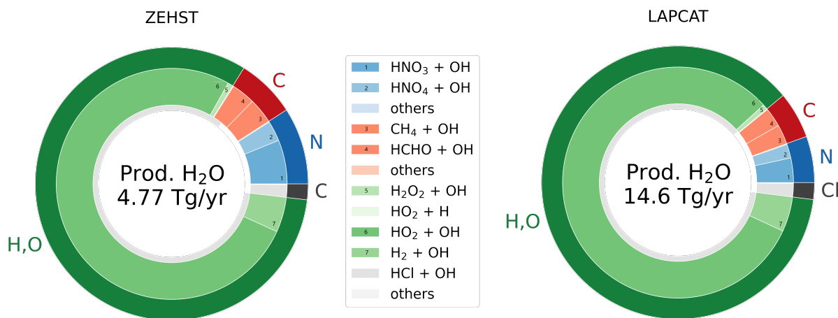
Figure 8. Pie plots on chemical reactions responsible for \text{H}_2\text{O} production derived from the EMAC simulation results (scenario-reference). Left: ZEHST scenario. Right: LAPCAT scenario. The darker outer ring shows the molecular category the reactions belong to (carbon-, nitrogen-, chlorine- or hydrogen-based). The total sum of \text{H}_2\text{O} production is written in the center. The colored inner ring shows the proportion of different reactions within each category. We added black numbers in the legend and the bright inner ring to represent the relation in addition to colours.
