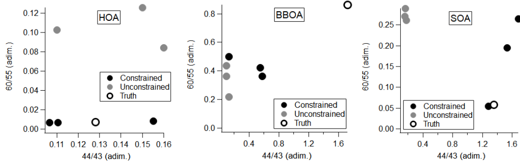
Figure R3.1. Scatterplots of m/z60-to-m/z55 ratio vs. m/z44-to-m/z43 ratio for the three basic factors in the synthetic dataset for each season.
