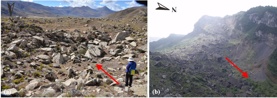
65 Figure 1: Giant blocks and their orientations (the red arrow indicates the motion direction of the rock avalanches): (a) Nixu rock avalanche in Tibet plateau, China (the base photo was provided from professor Yufeng Wang and Qiangong Cheng (Wang et al., 2021)); (b) Jiweishan rock avalanche in Chongqing, China (the base photo was provided from professor Ming Zhang (Zhang et al., 2019)).
