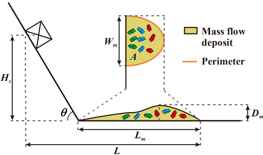
Figure 5: Diagram of experimental rock avalanches: L_m = Maximum length of the deposit; W_m = maximum width of the deposit; D_m = maximum depth of the deposit; A = area of the deposit projected on the horizontal plane; P =
