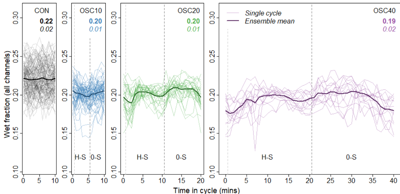
Figure 7. Wet fraction ( across the whole fan , measured from all channels), versus time in the sediment supply oscillation cycle. The thin lines represent each individual supply oscillation cycle; the thick line is the ensemble mean. H-S denotes the high-supply period; O-S denotes zero-supply. Coloured text indicates each experiment's time-averaged mean and standard deviation.
