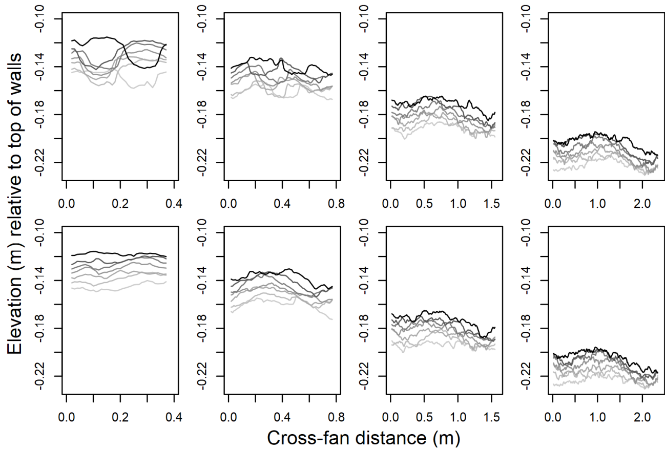
Figure A7. Fan elevation at arcuate cross-fan profiles in Run 9OSC40 , located 0.25, 0.5, 1.0 and 1.5 m downfan (left to right). Upper panel: examples of fan topography at the end of zero-supply periods. Lower panel: examples of fan topography at the end of high-supply periods. Example data are from time steps 80 minutes apart; darker colours denote later time steps.
