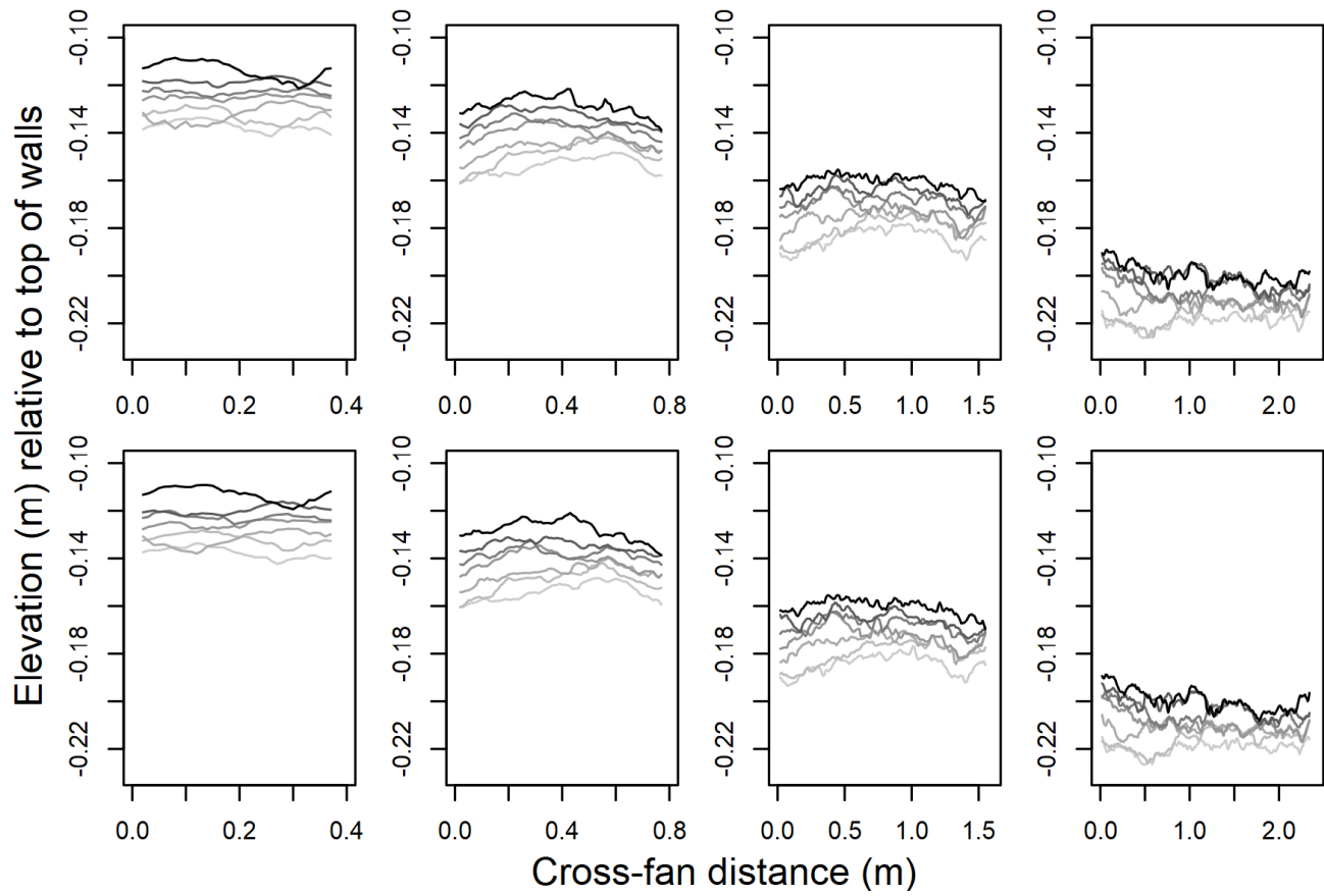
Figure A5. Fan elevation at arcuate cross-fan profiles in Run 7OSC10 , located 0.25, 0.5, 1.0 and 1.5 m downfan (left to right). Upper panel: examples of fan topography at the end of zero-supply periods. Lower panel: examples of fan topography at the end of high-supply periods. Example data are from time steps 80 minutes apart; darker colours denote later time steps.
