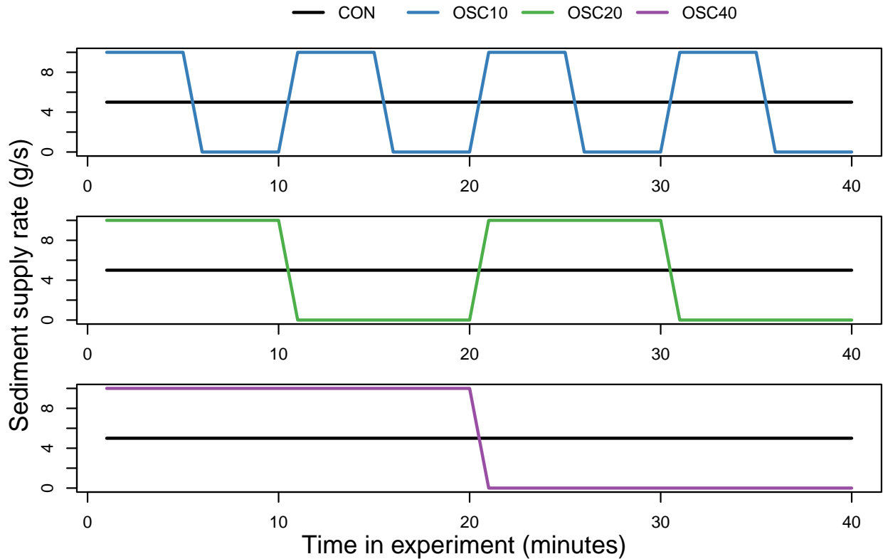
Figure 2. The durations of high-supply and zero-supply periods in Runs CON and 7-9 OSC10-OSC40 . The constant sediment supply rate in Run CON equals the mean supply rate in all other runs.
