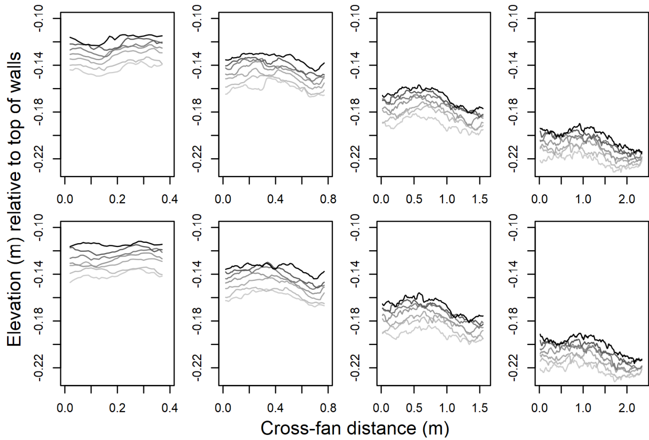
Figure A6. Fan elevation at arcuate cross-fan profiles in Run 8QSC20 , located 0.25, 0.5, 1.0 and 1.5 m downfan (left to right). Upper panel: examples of fan topography at the end of zero-supply periods. Lower panel: examples of fan topography at the end of high-supply periods. Example data are from time steps 80 minutes apart; darker colours denote later time steps.
