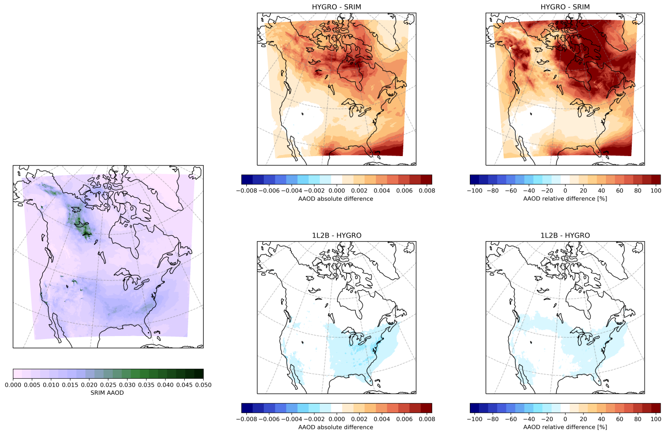
Figure 7. left: mean AAOD from the SRIM simulation; top centre: mean difference in AAOD between the HYGRO and SRIM simulations; top right: relative difference in mean AAOD between the HYGRO and SRIM simulations; bottom centre: mean difference in AAOD between the 1L2B and HYGRO simulations; bottom right: relative difference in mean AAOD between the 1L2B and HYGRO simulations. Only results from the hours of 1300-2100 UTC are included as the AOD is only calculated during local daylight hours.
