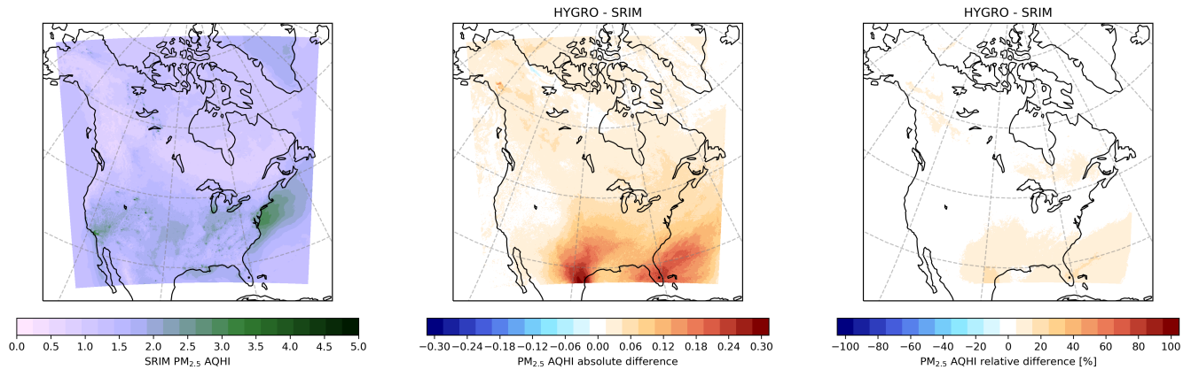
Figure 3. left: mean PM_{2.5} AQHI values from the SRIM simulation; centre: mean difference in PM_{2.5} AQHI values between the HYGRO and SRIM simulations; right: relative difference in mean PM_{2.5} AQHI values between the HYGRO and SRIM simulations. Note that PM_{2.5} AQHI values are nearly identical in the HYGRO and 1L2B simulations.
