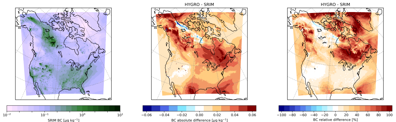
Figure 4. left: mean surface BC mixing ratios from the SRIM simulation; centre: mean difference in BC mixing ratios between the HYGRO and SRIM simulations; right: relative difference in mean BC mixing ratios between the HYGRO and SRIM simulations.
