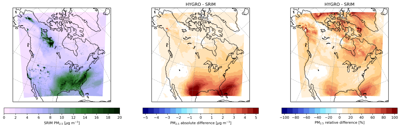
Figure 1. left: mean PM 2.5 concentrations from the SRIM simulation; centre: mean difference in PM 2.5 concentrations between the HYGRO and SRIM simulations; right: relative difference in mean PM 2.5 concentrations between the HYGRO and SRIM simulations.
