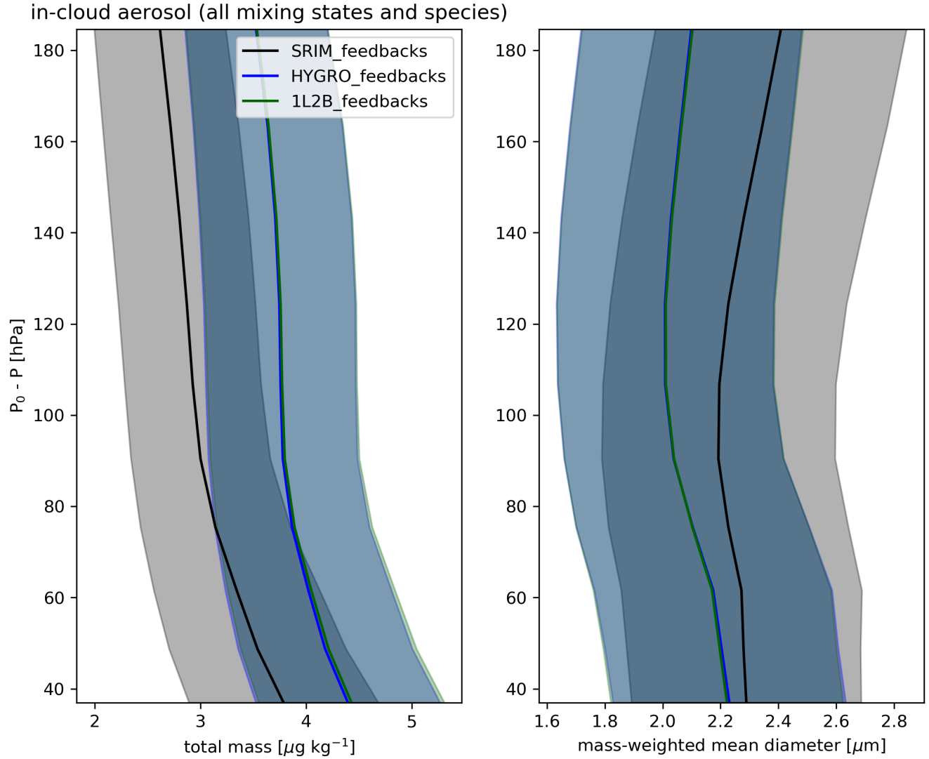
Figure 9. Vertical distribution of temporally and horizontally averaged aerosol properties in cloudy grid cells in the SRIM_feedbacks, HYGRO_feedbacks, and 1L2B_feedbacks simulations. Left: total mass mixing ratios. Right: mass-mean aerosol diameter. The shading indicates one temporal standard deviation about the mean.
