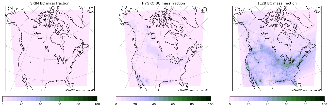
Figure 5. Black carbon mass fractions in BC-containing particles. Values are given at the surface, and weighted by the BC mass in each size bin and mixing-state category. Values are shown for the following simulations: left: SRIM; centre: HYGRO; right: 1L2B.
