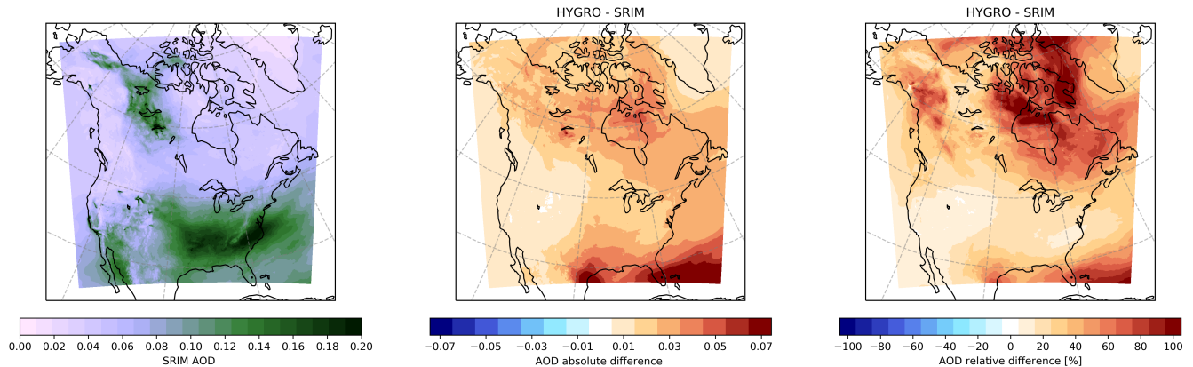
Figure 6. left: mean AOD from the SRIM simulation; centre: mean difference in AOD between the HYGRO and SRIM simulations; right: relative difference in mean AOD between the HYGRO and SRIM simulations. Only results from the hours of 1300-2100 UTC are included as the AOD is only calculated during local daylight hours.
