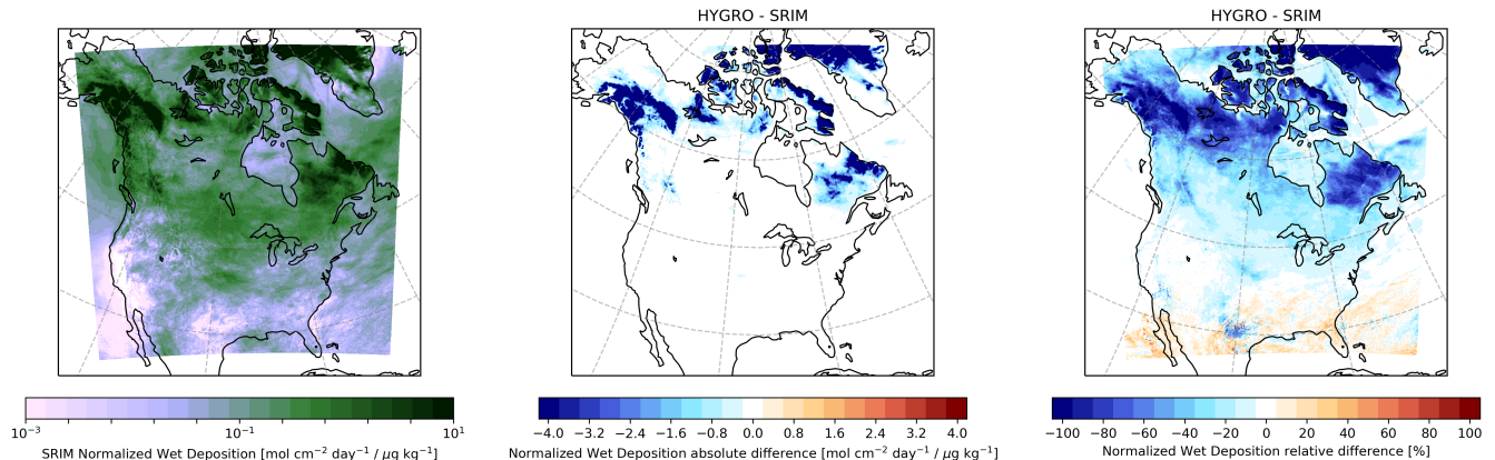
Figure 2. left: temporal means of wet deposition fluxes normalized by surface total aerosol concentrations from the SRIM simulation; centre: mean difference in normalized wet deposition fluxes between the HYGRO and SRIM simulations; right: relative difference in mean normalized wet deposition fluxes between the HYGRO and SRIM simulations.
