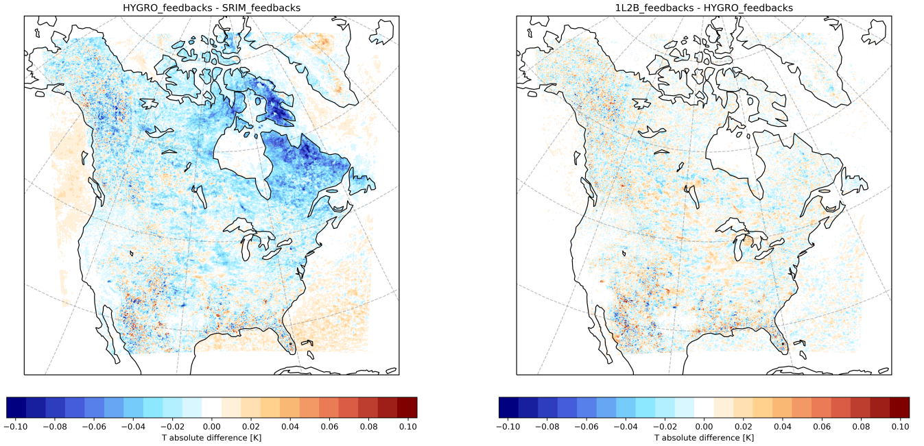
Figure 11. Left: mean difference in surface temperature between the HYGRO_feedbacks and SRIM_feedbacks simulations; right: mean difference in surface temperature between the 1L2B_feedbacks and HYGRO_feedbacks simulations.
