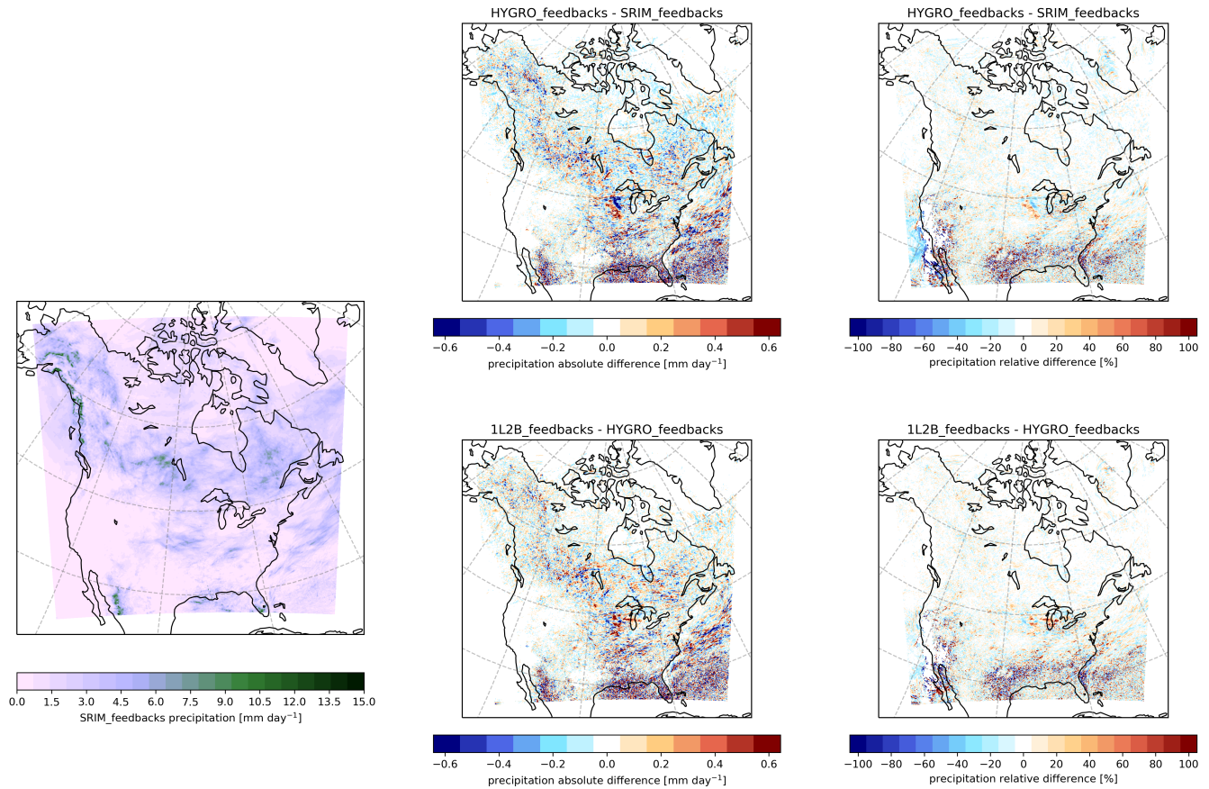
Figure 10. Left: mean precipitation from the SRIM_feedbacks simulation; top centre: mean difference in precipitation between the HYGRO_feedbacks and SRIM_feedbacks simulations; top right: relative difference in mean precipitation between the HYGRO_feedbacks and SRIM_feedbacks simulations; bottom centre: mean difference in precipitation between the 1L2B_feedbacks and HYGRO_feedbacks simulations; bottom right: relative difference in mean precipitation between the 1L2B_feedbacks and HYGRO_feedbacks simulations.
